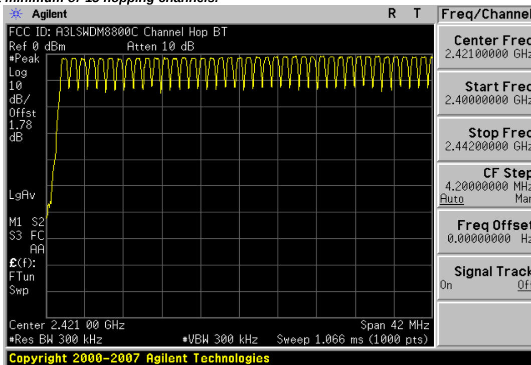
Plot 6-10. Low End Spectrum Channel Hopping Plot (Bluetooth)
