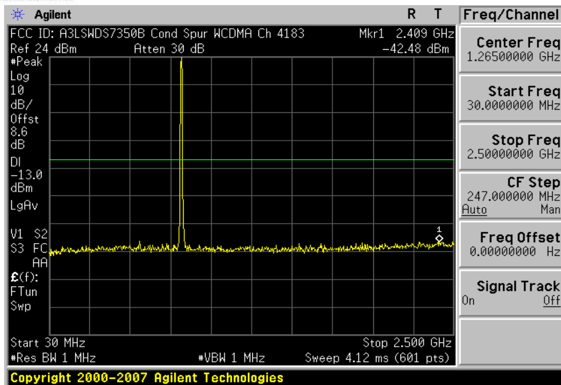
Plot 7-27. Conducted Spurious Plot (Cellular WCDMA Mode – Ch. 4183)
