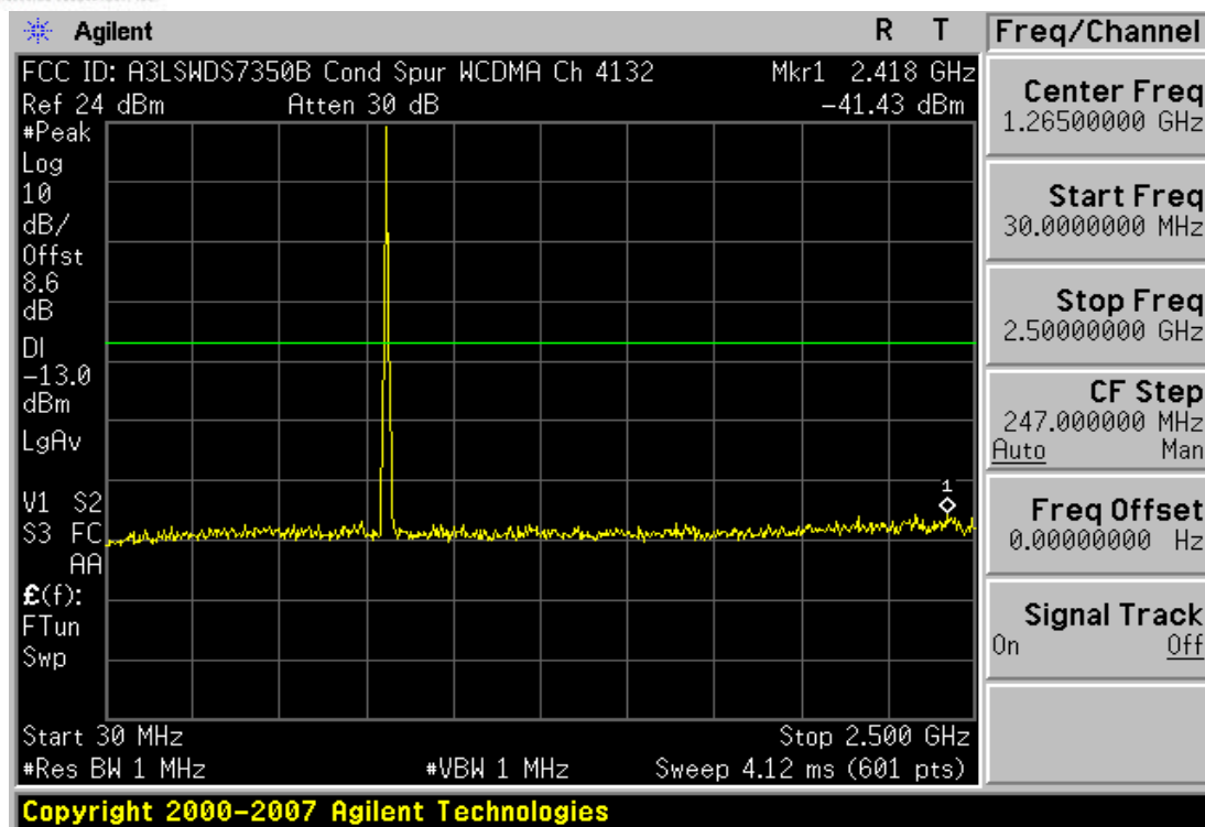
Plot 7-23. Conducted Spurious Plot (Cellular WCDMA Mode - Ch. 4132)
