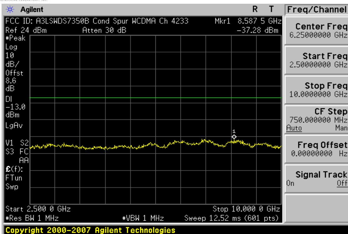
Plot 7-31. Conducted Spurious Plot (Cellular WCDMA Mode – Ch. 4233)
