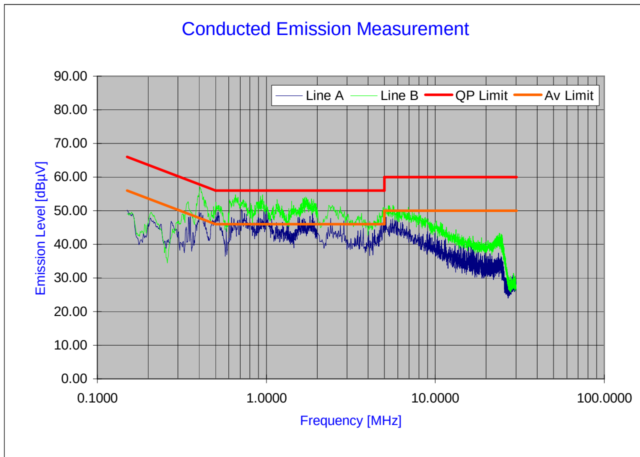
Plot 6-24. Line Conducted Plot with 802.11g
