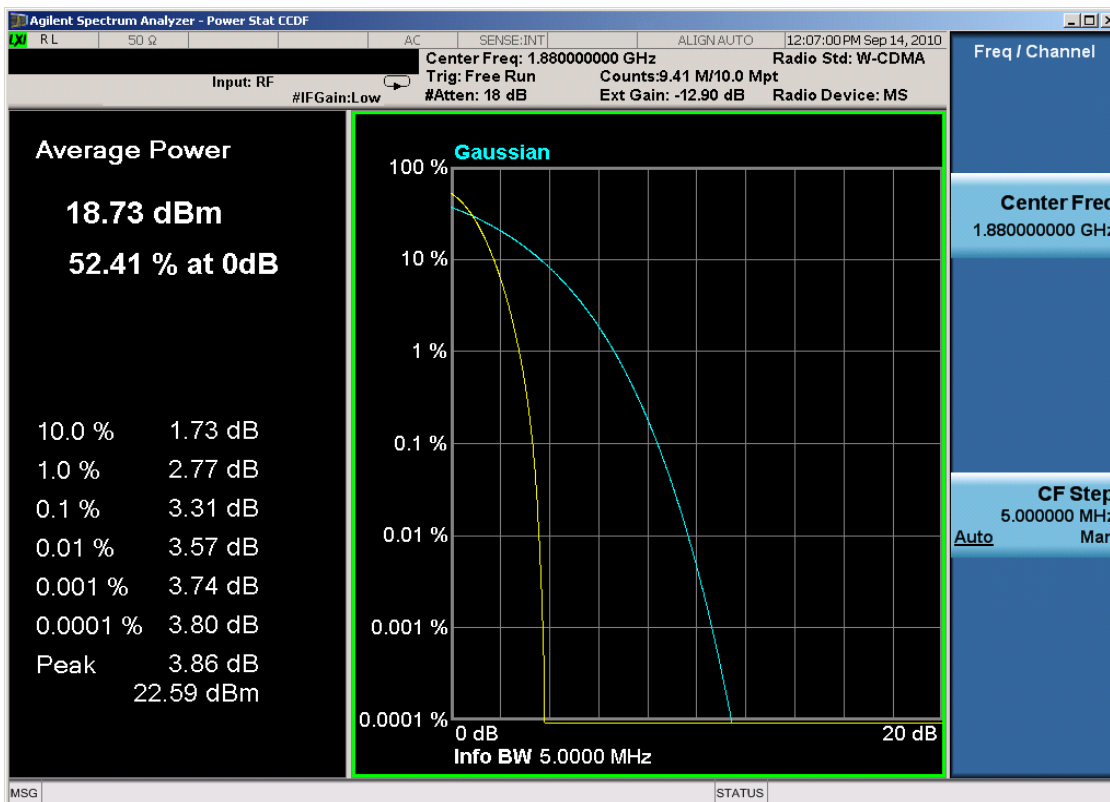
Plot 7-30. Peak-Average Ratio Plot (PCS WCDMA Mode – Ch. 9400)
