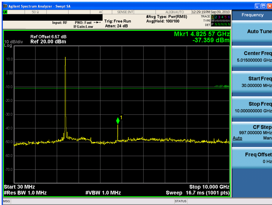
Plot 6-41. Conducted Spurious Plot (802.11b – Ch. 1)
