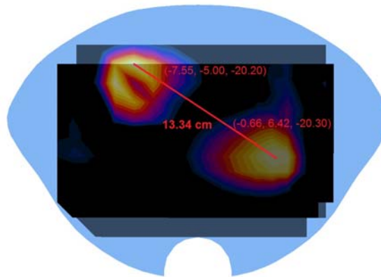
Figure 11-1 Peak SAR Location Plot of GPRS 1900 and 2.4 GHz WLAN for Back Side (at 0.0 cm)
