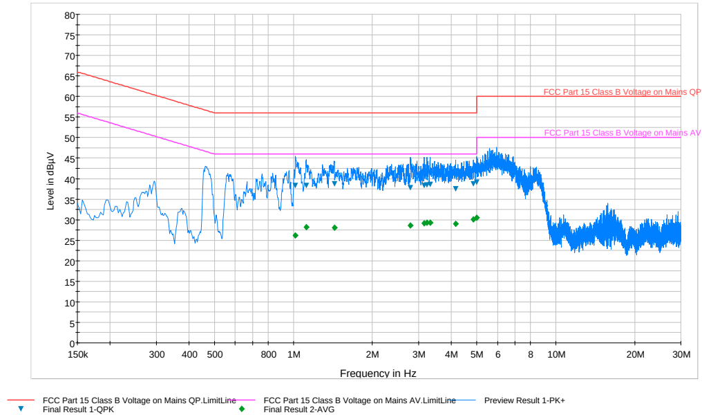
Plot 6-60. Line Conducted Plot with 802.11a UNII Band 3 (N)
