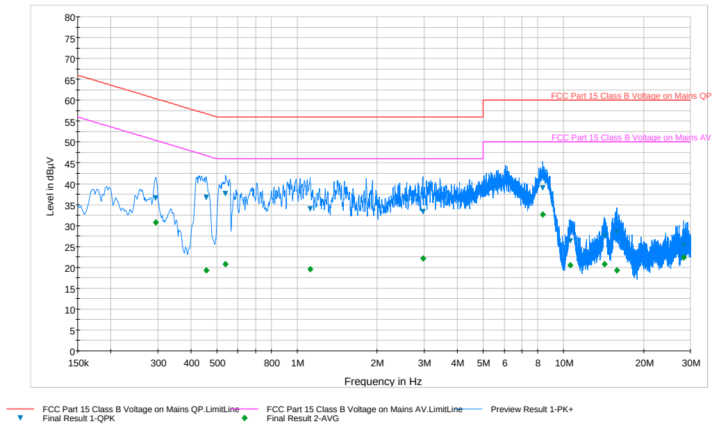
Plot 6-55. Line Conducted Plot with 802.11a UNII Band 1 (L1)
