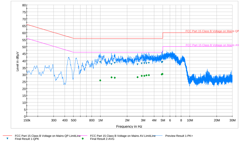
Plot 6-56. Line Conducted Plot with 802.11a UNII Band 1 (N)
