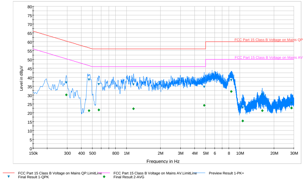
Plot 6-57. Line Conducted Plot with 802.11a UNII Band 2 (L1)
