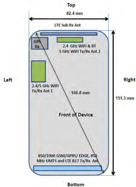
Figure 1-1 DUT Antenna Locations
