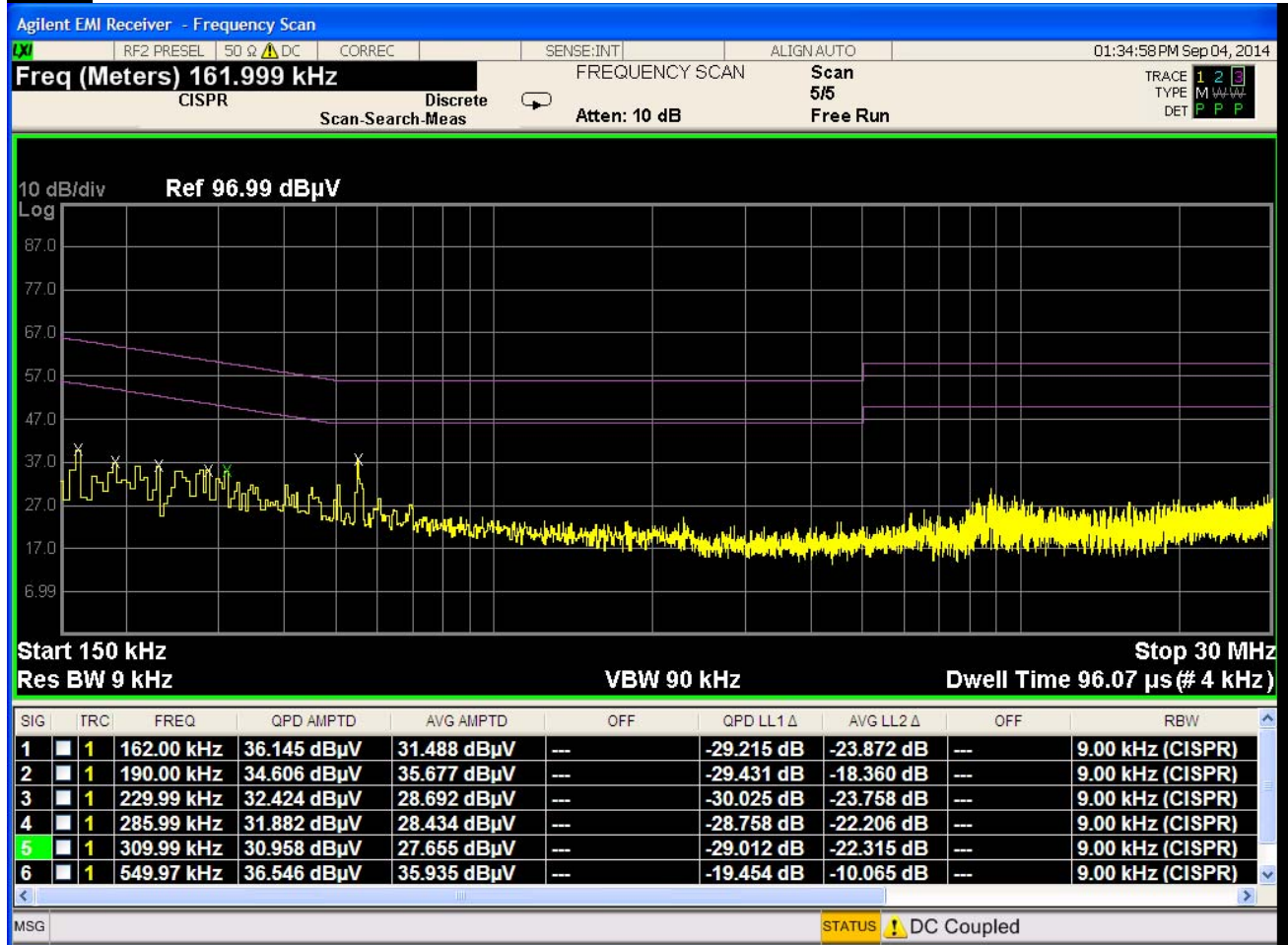
Plot 6-45. Line-Conducted Test Plot (N)
