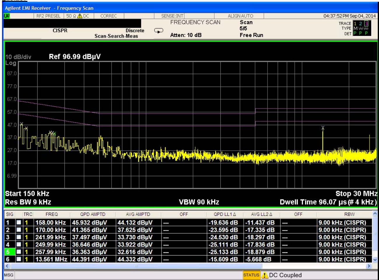
Plot 8-1. Line-Conducted Test Plot (L1)
