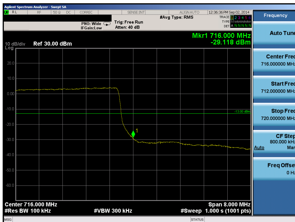
Plot 6-22. Upper Band Edge Plot (Band 17 – 10.0MHz QPSK – RB Size 50)
