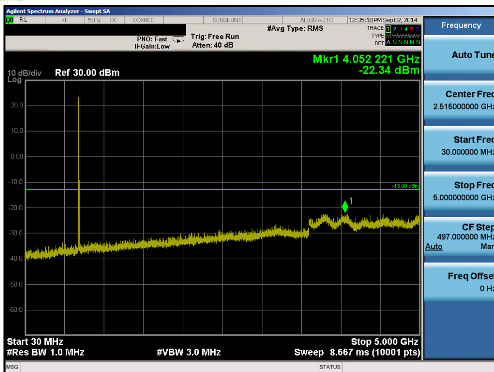
Plot 6-15. Conducted Spurious Plot (Band 17 – 10.0MHz QPSK – RB Size 1, RB Offset 0 – High Channel)
