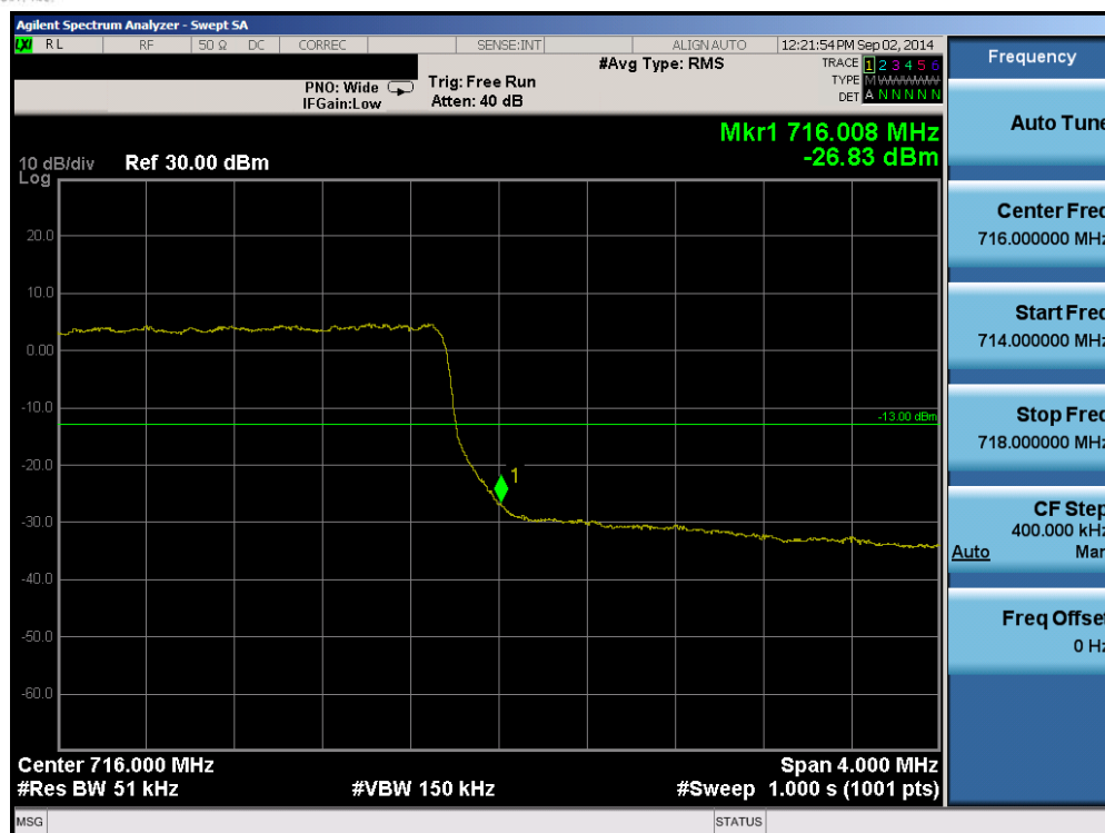
Plot 6-19. Upper Band Edge Plot (Band 17 – 5.0MHz QPSK – RB Size 25)
