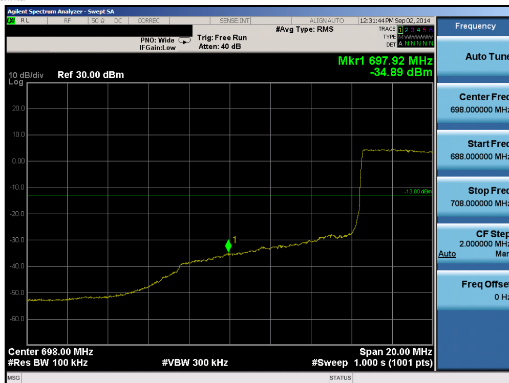
Plot 6-21. Lower Band Edge Plot (Band 17 – 10.0MHz QPSK – RB Size 50)
