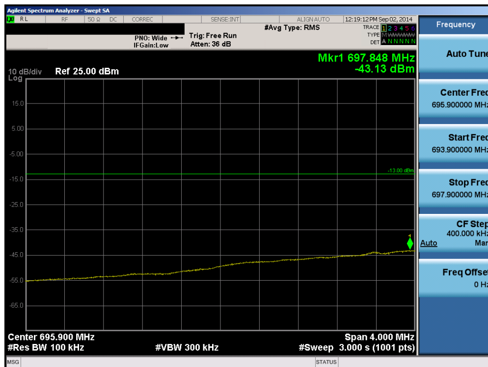
Plot 6-18. Lower Extended Band Edge Plot (Band 17 – 5.0MHz QPSK – RB Size 25)
