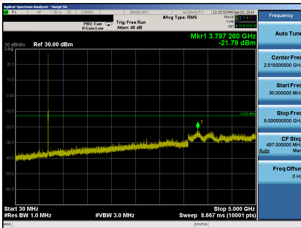
Plot 6-7. Conducted Spurious Plot (Band 17 – 5.0MHz QPSK – RB Size 1, RB Offset 0 – Mid Channel)
