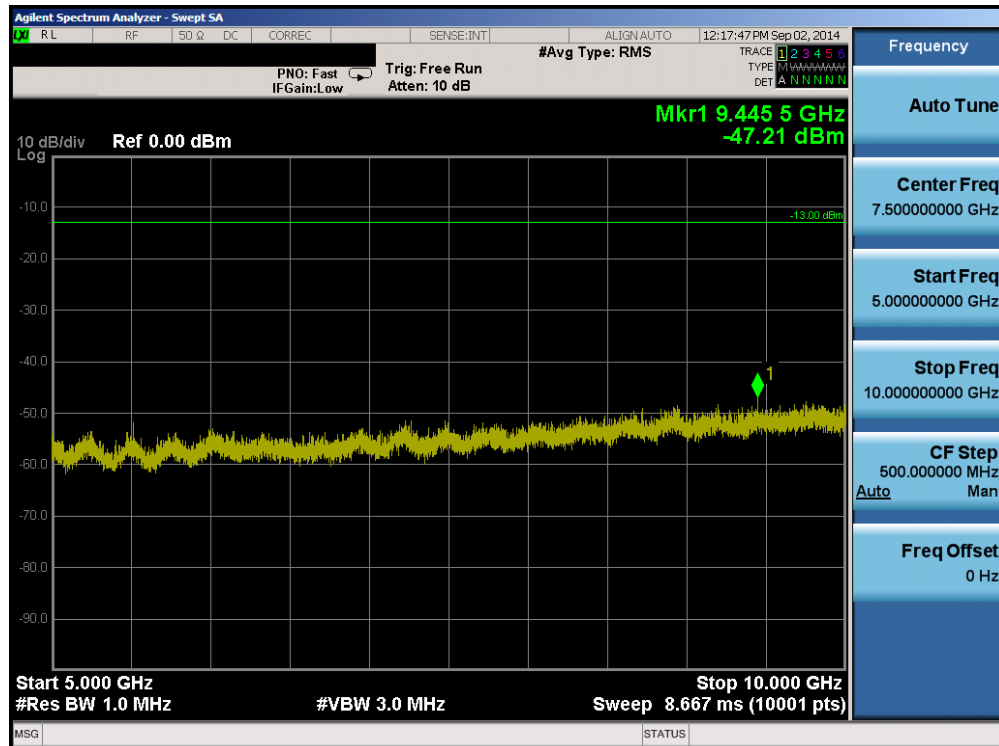
Plot 6-6. Conducted Spurious Plot (Band 17 – 5.0MHz QPSK – RB Size 1, RB Offset 0 – Low Channel)
