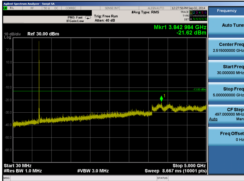
Plot 6-11. Conducted Spurious Plot (Band 17 – 10.0MHz QPSK – RB Size 1, RB Offset 0– Low Channel)
