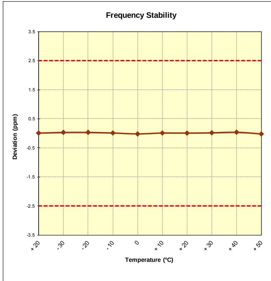
Figure 6-6. Frequency Stability Graph (Band 17)
