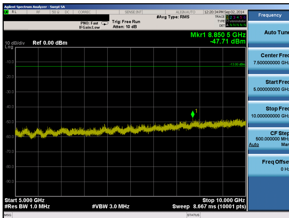
Plot 6-10. Conducted Spurious Plot (Band 17 – 5.0MHz QPSK – RB Size 1, RB Offset 0 – High Channel)
