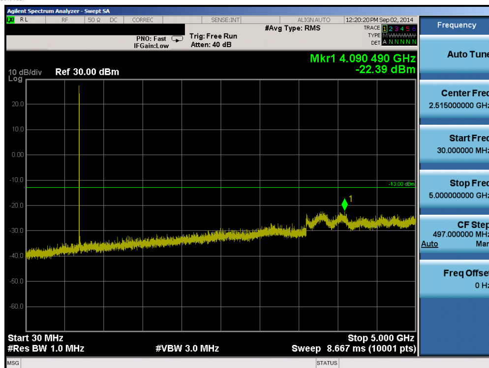
Plot 6-9. Conducted Spurious Plot (Band 17 – 5.0MHz QPSK – RB Size 1, RB Offset 0 – High Channel)
