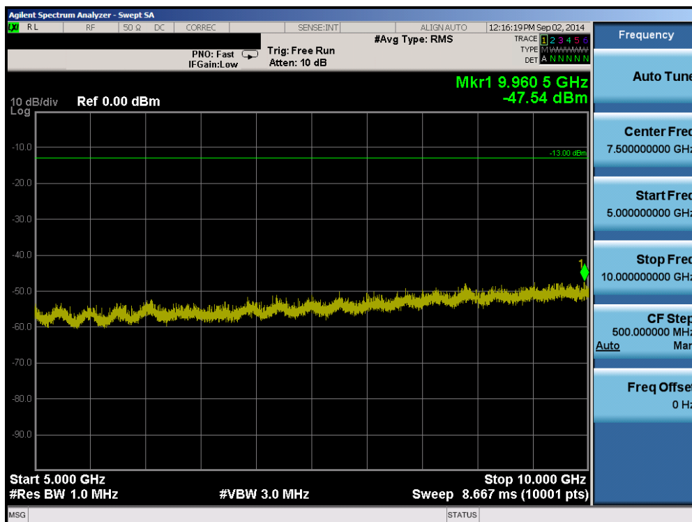
Plot 6-8. Conducted Spurious Plot (Band 17 – 5.0MHz QPSK – RB Size 1, RB Offset 0 – Mid Channel)
