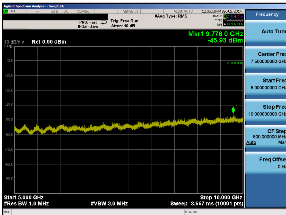
Plot 6-16. Conducted Spurious Plot (Band 17 – 10.0MHz QPSK – RB Size 1, RB Offset 0 – High Channel)
