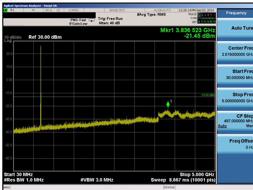
Plot 6-13. Conducted Spurious Plot (Band 17 – 10.0MHz QPSK – RB Size 1, RB Offset 0 – Mid Channel)
