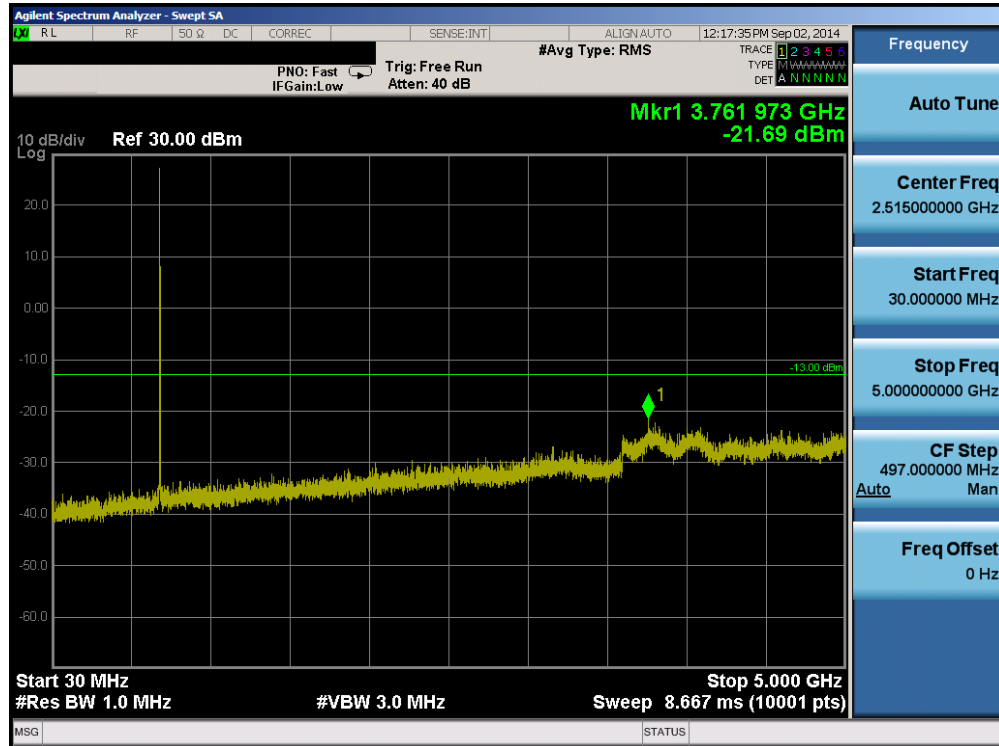
Plot 6-5. Conducted Spurious Plot (Band 17 – 5.0MHz QPSK – RB Size 1, RB Offset 0 – Low Channel)
