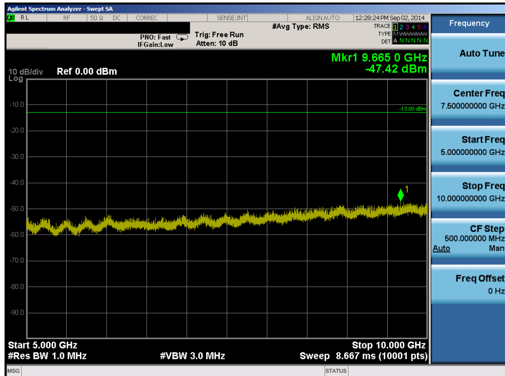
Plot 6-12. Conducted Spurious Plot (Band 17 – 10.0MHz QPSK – RB Size 1, RB Offset 0 – Low Channel)
