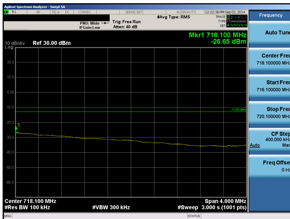
Plot 6-20. Upper Extended Band Edge Plot (Band 17 – 5.0MHz QPSK – RB Size 25)
