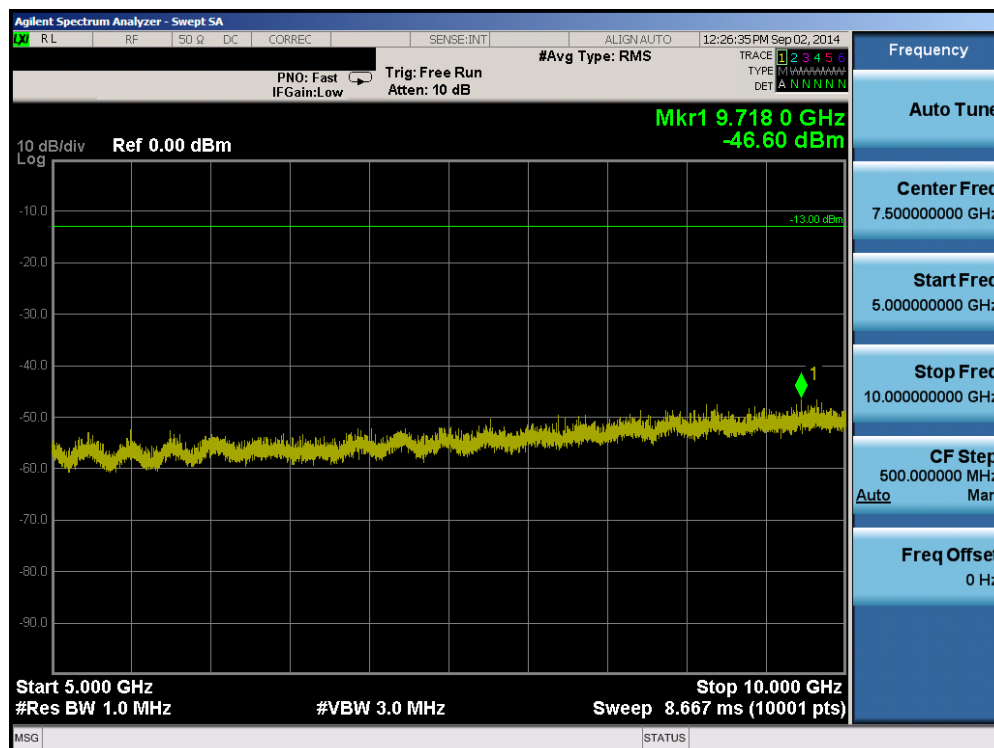
Plot 6-14. Conducted Spurious Plot (Band 17 – 10.0MHz QPSK – RB Size 1, RB Offset 0 – Mid Channel)
