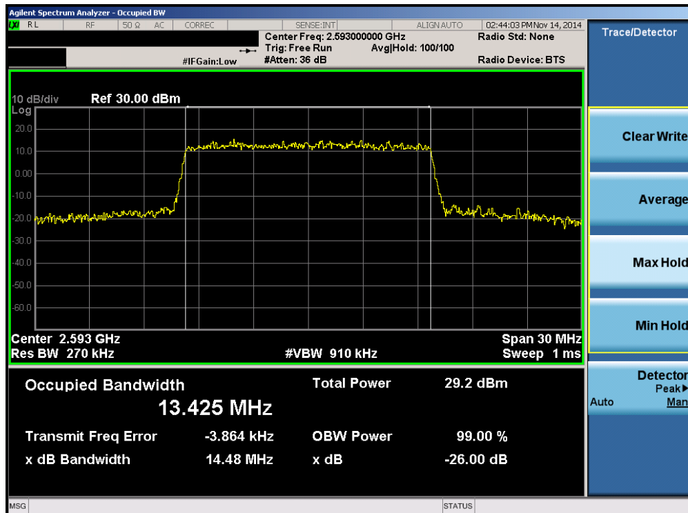
Plot 6-6. Occupied Bandwidth Plot (Band 41 – 15.0MHz 16-QAM – RB Size 75)
