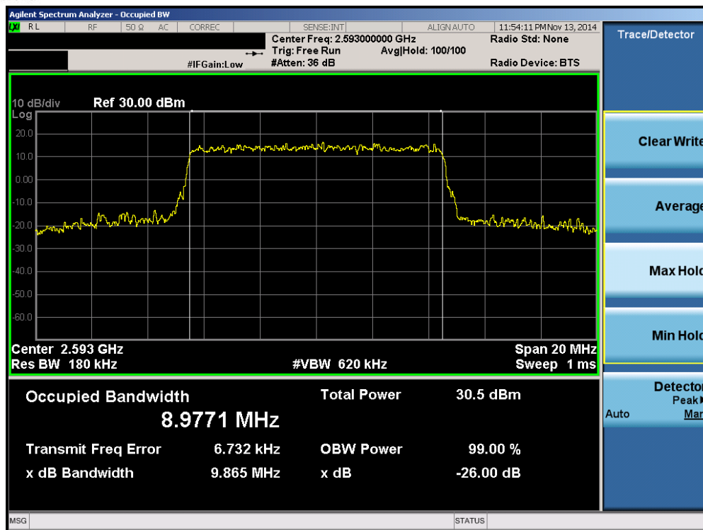
Plot 6-3. Occupied Bandwidth Plot (Band 41 – 10.0MHz QPSK – RB Size 50)
