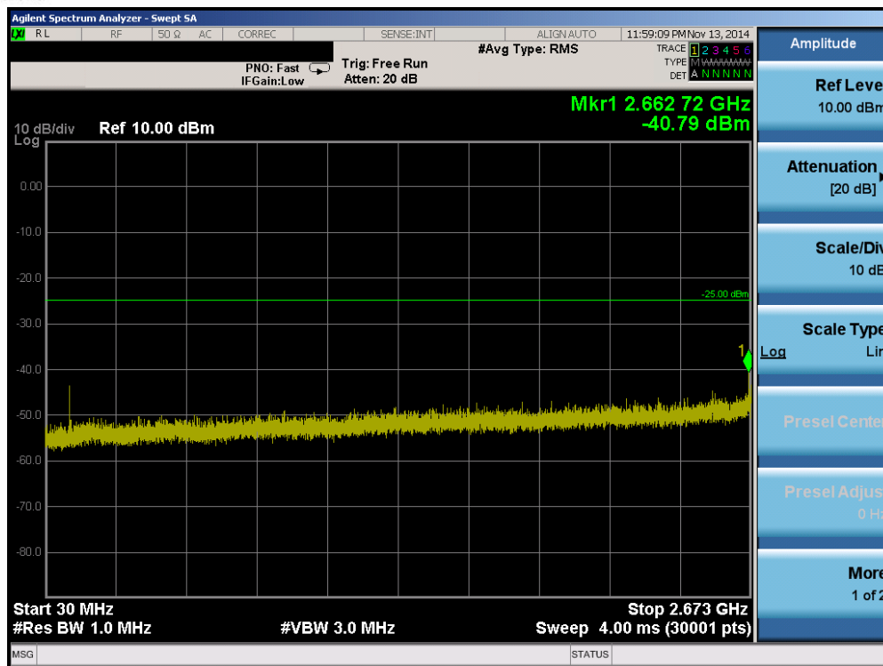
Plot 6-15. Conducted Spurious Plot (Band 41 – 10.0MHz QPSK – RB Size 1, RB Offset 0 – High Channel)
