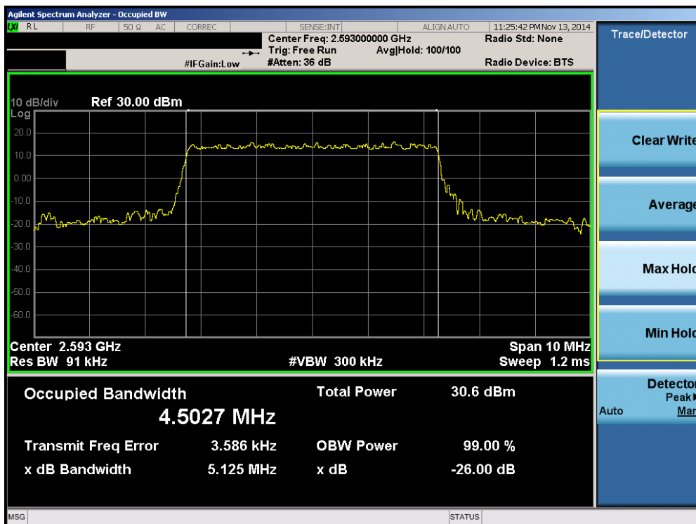
Plot 6-2. Occupied Bandwidth Plot (Band 41 – 5.0MHz 16-QAM – RB Size 25)
