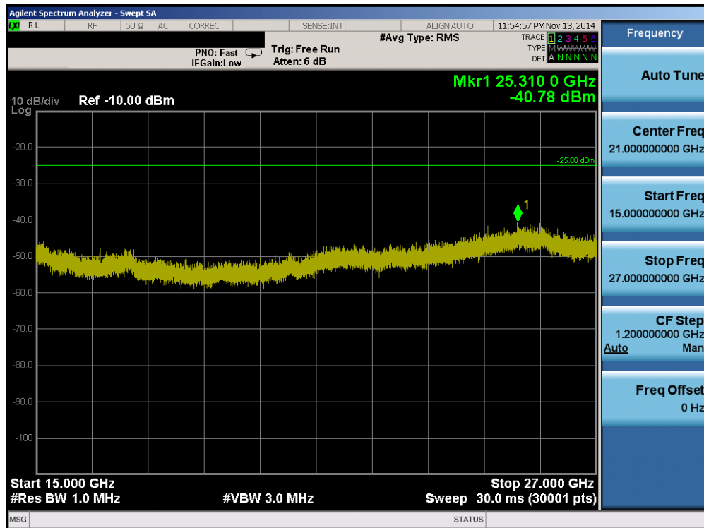
Plot 6-14. Conducted Spurious Plot (Band 41 – 10.0MHz QPSK – RB Size 1, RB Offset 0 – Mid Channel)
