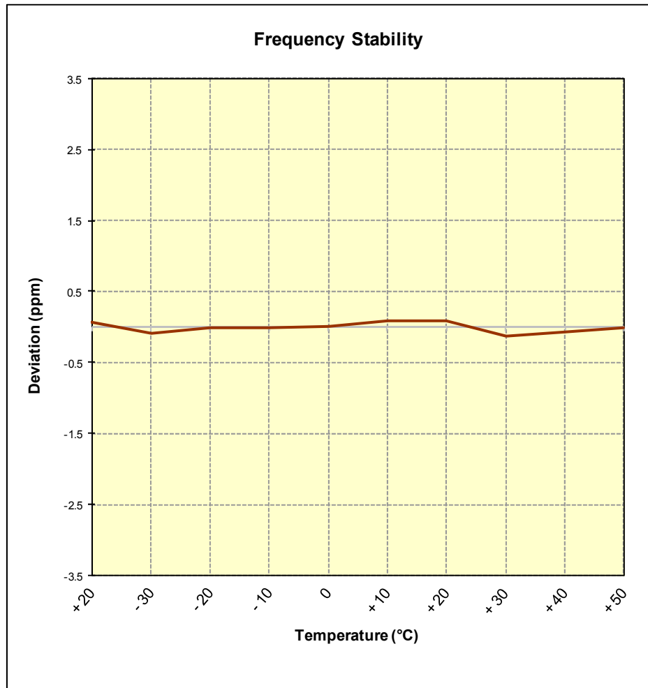
Figure 6-6. Frequency Stability Graph (Band 41)
