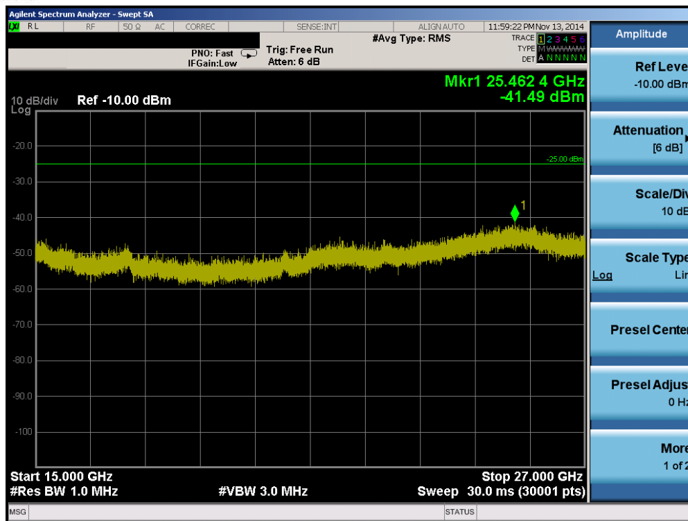
Plot 6-17. Conducted Spurious Plot (Band 41 – 10.0MHz QPSK – RB Size 1, RB Offset 0 – High Channel)
