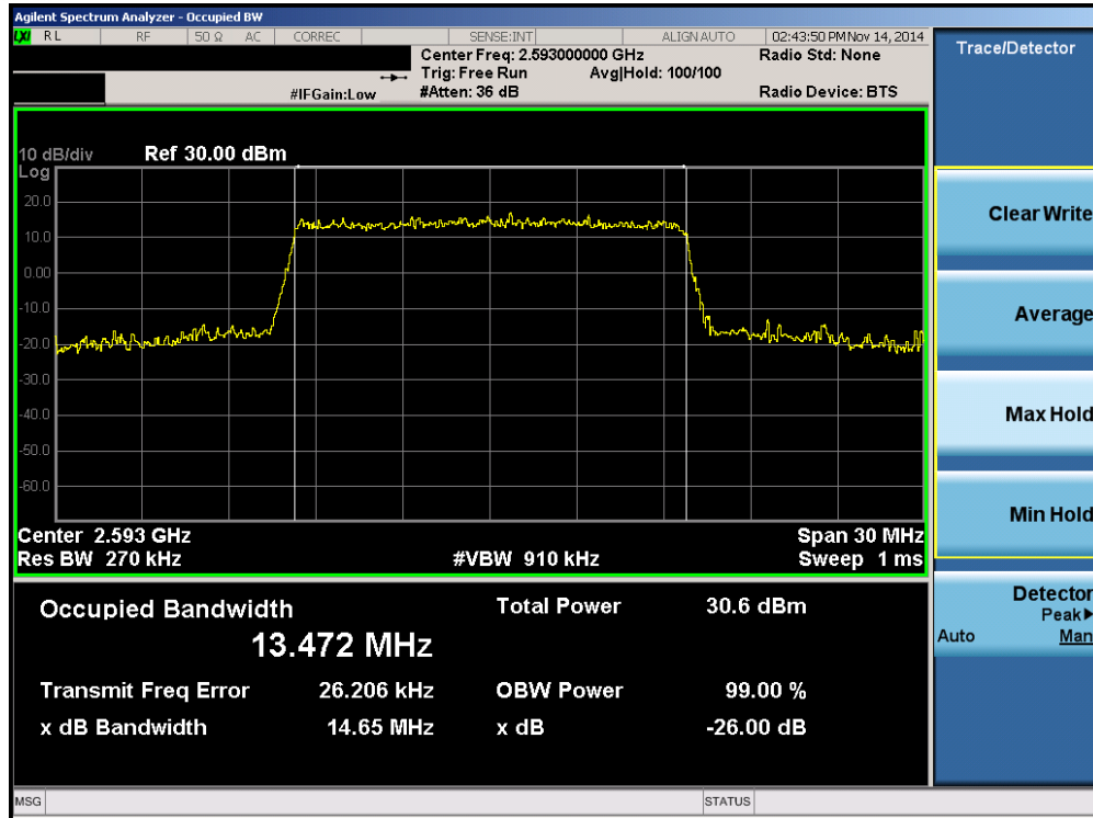
Plot 6-5. Occupied Bandwidth Plot (Band 41 – 15.0MHz QPSK – RB Size 75)
