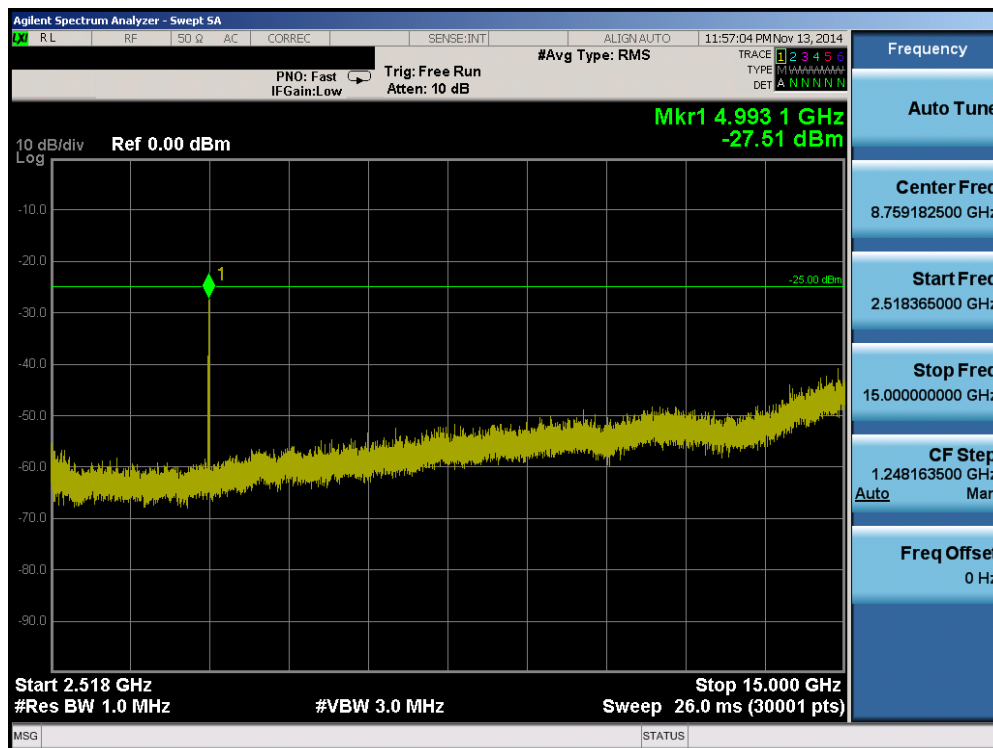
Plot 6-10. Conducted Spurious Plot (Band 41 – 10.0MHz QPSK – RB Size 1, RB Offset 0 – Low Channel)
