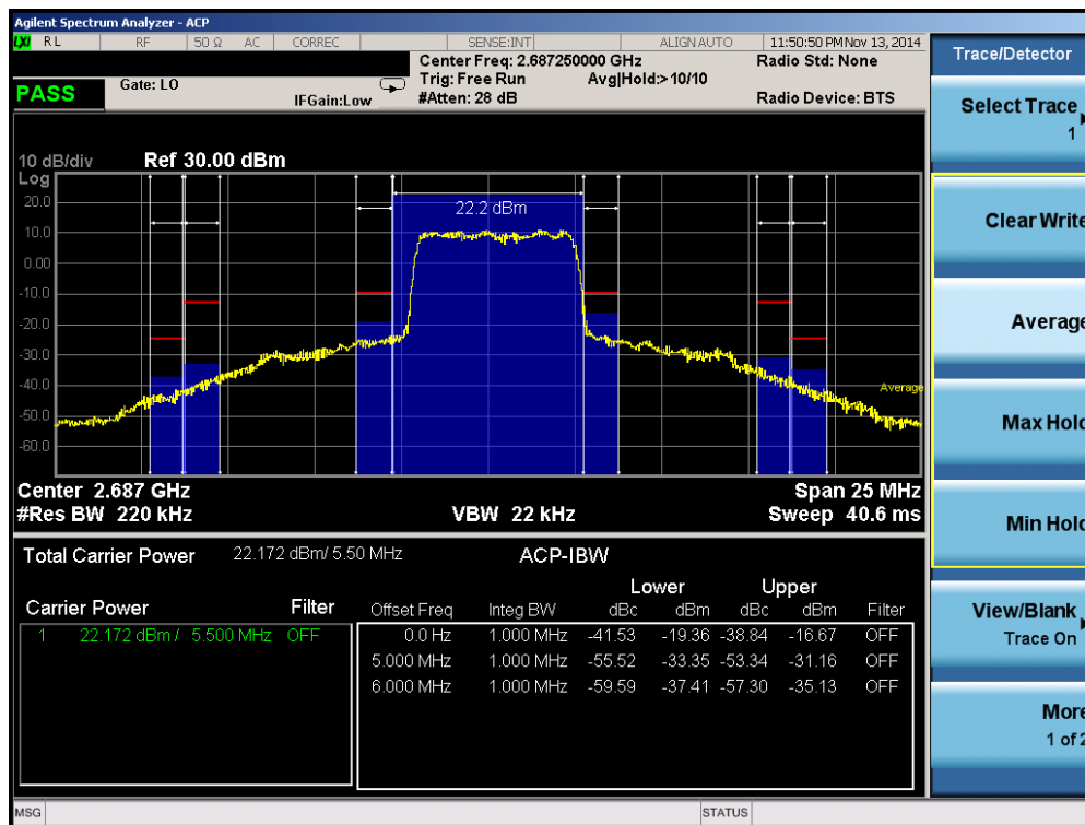
Plot 6-19. Upper ACP Plot (Band 41 – 5.0MHz QPSK – RB Size 25)
