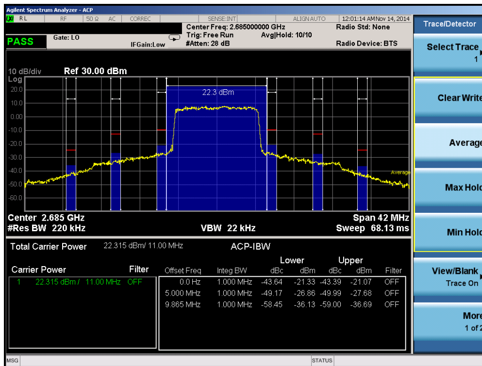
Plot 6-21. Upper ACP Plot (Band 41 – 10.0MHz QPSK – RB Size 50)
