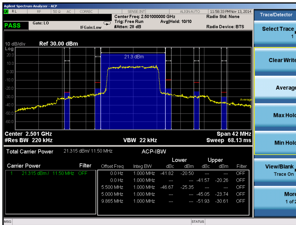
Plot 6-20. Lower ACP Plot (Band 41 – 10.0MHz QPSK – RB Size 50)
