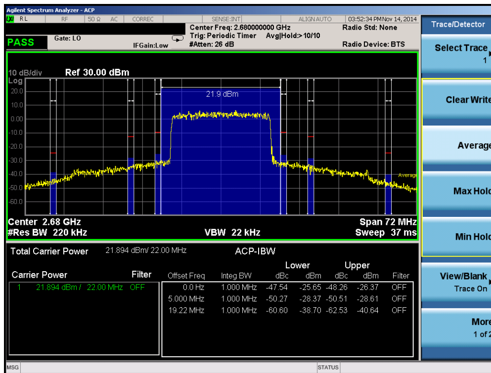
Plot 6-25. Upper ACP Plot (Band 41 – 20.0MHz QPSK – RB Size 100)
