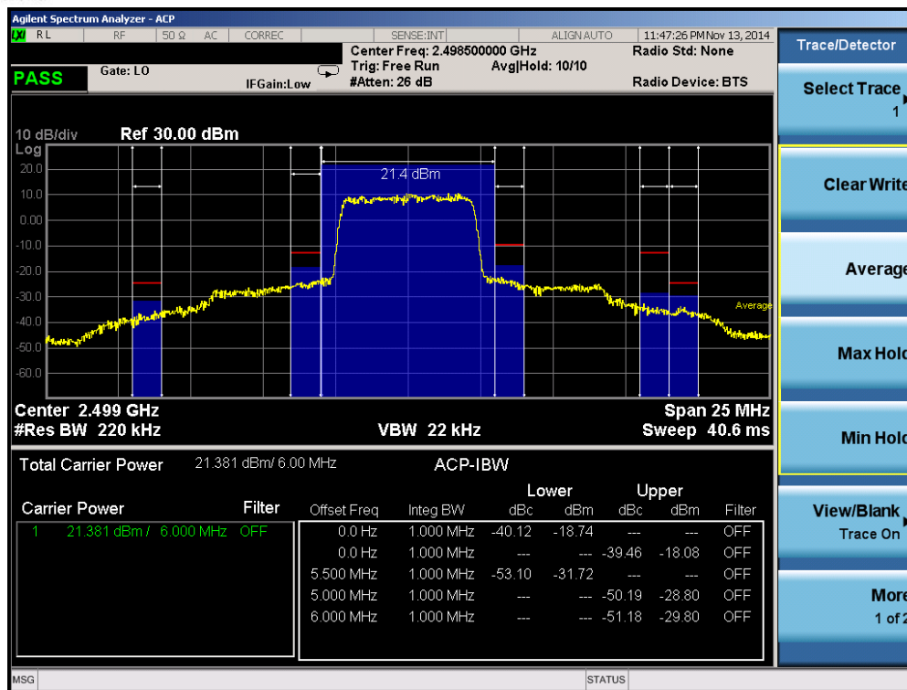
Plot 6-18. Lower ACP Plot (Band 41 – 5.0MHz QPSK – RB Size 25)
