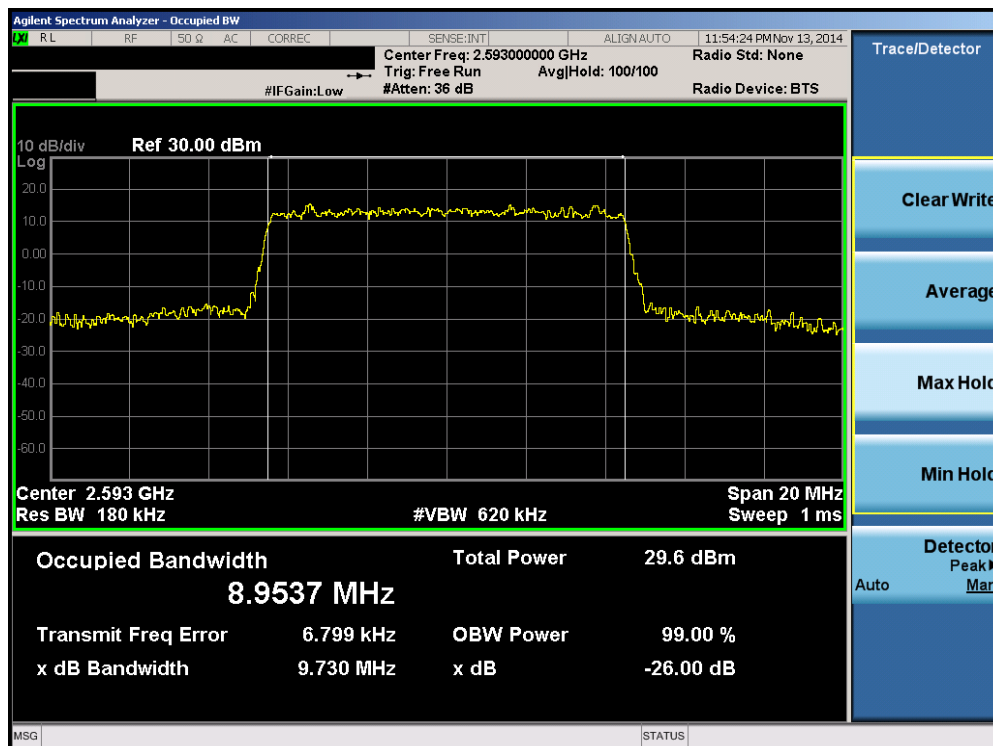
Plot 6-4. Occupied Bandwidth Plot (Band 41 – 10.0MHz 16-QAM – RB Size 50)
