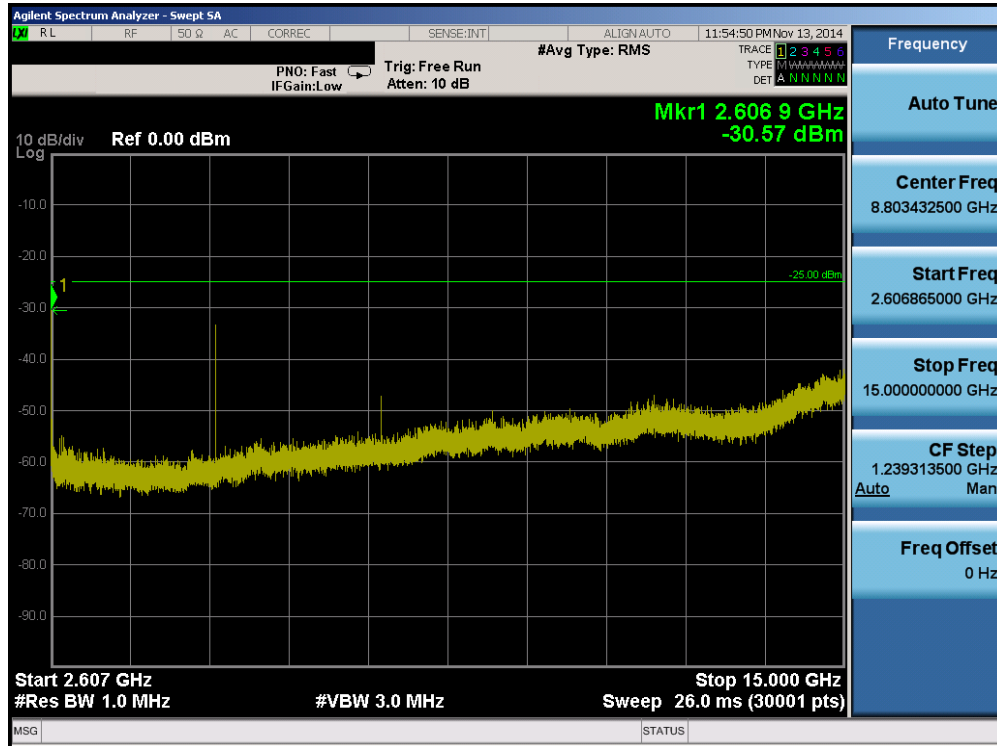
Plot 6-13. Conducted Spurious Plot (Band 41 – 10.0MHz QPSK – RB Size 1, RB Offset 0 – Mid Channel)
