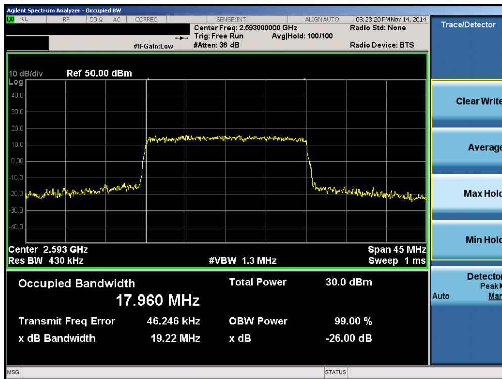
Plot 6-7. Occupied Bandwidth Plot (Band 41 – 20.0MHz QPSK – RB Size 100)
