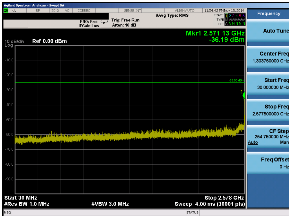
Plot 6-12. Conducted Spurious Plot (Band 41 – 10.0MHz QPSK – RB Size 1, RB Offset 0 – Mid Channel)
