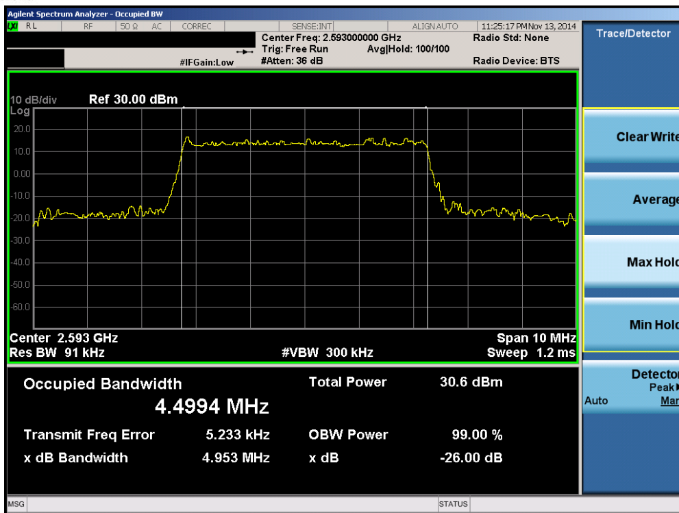
Plot 6-1. Occupied Bandwidth Plot (Band 41 – 5.0MHz QPSK – RB Size 25)
