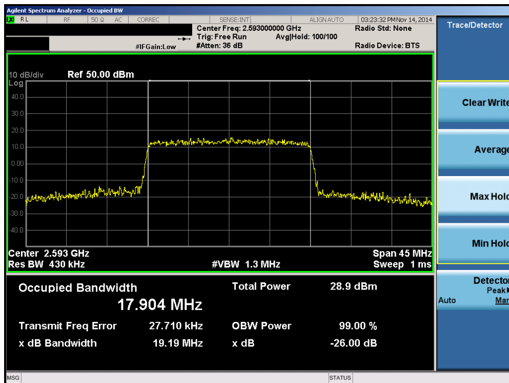
Plot 6-8. Occupied Bandwidth Plot (Band 41 – 20.0MHz 16-QAM – RB Size 100)
