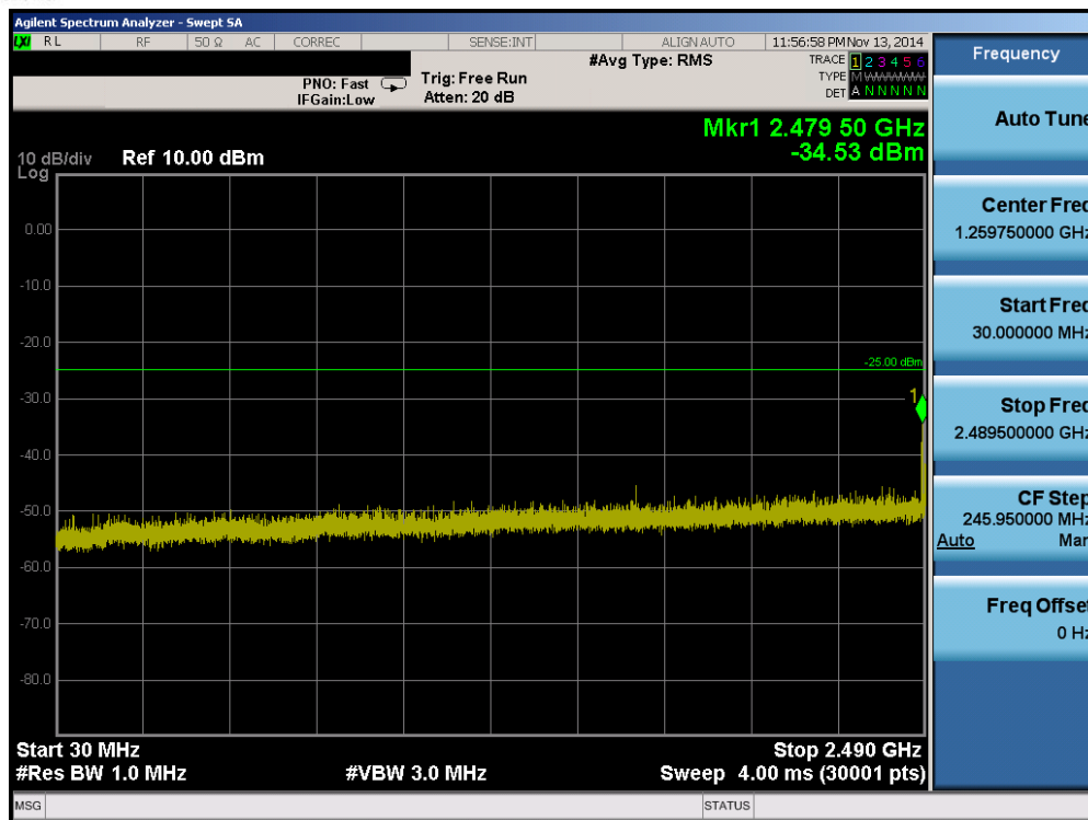
Plot 6-9. Conducted Spurious Plot (Band 41 – 10.0MHz QPSK – RB Size 1, RB Offset 0– Low Channel)
