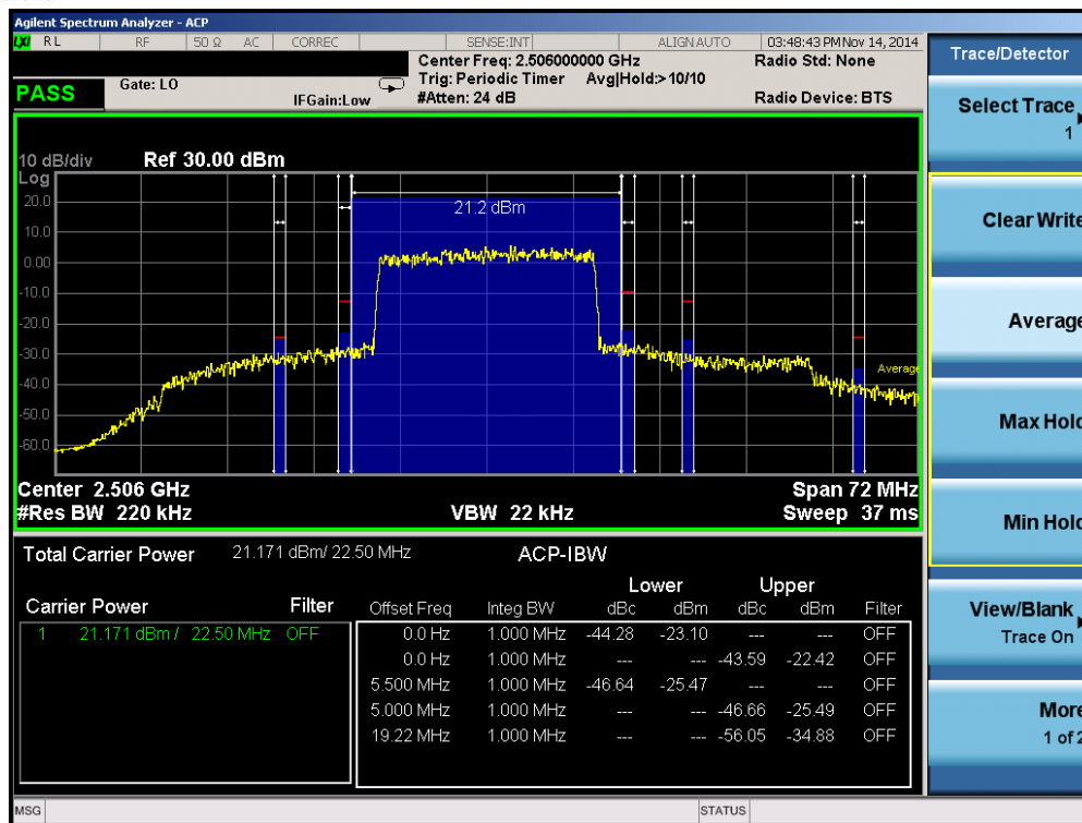
Plot 6-24. Lower ACP Plot (Band 41 – 20.0MHz QPSK – RB Size 100)
