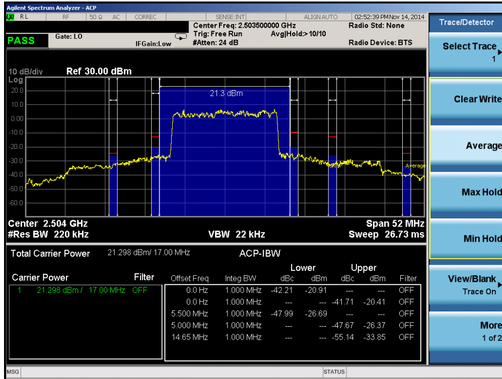
Plot 6-22. Lower ACP Plot (Band 41 – 15.0MHz QPSK – RB Size 75)
