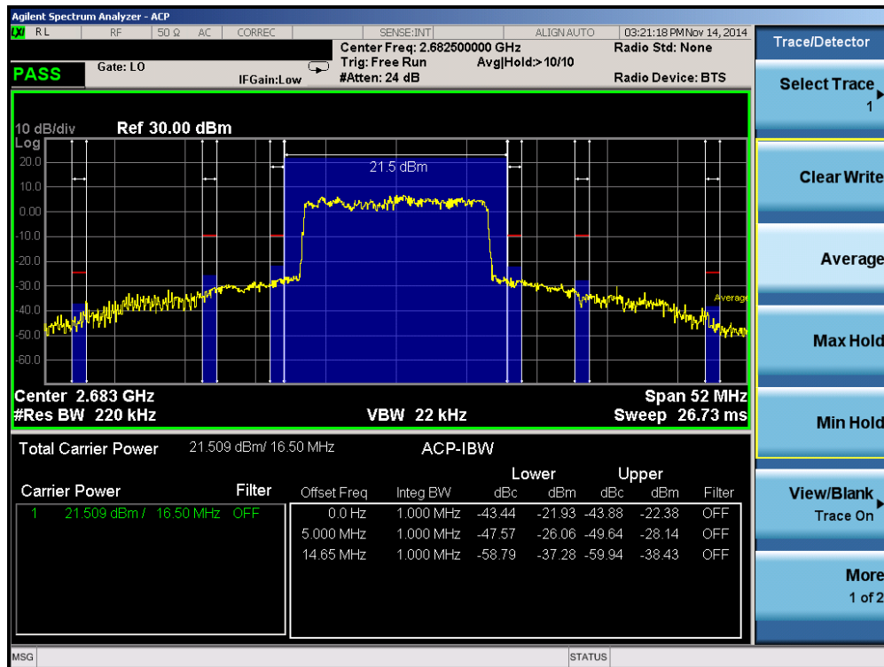
Plot 6-23. Upper ACP Plot (Band 41 – 15.0MHz QPSK – RB Size 75)
