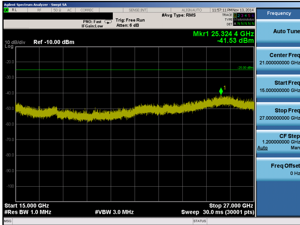
Plot 6-11. Conducted Spurious Plot (Band 41 – 10.0MHz QPSK – RB Size 1, RB Offset 0 – Low Channel)
