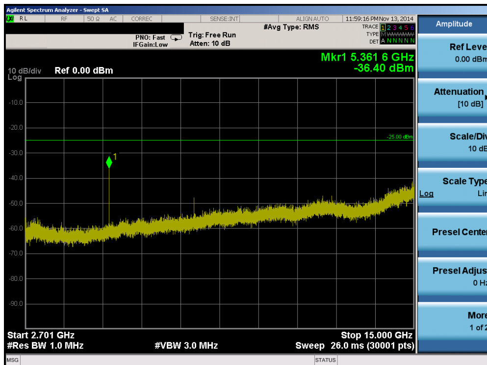
Plot 6-16. Conducted Spurious Plot (Band 41 – 10.0MHz QPSK – RB Size 1, RB Offset 0 – High Channel)
