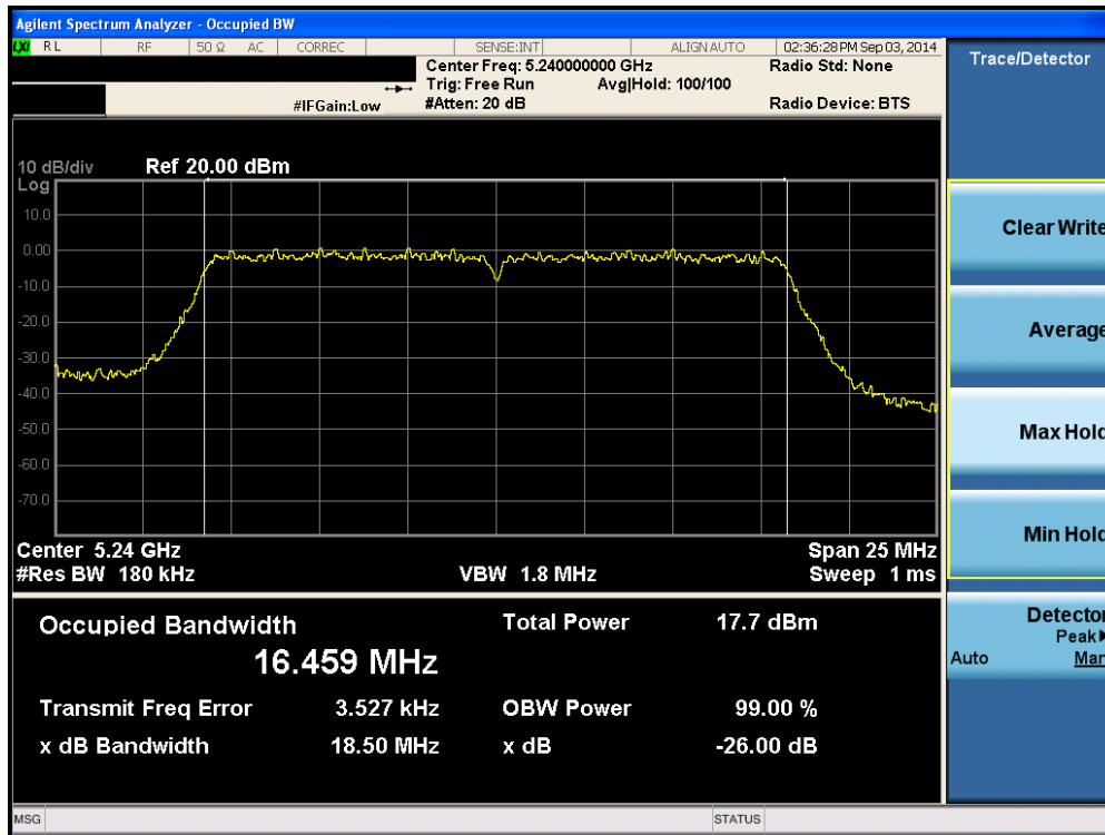
Plot 6-34. 26dB Bandwidth Plot (802.11a (UNII Band 1) – Ch. 48)
