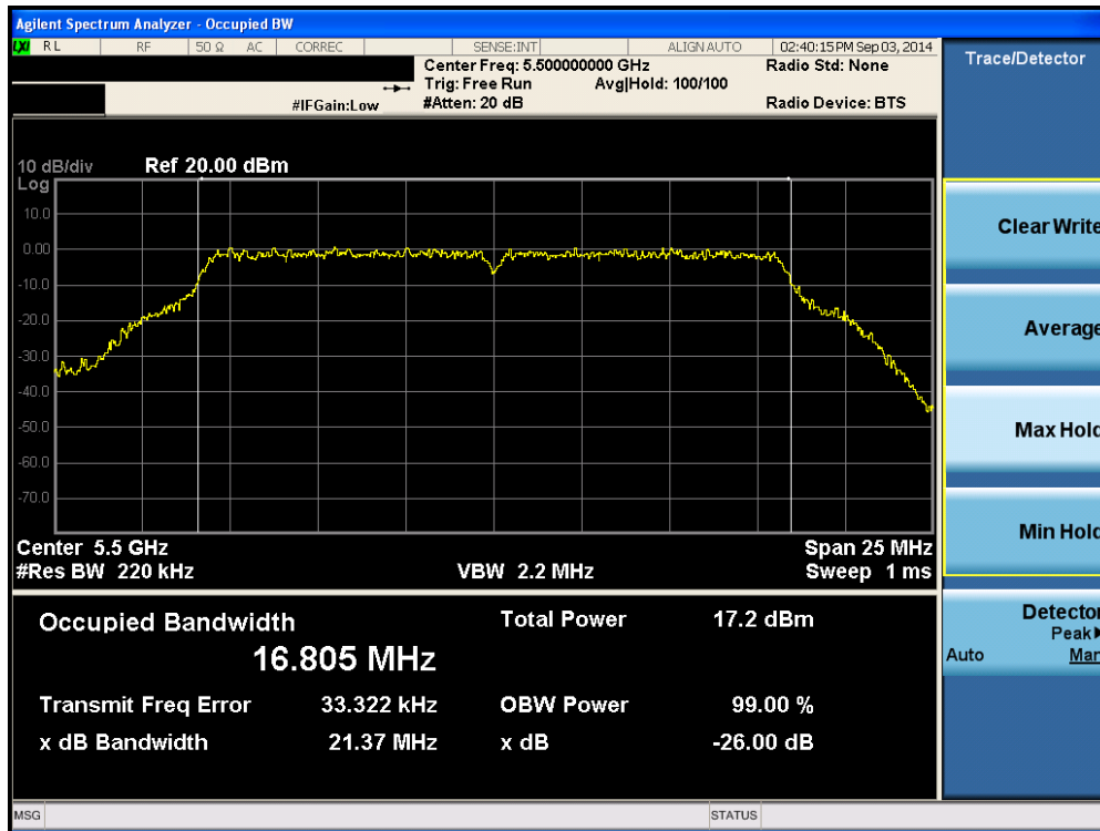
Plot 6-50. 26dB Bandwidth Plot (802.11a (UNII Band 2C) – Ch. 100)
