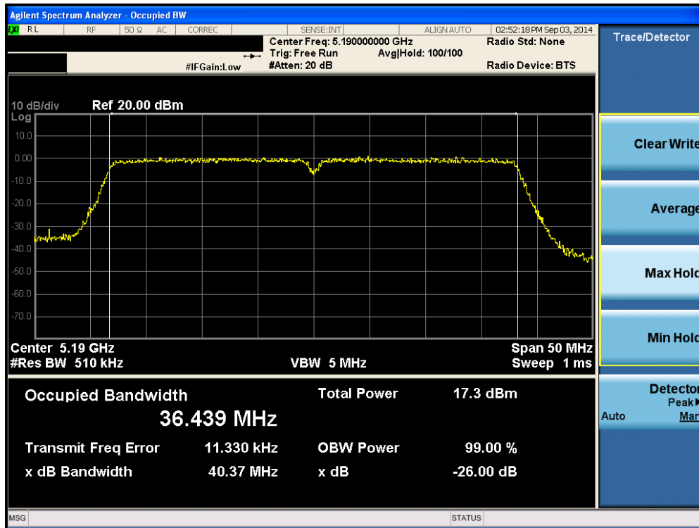
Plot 6-38. 26dB Bandwidth Plot (40MHz BW 802.11n (UNII Band 1) – Ch. 38)
