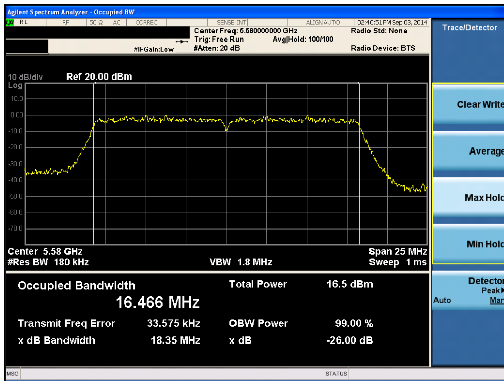
Plot 6-51. 26dB Bandwidth Plot (802.11a (UNII Band 2C) – Ch. 116)
