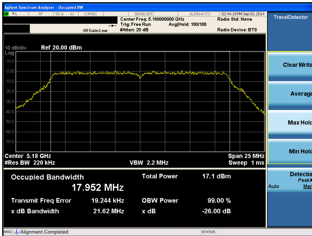
Plot 6-35. 26dB Bandwidth Plot (20MHz BW 802.11n (UNII Band 1) – Ch. 36)
