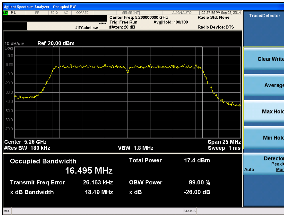
Plot 6-41. 26dB Bandwidth Plot (802.11a (UNII Band 2A) – Ch. 52)
