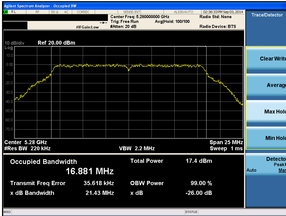
Plot 6-42. 26dB Bandwidth Plot (802.11a (UNII Band 2A) – Ch. 56)
