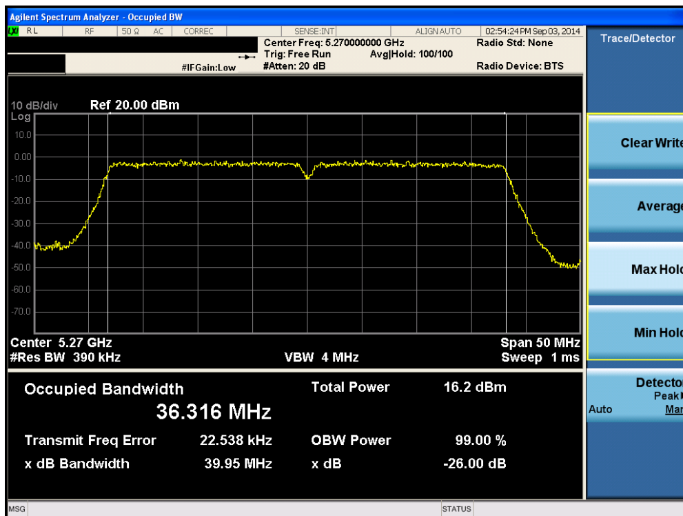
Plot 6-47. 26dB Bandwidth Plot (40MHz BW 802.11n (UNII Band 2A) – Ch. 54)
