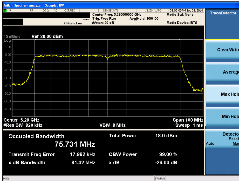
Plot 6-49. 26dB Bandwidth Plot (80MHz BW 802.11ac (UNII Band 2A) – Ch. 58)
