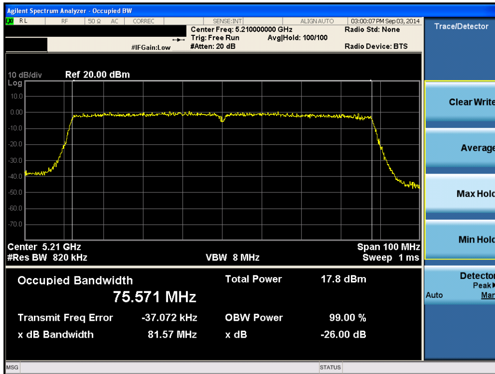
Plot 6-40. 26dB Bandwidth Plot (80MHz BW 802.11ac (UNII Band 1) – Ch. 42)
