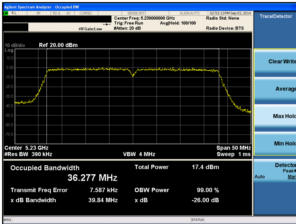
Plot 6-39. 26dB Bandwidth Plot (40MHz BW 802.11n (UNII Band 1) – Ch. 46)
