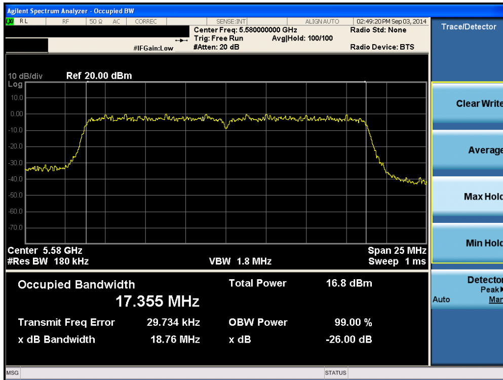
Plot 6-54. 26dB Bandwidth Plot (20MHz BW 802.11n (UNII Band 2C) – Ch. 116)
