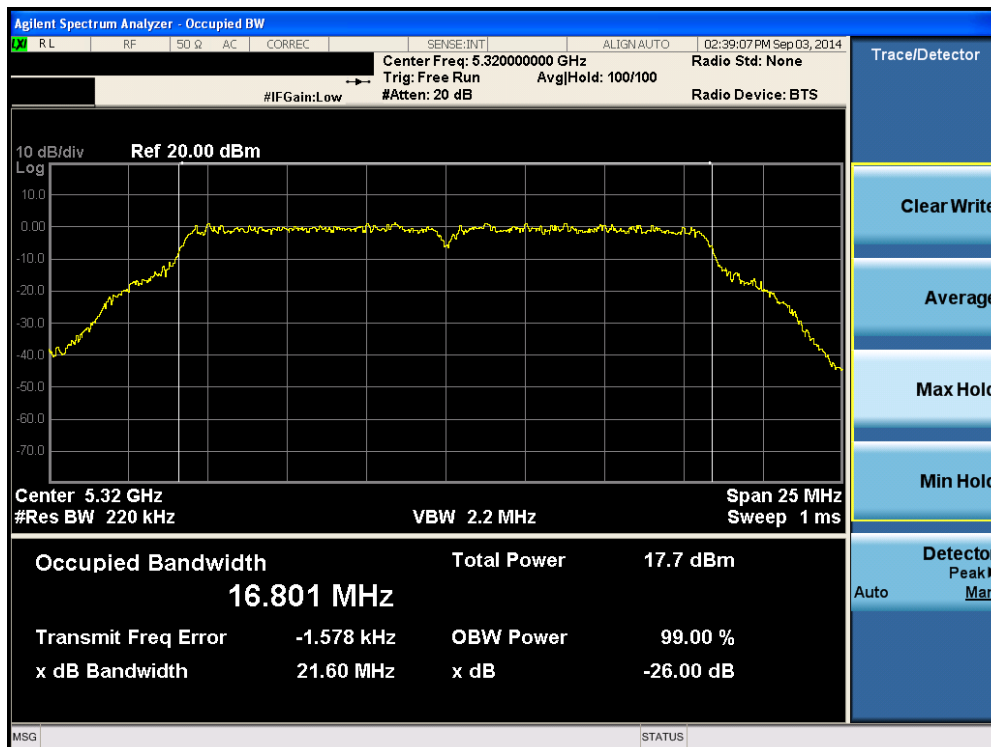
Plot 6-43. 26dB Bandwidth Plot (802.11a (UNII Band 2A) – Ch. 64)
