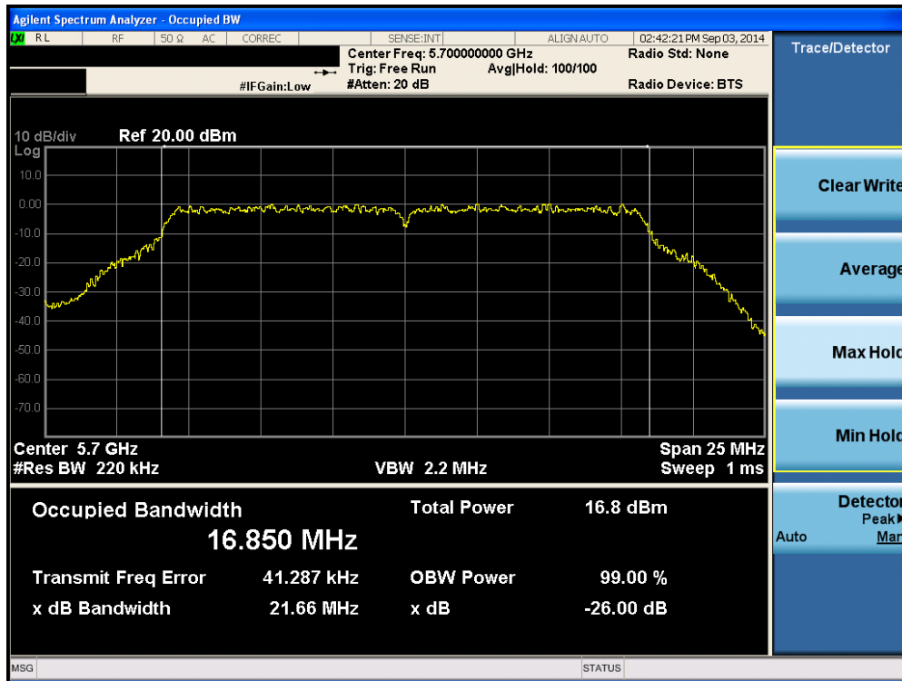
Plot 6-52. 26dB Bandwidth Plot (802.11a (UNII Band 2C) – Ch. 140)
