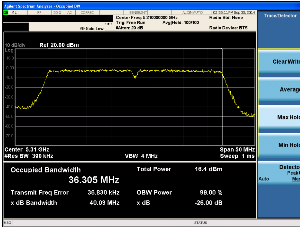
Plot 6-48. 26dB Bandwidth Plot (40MHz BW 802.11n (UNII Band 2A) – Ch. 62)
