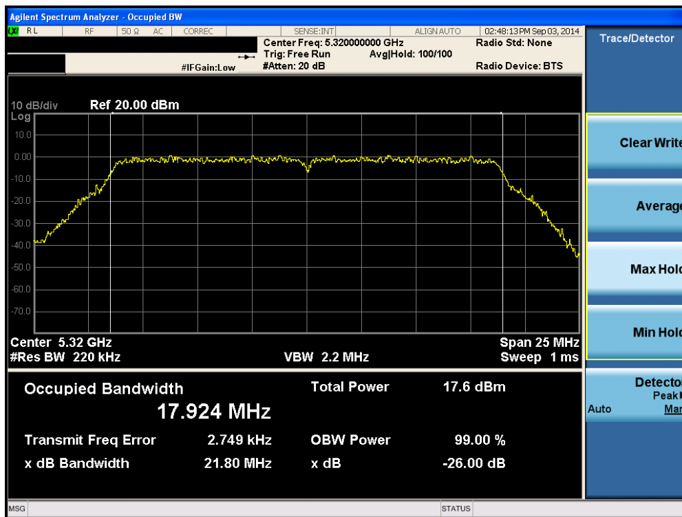
Plot 6-46. 26dB Bandwidth Plot (20MHz BW 802.11n (UNII Band 2A) – Ch. 64)
