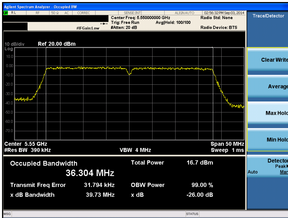
Plot 6-57. 26dB Bandwidth Plot (40MHz BW 802.11n (UNII Band 2C) – Ch. 110)
