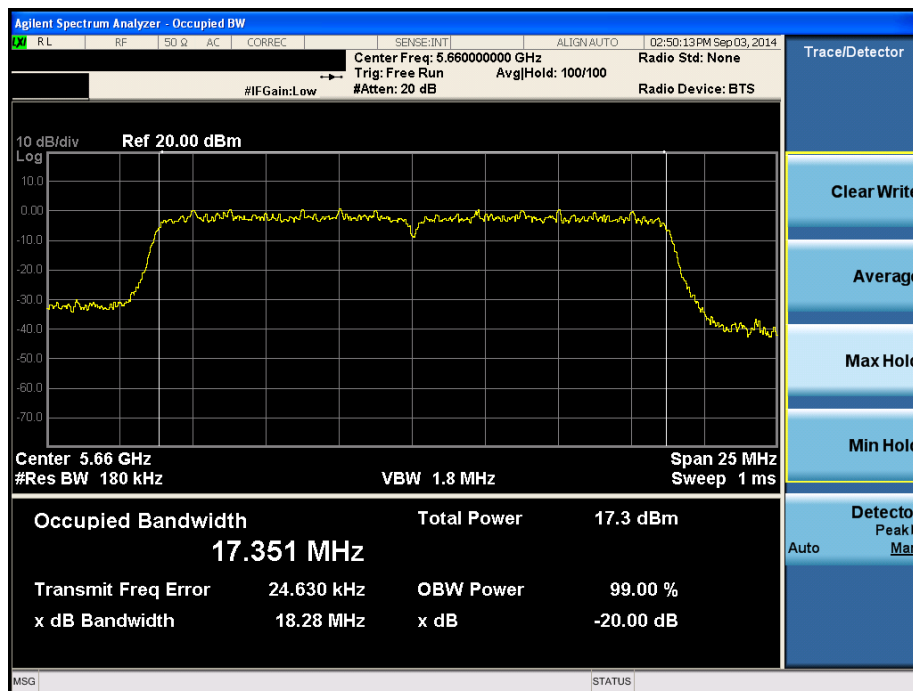
Plot 6-60. 20dB Bandwidth Plot (20MHz BW 802.11n (UNII Band 2C) – Ch. 132)
