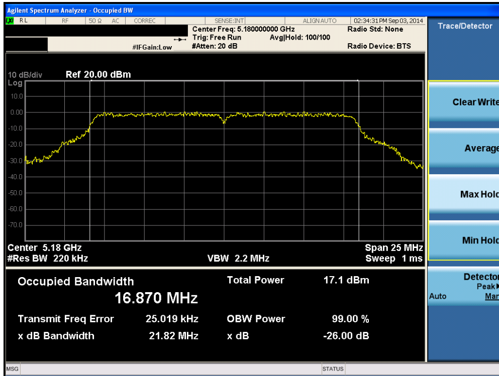
Plot 6-32. 26dB Bandwidth Plot (802.11a (UNII Band 1) – Ch. 36)
