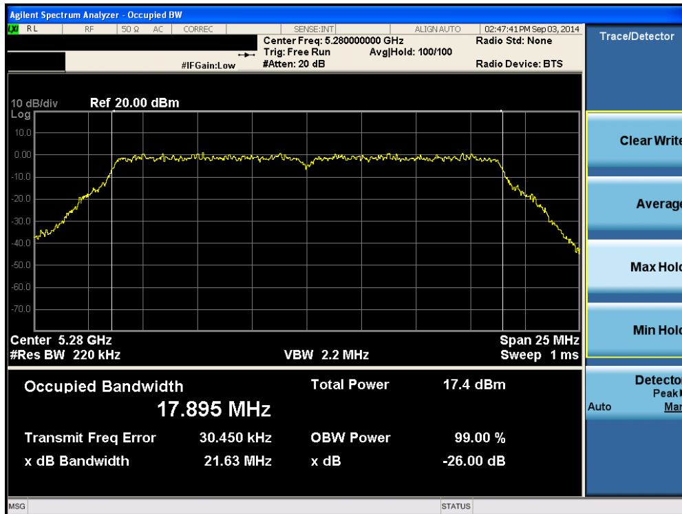
Plot 6-45. 26dB Bandwidth Plot (20MHz BW 802.11n (UNII Band 2A) – Ch. 56)
