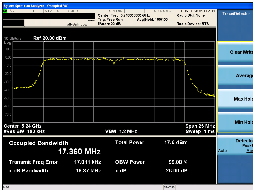
Plot 6-37. 26dB Bandwidth Plot (20MHz BW 802.11n (UNII Band 1) – Ch. 48)
