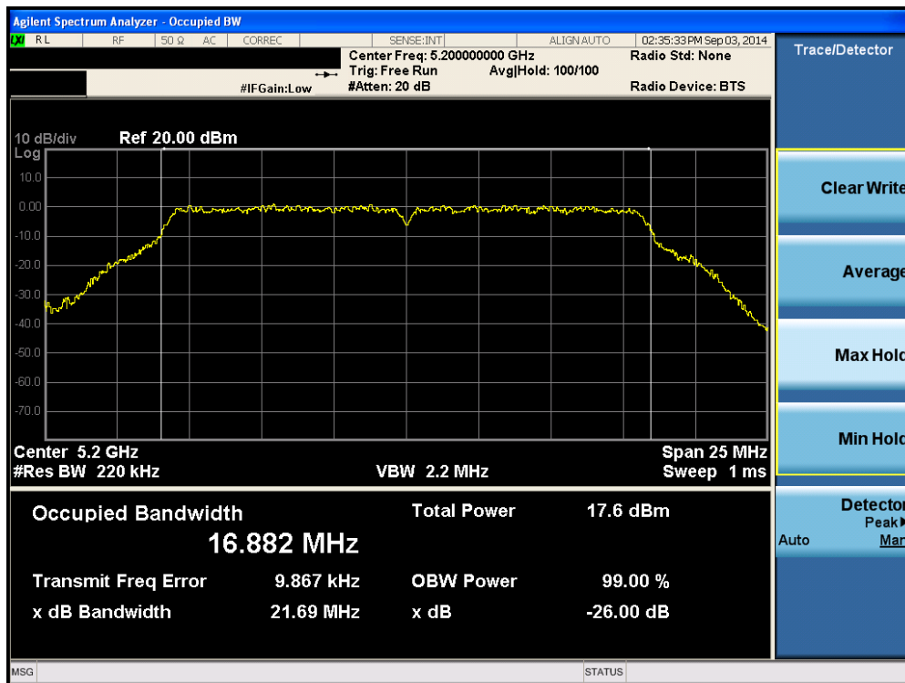
Plot 6-33. 26dB Bandwidth Plot (802.11a (UNII Band 1) – Ch. 40)
