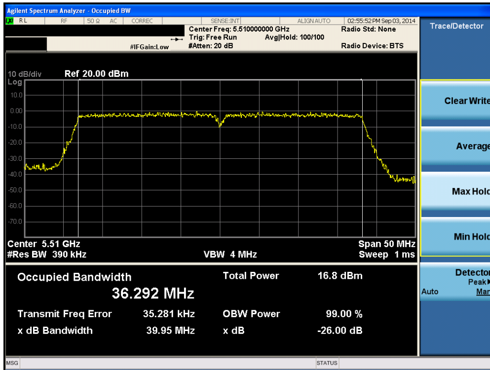
Plot 6-56. 26dB Bandwidth Plot (40MHz BW 802.11n (UNII Band 2C) – Ch. 102)
