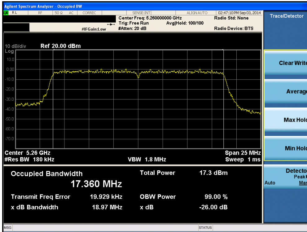
Plot 6-44. 26dB Bandwidth Plot (20MHz BW 802.11n (UNII Band 2A) – Ch. 52)
