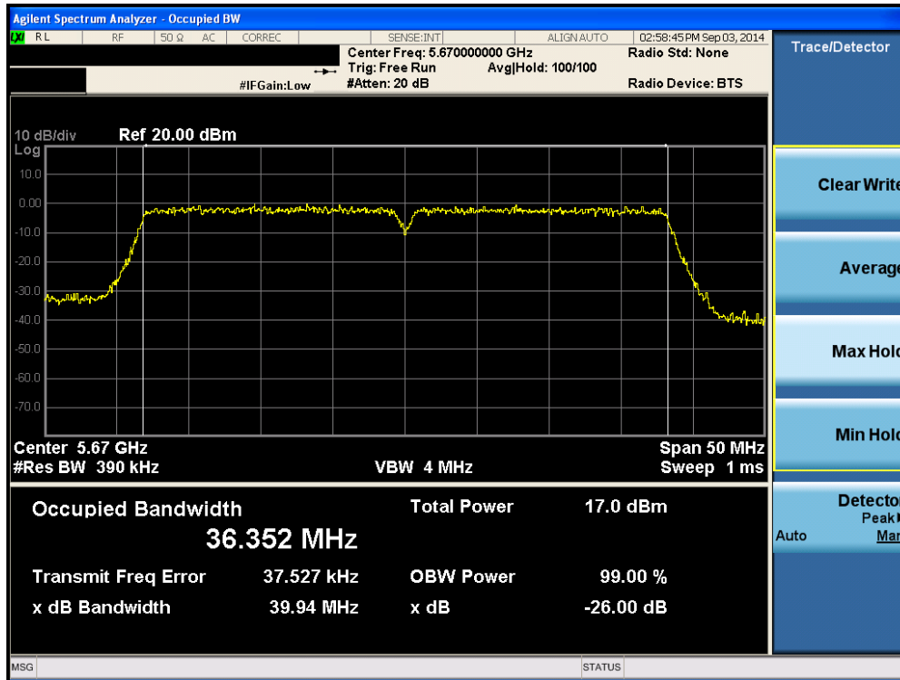
Plot 6-58. 26dB Bandwidth Plot (40MHz BW 802.11n (UNII Band 2C) – Ch. 134)
