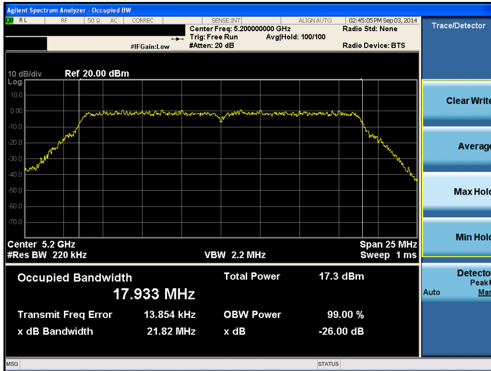
Plot 6-36. 26dB Bandwidth Plot (20MHz BW 802.11n (UNII Band 1) – Ch. 40)
