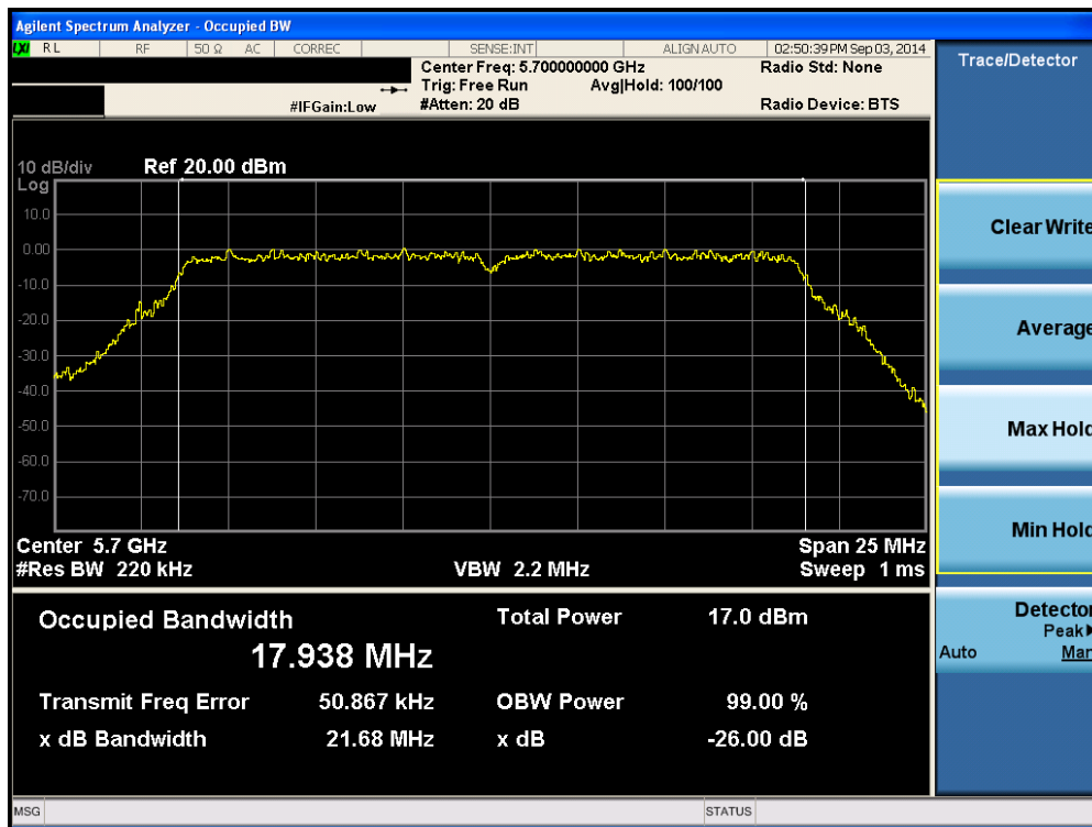
Plot 6-55. 26dB Bandwidth Plot (20MHz BW 802.11n (UNII Band 2C) – Ch. 140)
