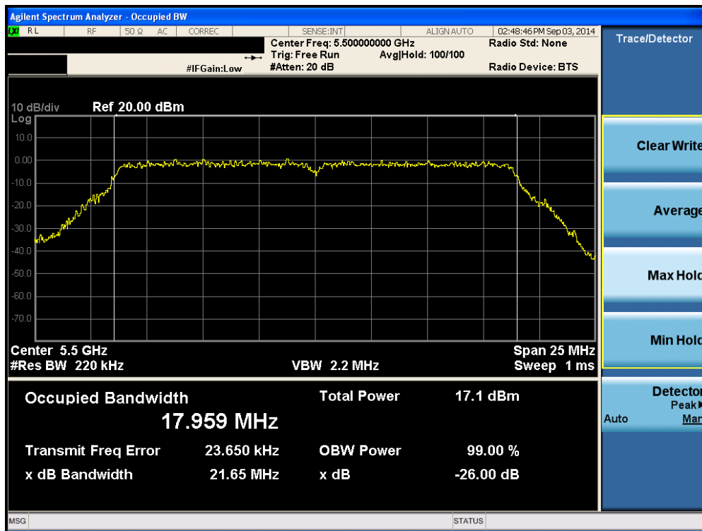
Plot 6-53. 26dB Bandwidth Plot (20MHz BW 802.11n (UNII Band 2C) – Ch. 100)
