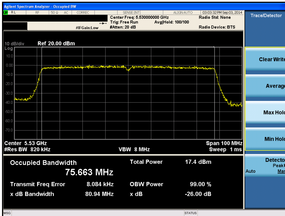
Plot 6-59. 26dB Bandwidth Plot (80MHz BW 802.11ac (UNII Band 2C) – Ch. 106)
