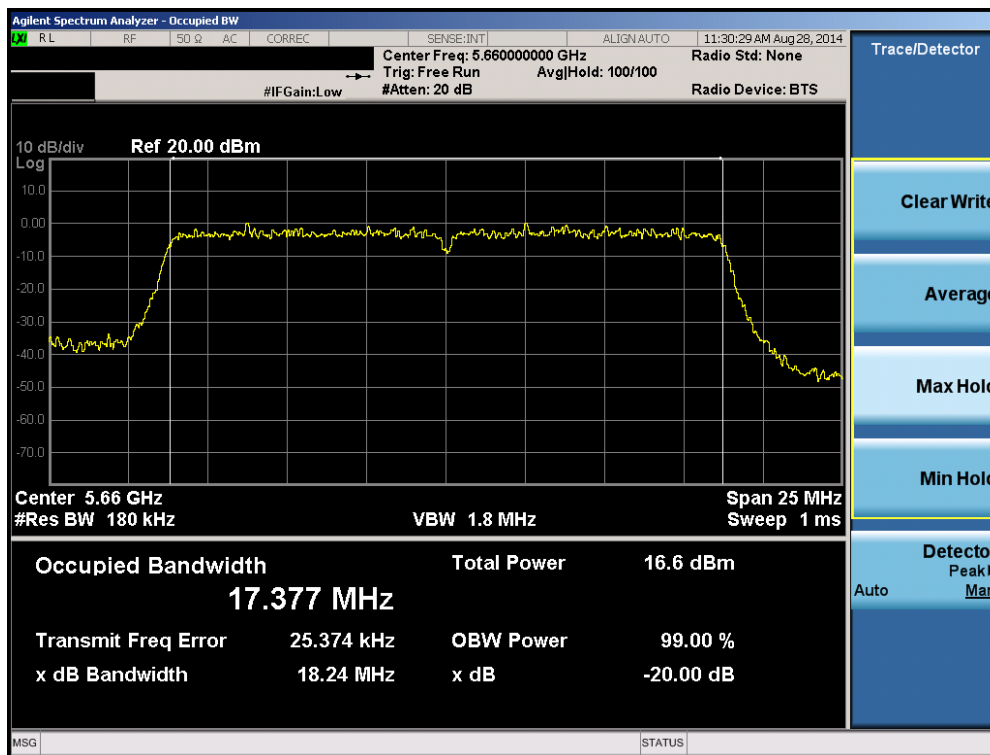
Plot 6-29. 20dB Bandwidth Plot (20MHz BW 802.11n (UNII Band 2C) – Ch. 132)
