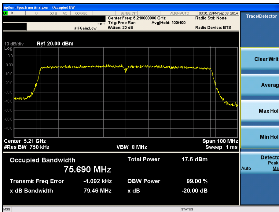
Plot 6-61. 20dB Bandwidth Plot (80MHz BW 802.11ac (UNII Band 1) – Ch. 42)
