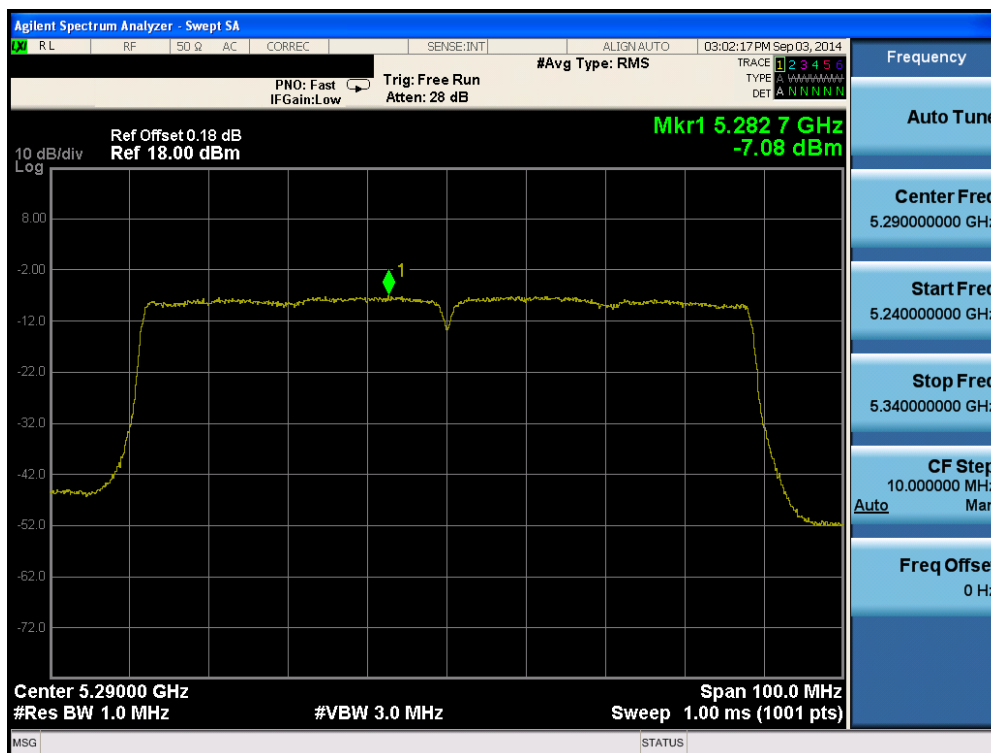
Plot 6-107. Peak Power Spectral Density Plot (80MHz BW 802.11ac (UNII Band 2A) – Ch. 58)
