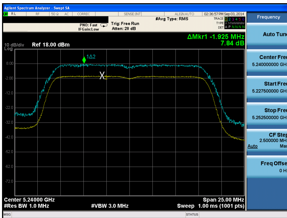
Plot 6-122. Peak Excursion Ratio Plot (802.11a (UNII Band 1) – Ch. 48)
