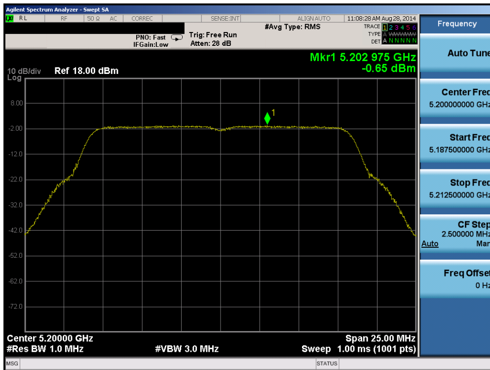
Plot 6-63. Peak Power Spectral Density Plot (802.11a (UNII Band 1) – Ch. 40)
