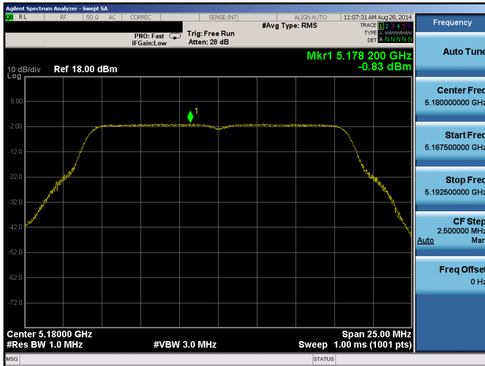
Plot 6-62. Peak Power Spectral Density Plot (802.11a (UNII Band 1) – Ch. 36)
