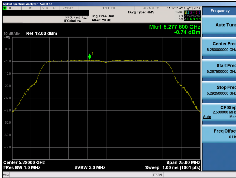
Plot 6-72. Peak Power Spectral Density Plot (802.11a (UNII Band 2A) – Ch. 56)
