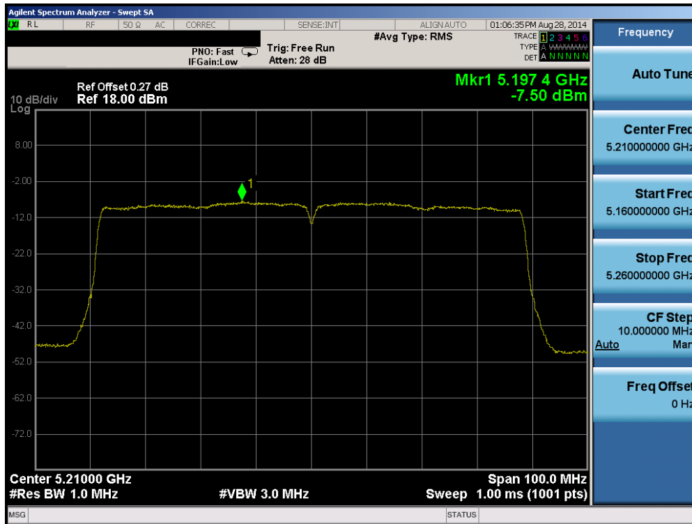
Plot 6-70. Peak Power Spectral Density Plot (80MHz BW 802.11ac (UNII Band 1) – Ch. 42)
