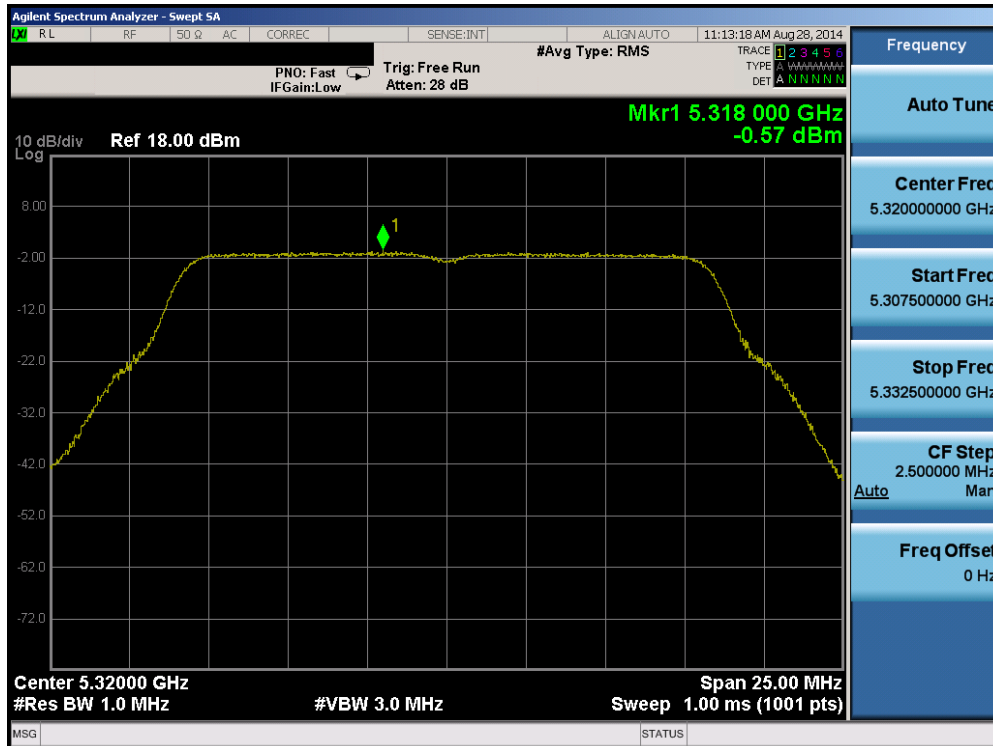
Plot 6-73. Peak Power Spectral Density Plot (802.11a (UNII Band 2A) – Ch. 64)
