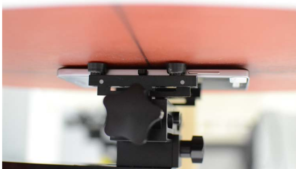
SAR Test Setup Photo 6 – Back Side at 0.0 cm
