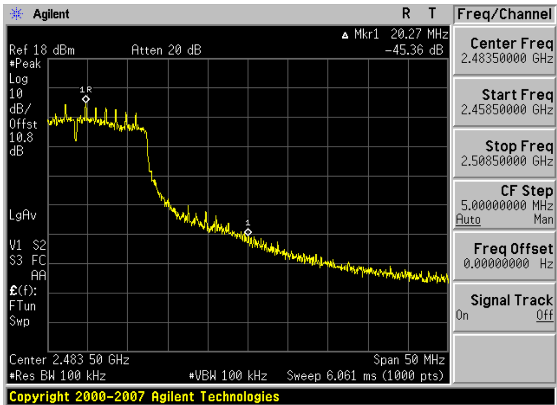
Plot 6-12. Band Edge Plot (802.11n – Ch. 11)
