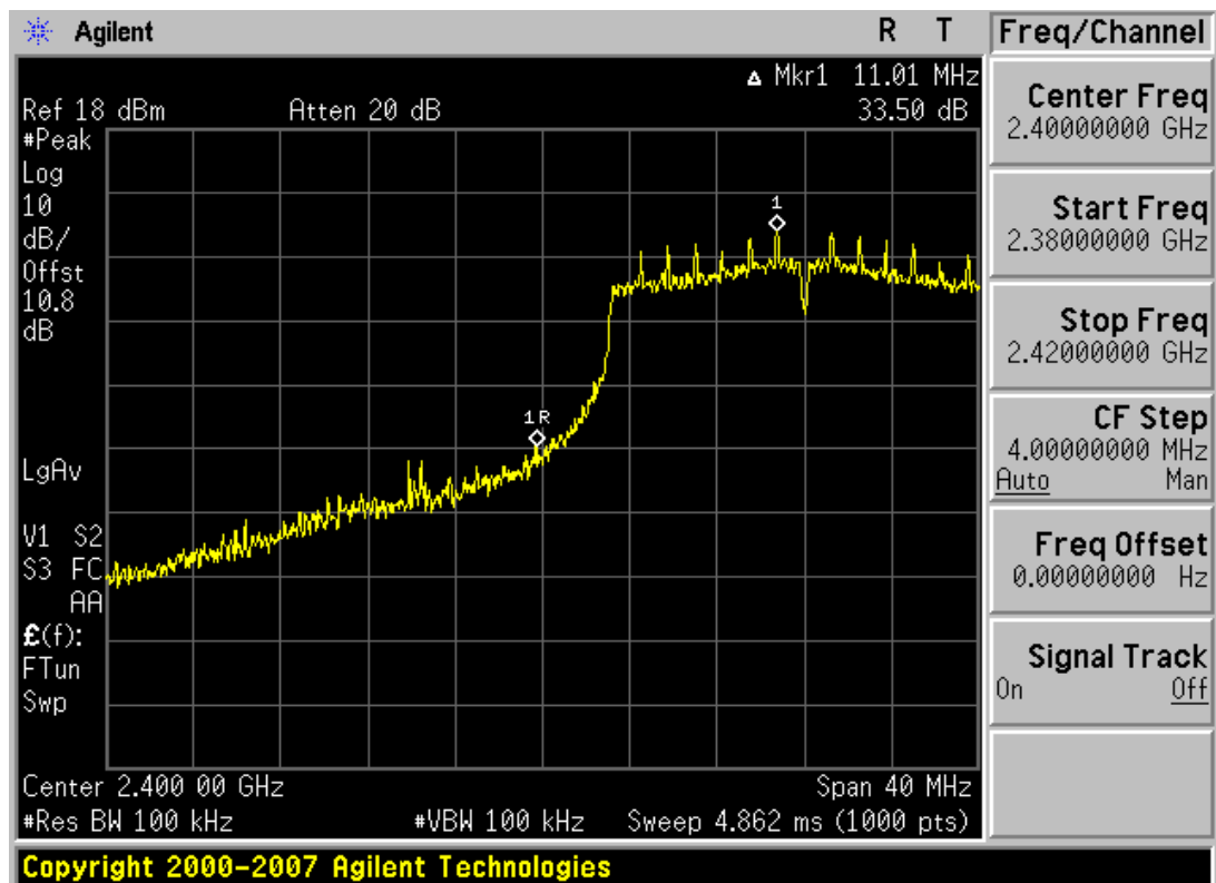
Plot 6-11. Band Edge Plot (802.11n – Ch. 1)
