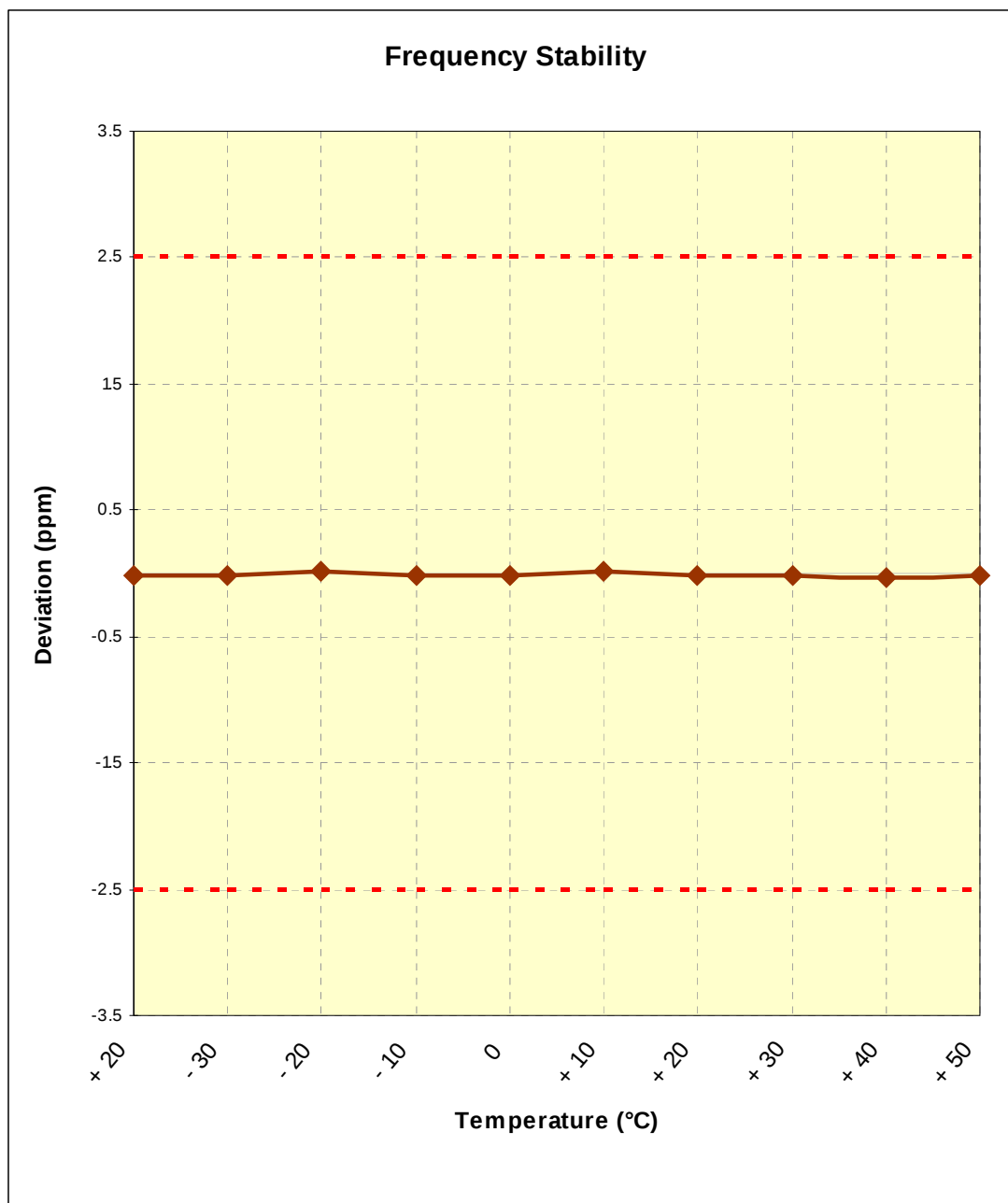
Figure 6-1. Frequency Stability Graph (Cellular GSM Mode – Ch. 190)
