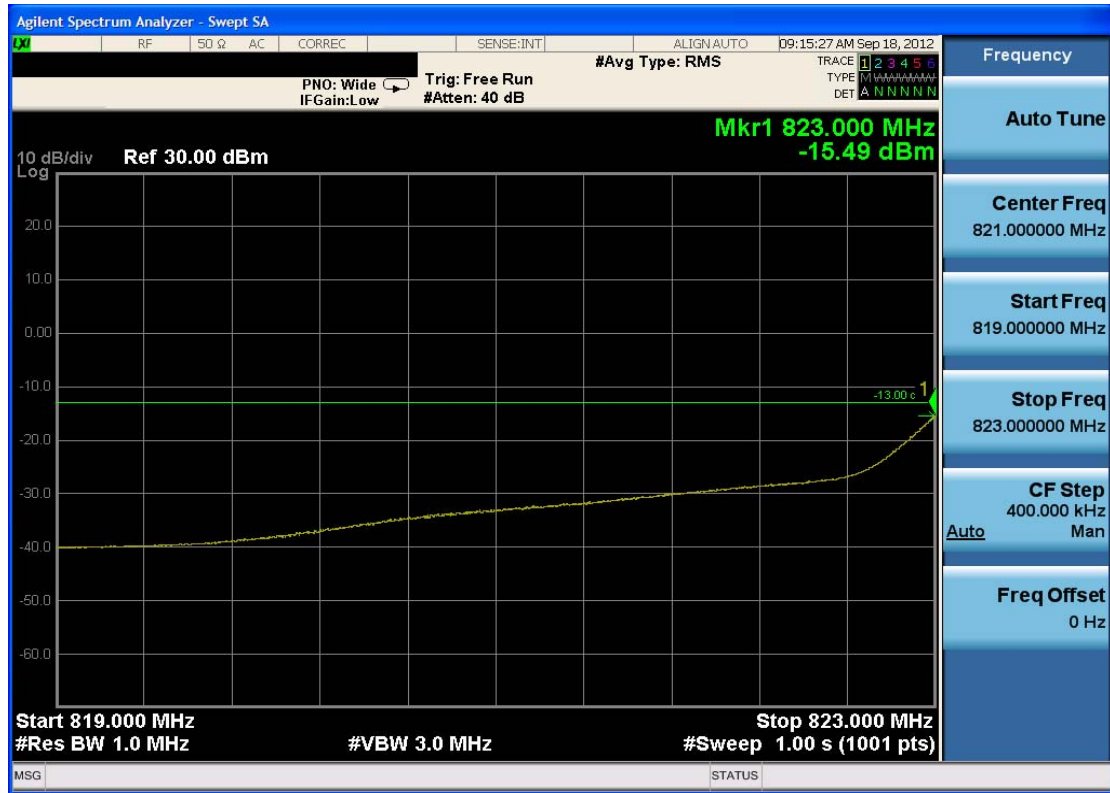
Plot 7-29. 4MHz Span Plot (Cellular WCDMA Mode – Ch. 4132)
