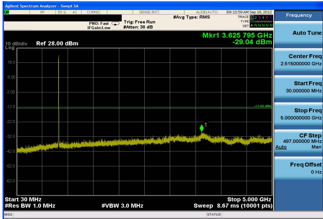
Plot 7-33. Conducted Spurious Plot (Cellular WCDMA Mode – Ch. 4233)
