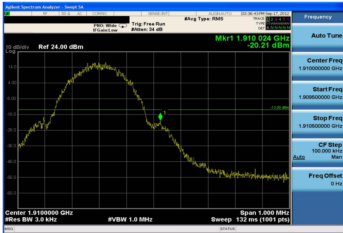
Plot 7-23. Band Edge Plot (PCS GSM Mode – Ch. 810)
