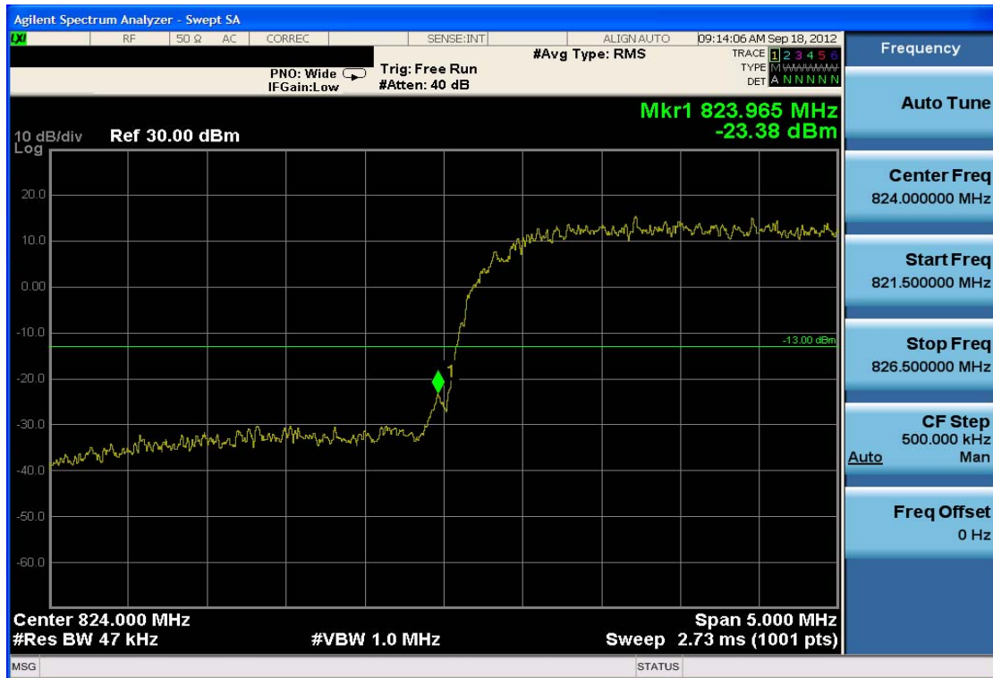
Plot 7-28. Band Edge Plot (Cellular WCDMA Mode – Ch. 4132)
