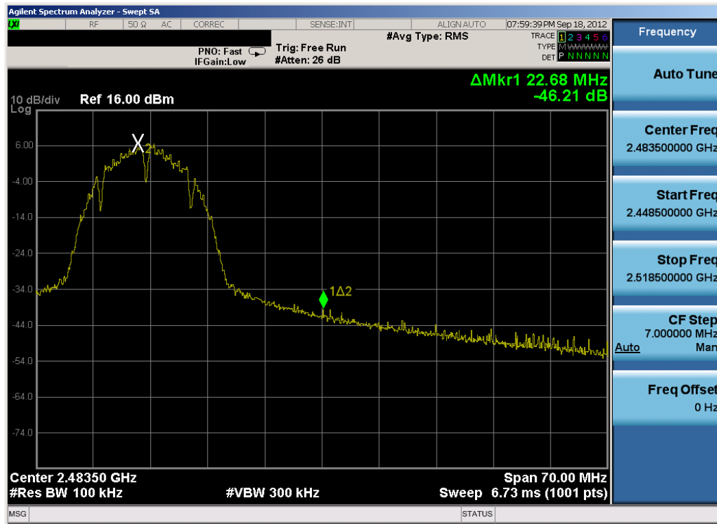
Plot 6-36. Band Edge Plot (802.11b - Ch. 11)
