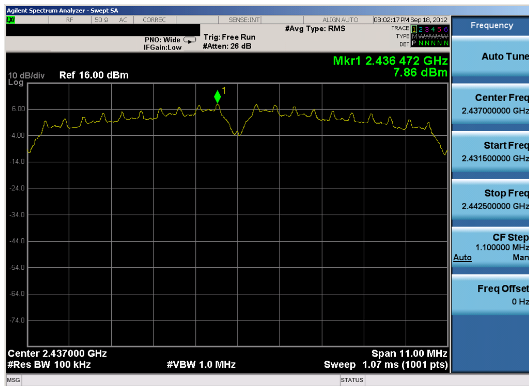
Plot 6-19. Power Spectral Density Plot (802.11b – Ch. 6)
