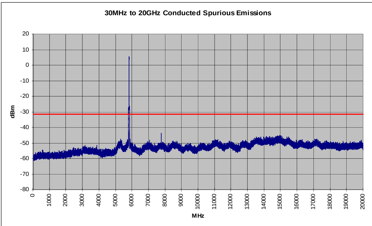
Plot 6-57. Conducted Spurious Plot (802.11a – Ch. 165)
