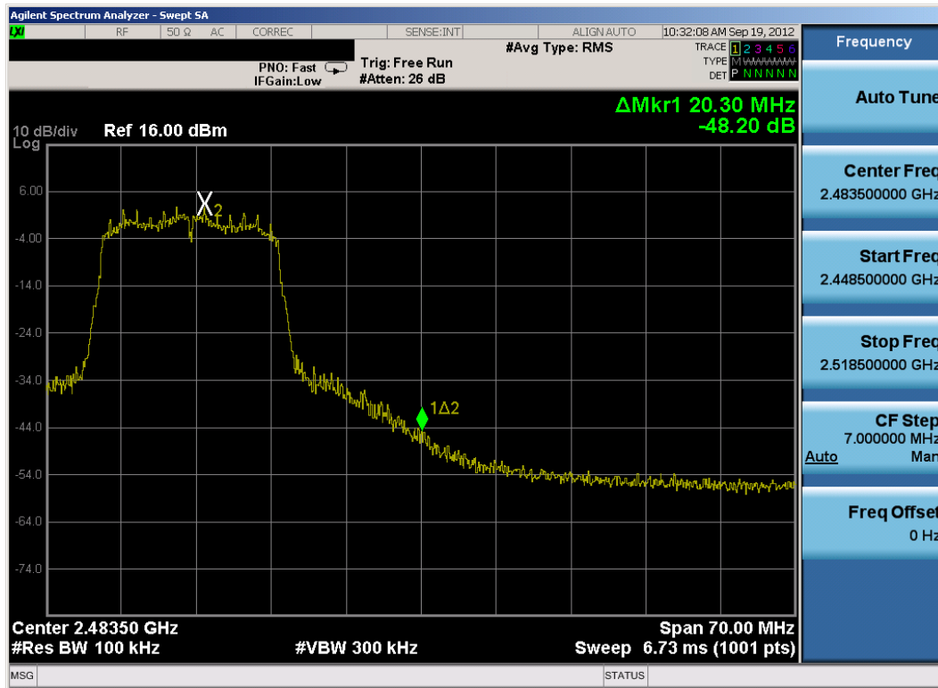
Plot 6-38. Band Edge Plot (802.11g – Ch. 11)
