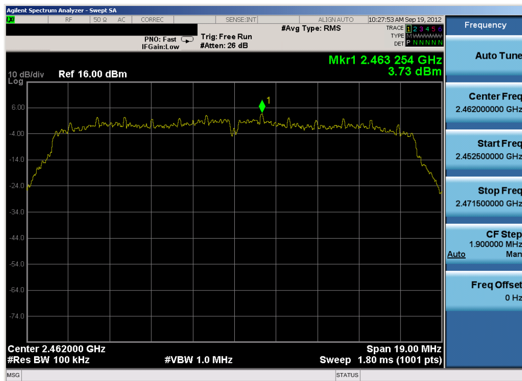
Plot 6-23. Power Spectral Density Plot (802.11g – Ch. 11)
