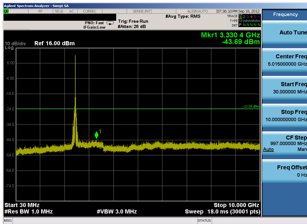
Plot 6-51. Conducted Spurious Plot (802.11b – Ch. 11)
