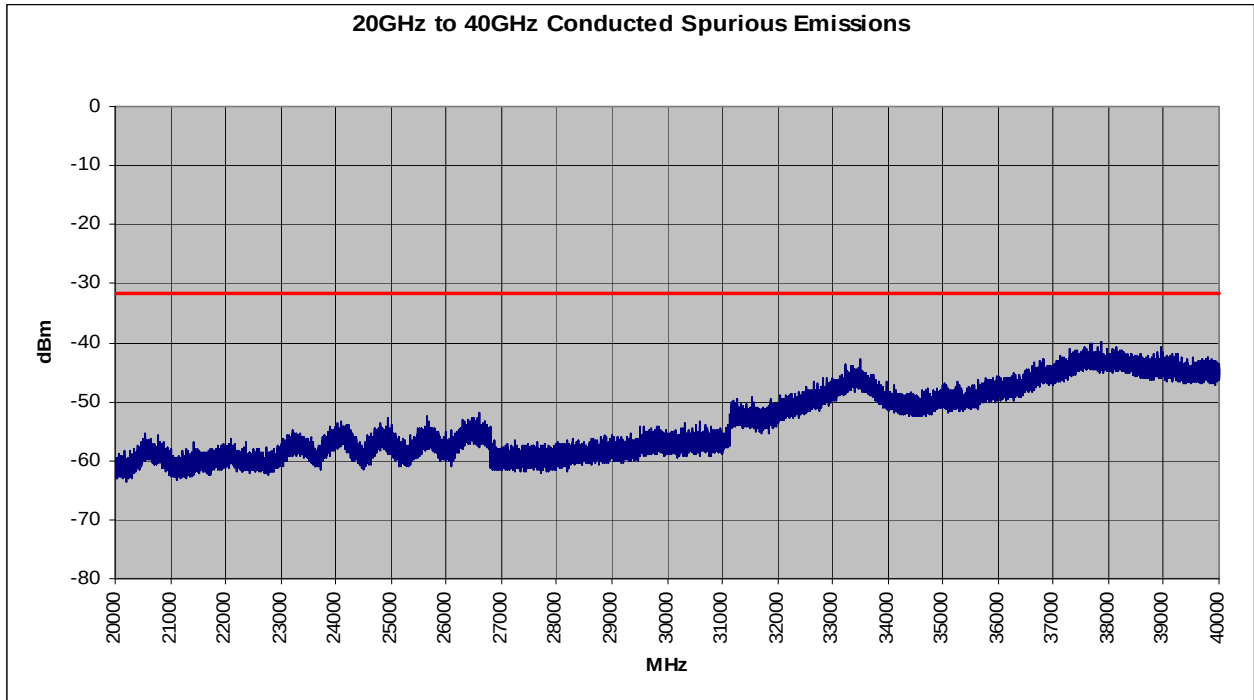
Plot 6-54. Conducted Spurious Plot (802.11a – Ch. 149)
