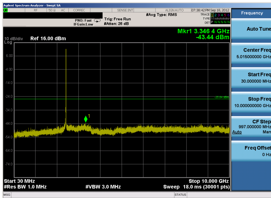
Plot 6-49. Conducted Spurious Plot (802.11b – Ch. 6)
