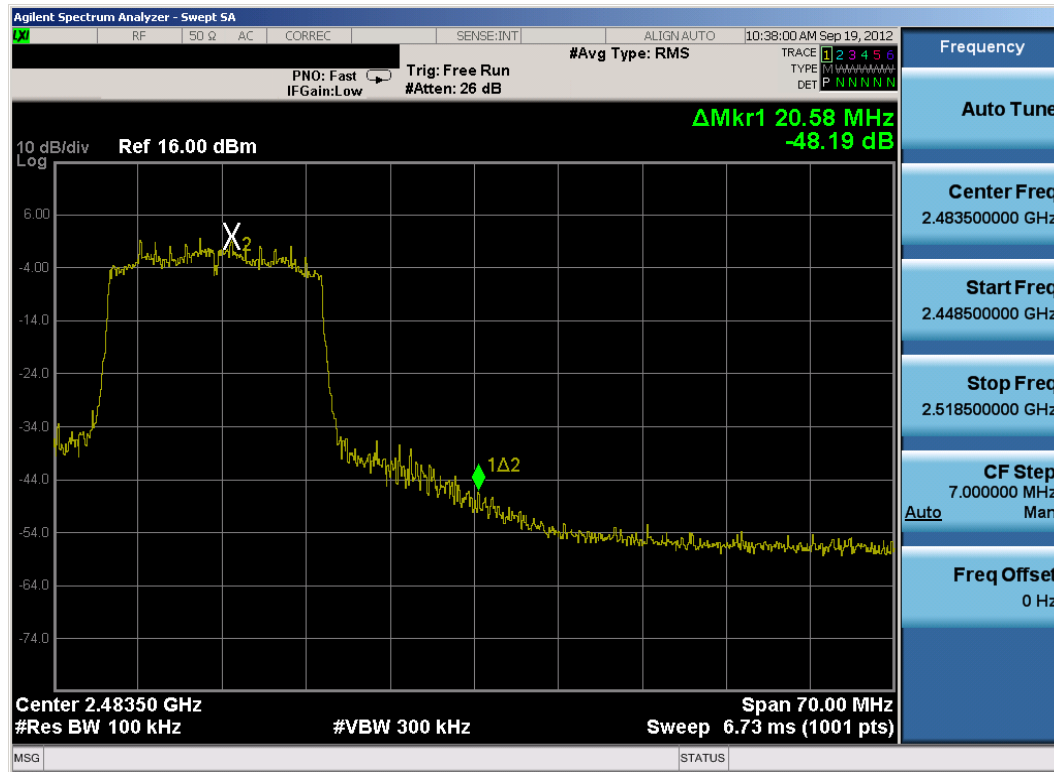
Plot 6-40. Band Edge Plot (802.11n (2.4GHz) – Ch. 11)
