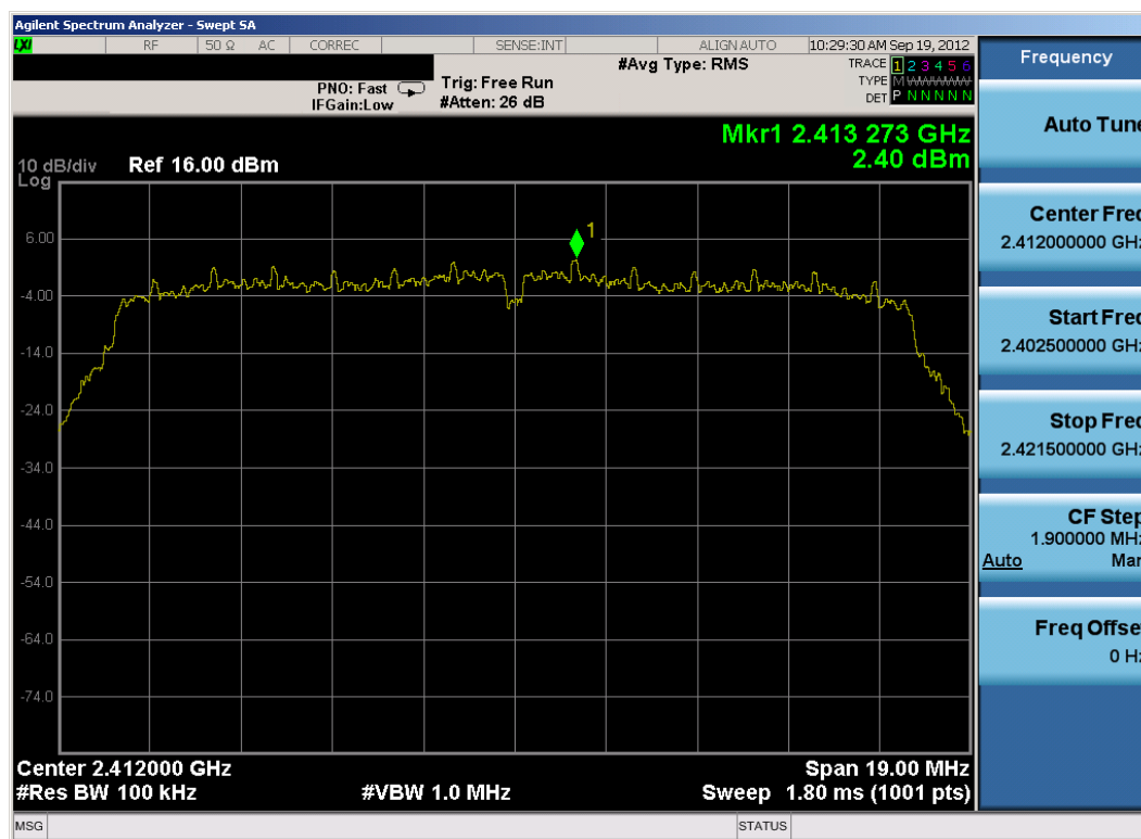
Plot 6-21. Power Spectral Density Plot (802.11g – Ch. 1)
