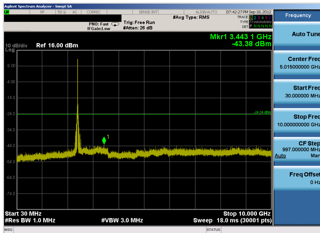
Plot 6-47. Conducted Spurious Plot (802.11b – Ch. 1)
