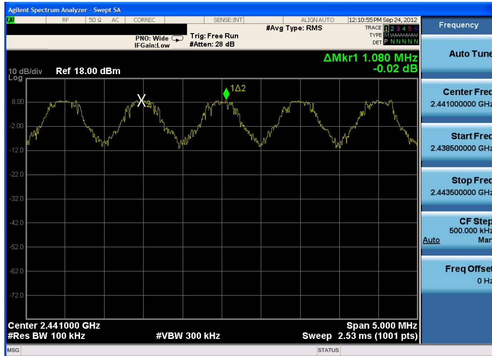
Plot 6-23. Channel Spacing Plot (Bluetooth)
