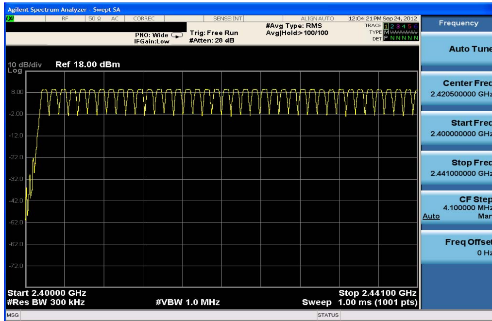
Plot 6-25. Low End Spectrum Channel Hopping Plot (Bluetooth)
