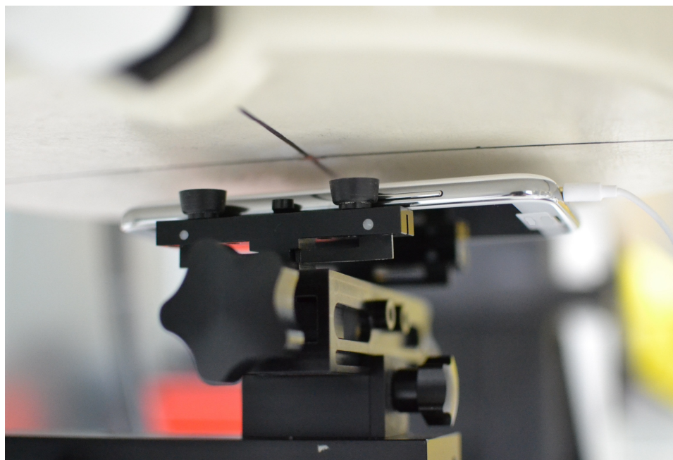
SAR Test Setup Photo 9 – Body-Worn Back Side at 1.0 cm
