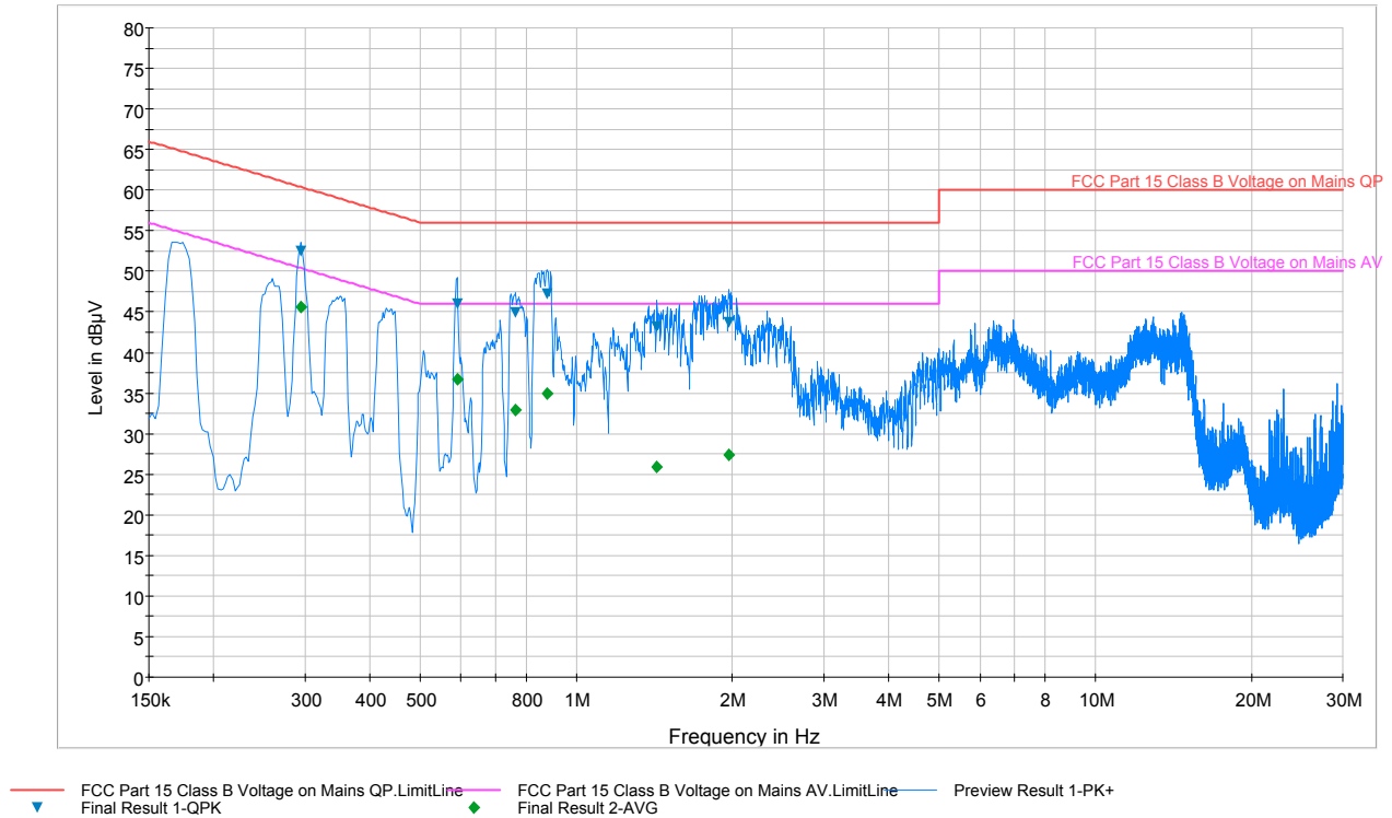
Plot 6-5. Line-Conducted Test Plot (L1)
