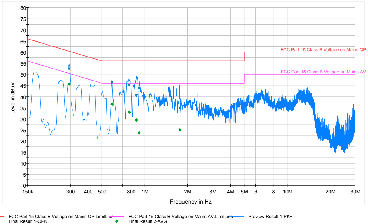
Plot 6-6. Line-Conducted Test Plot (N)
