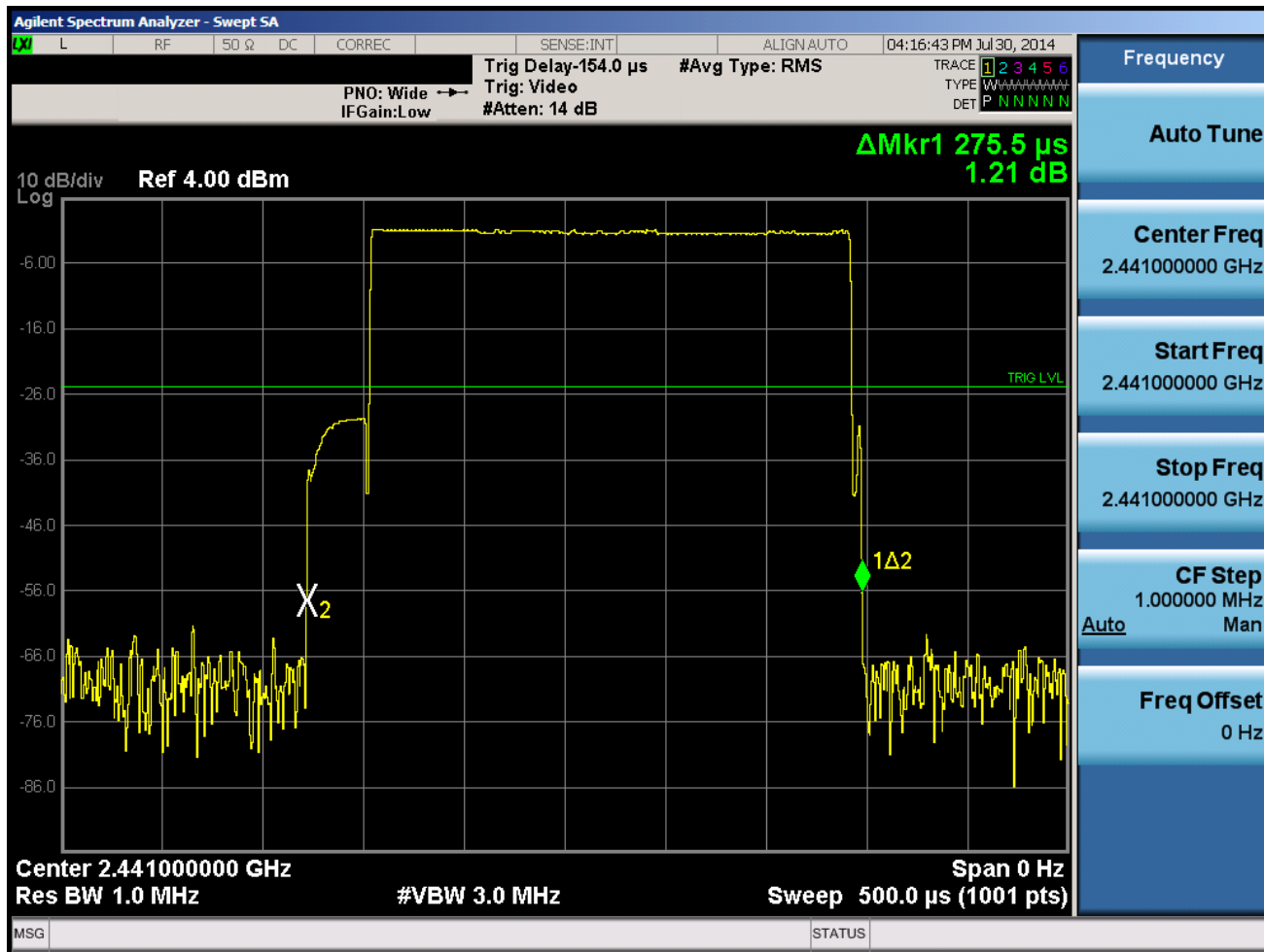
Plot 6-1. Pulse Width Measurement
