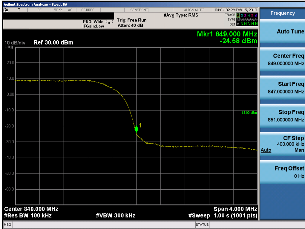
Plot 7-35. Band Edge Plot (Cellular WCDMA Mode – Ch. 4233)
