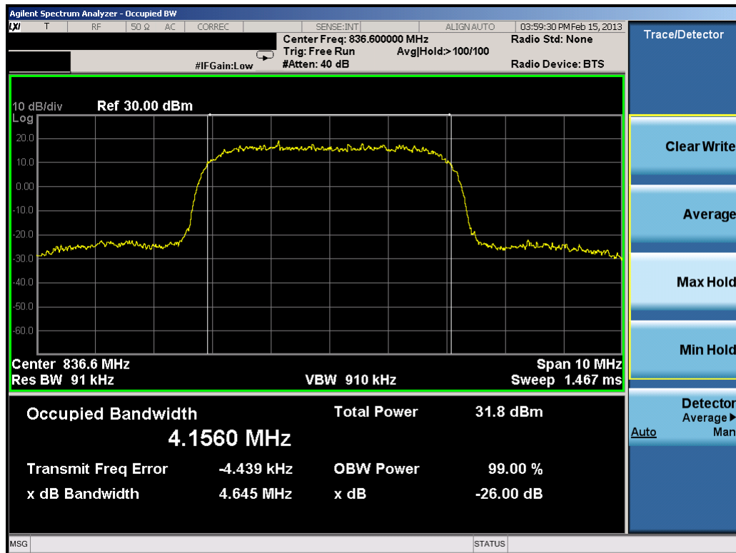
Plot 7-32. Occupied Bandwidth Plot (Cellular WCDMA Mode – Ch. 4183)
