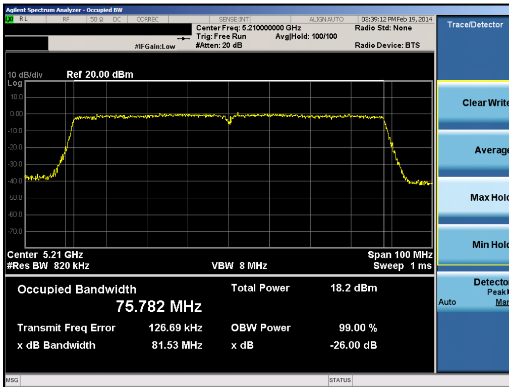
Plot 6-39. 26dB Bandwidth Plot (80MHz BW 802.11ac (UNII Band 1) – Ch. 42)
