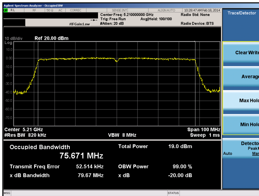
Plot 6-30. 20dB Bandwidth Plot (80MHz BW 802.11ac (UNII Band 1) – Ch. 42)
