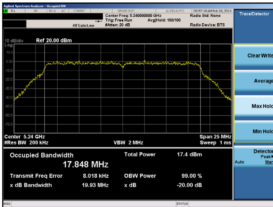
Plot 6-59. 20dB Bandwidth Plot (20MHz BW 802.11n (UNII Band 1) – Ch. 48)
