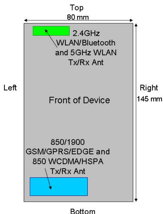
Figure 1-2 DUT Antenna Locations
