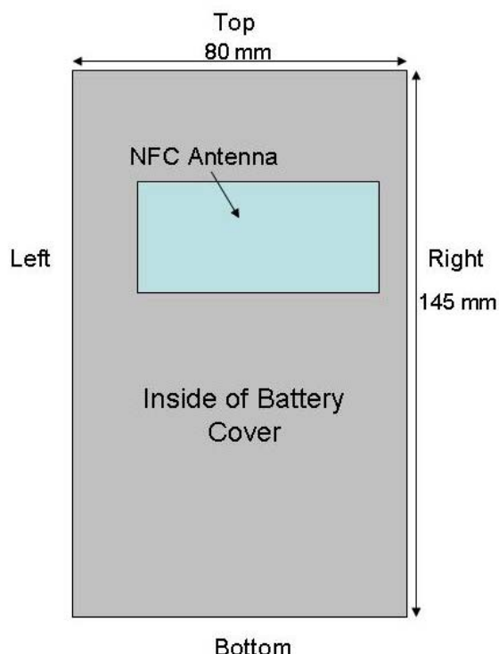
Figure 1-1 NFC Antenna Location
