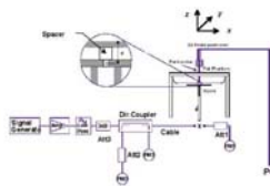
Figure 10-1 System Verification Setup Diagram
