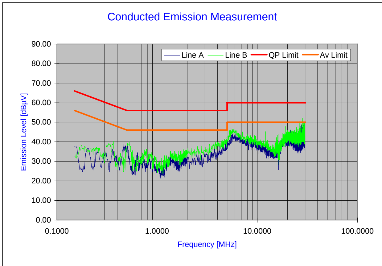
Plot 6-58. Line Conducted Plot with 802.11a
