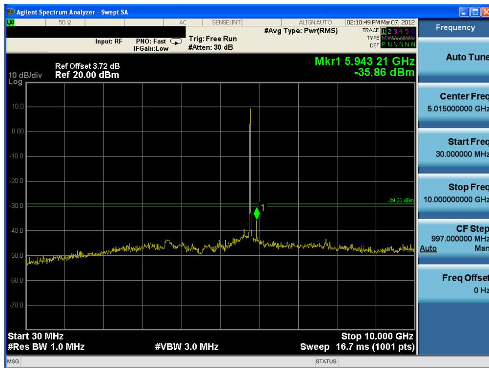
Plot 6-47. Conducted Spurious Plot (802.11a – Ch. 149)
