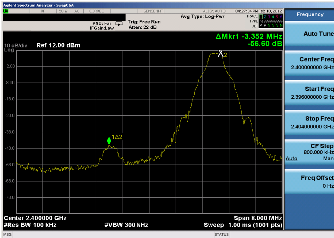
Plot 6-10. Band Edge Plot (Bluetooth with Hopping Disabled, 1Mbps – Ch. 0)
