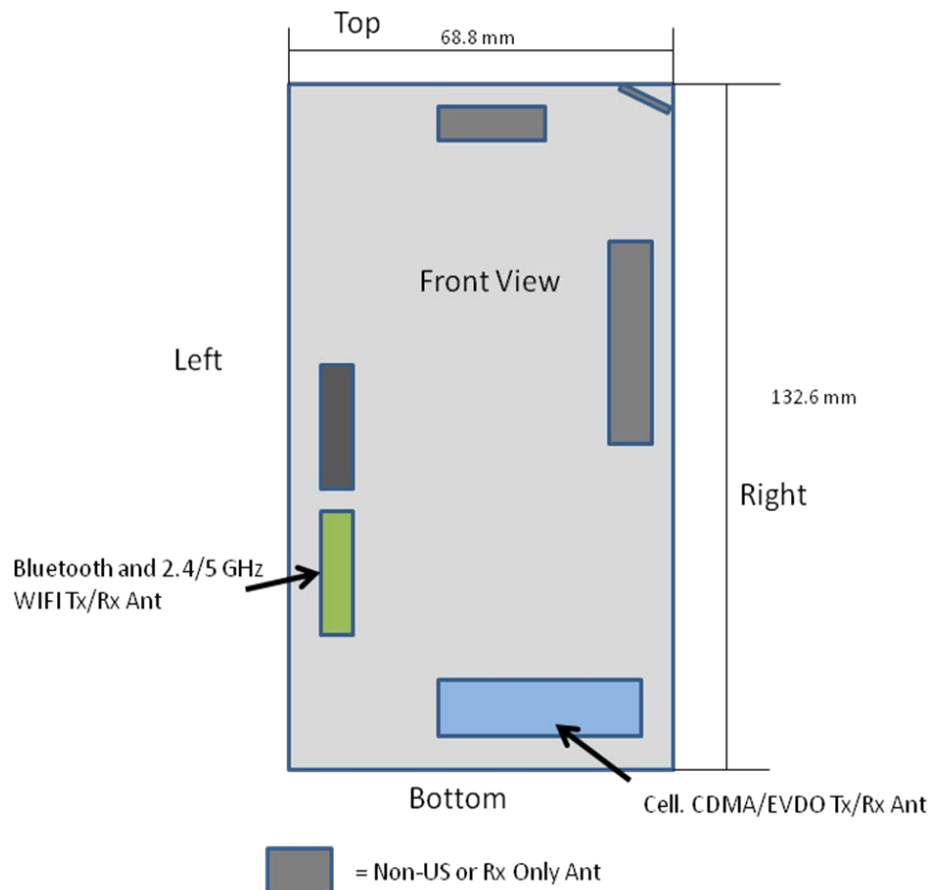
Figure 13-1 Identification of Sides for SAR Testing
