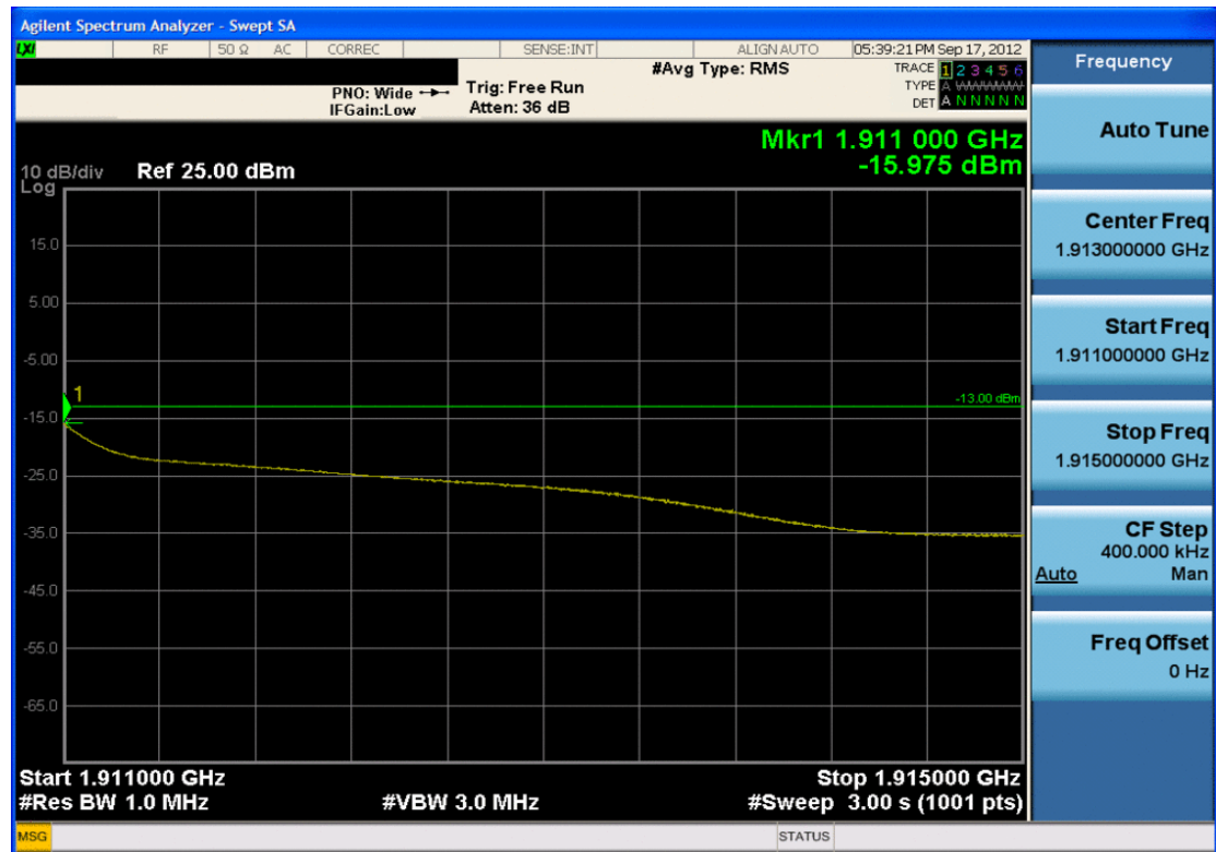
Plot 7-46. 4MHz Span Plot (PCS WCDMA Mode – Ch. 9538)
