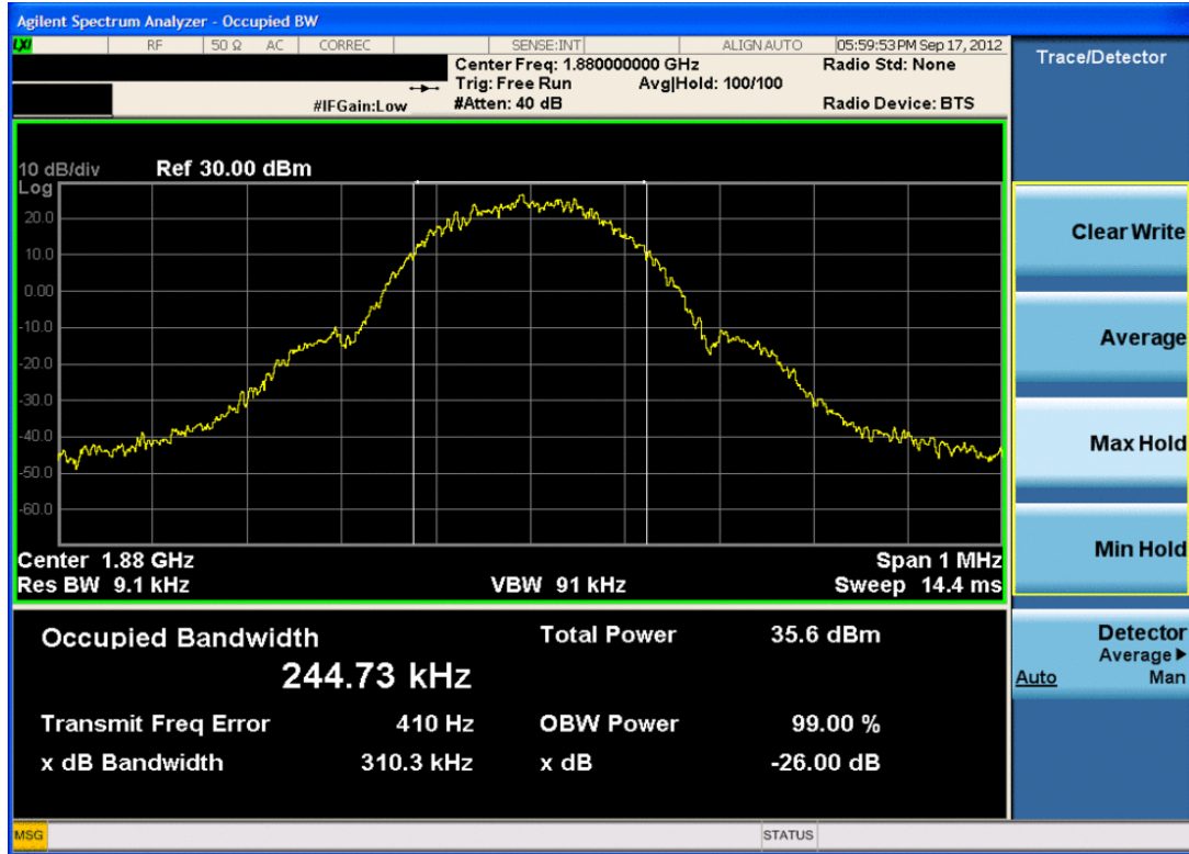
Plot 7-17. Occupied Bandwidth Plot (PCS GSM Mode – Ch. 661)
