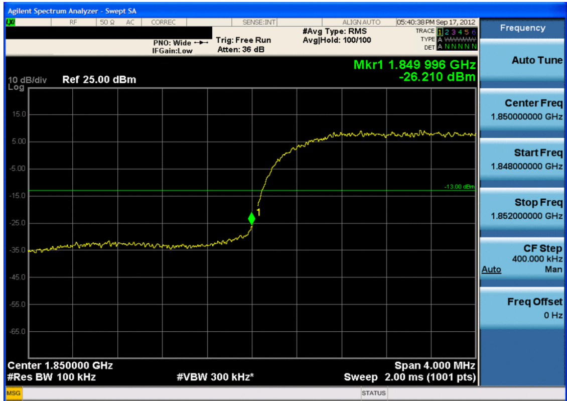
Plot 7-37. Band Edge Plot (PCS WCDMA Mode – Ch. 9262)
