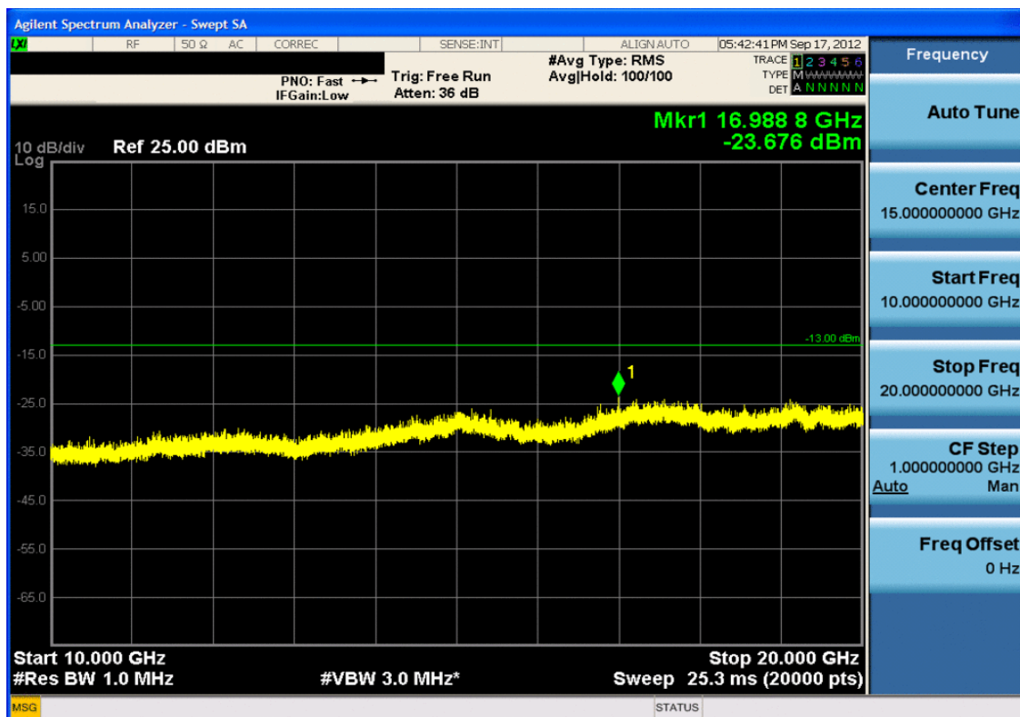
Plot 7-36. Conducted Spurious Plot (PCS WCDMA Mode – Ch. 9262)
