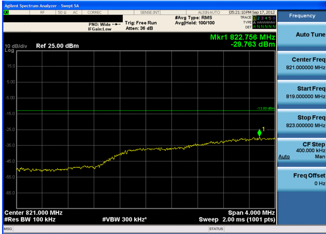
Plot 7-27. 4MHz Span Plot (Cellular WCDMA Mode – Ch. 4132)
