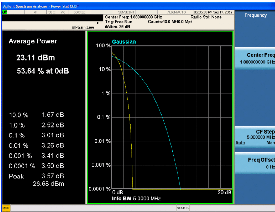
Plot 7-42. Peak-Average Ratio Plot (PCS WCDMA Mode – Ch. 9400)
