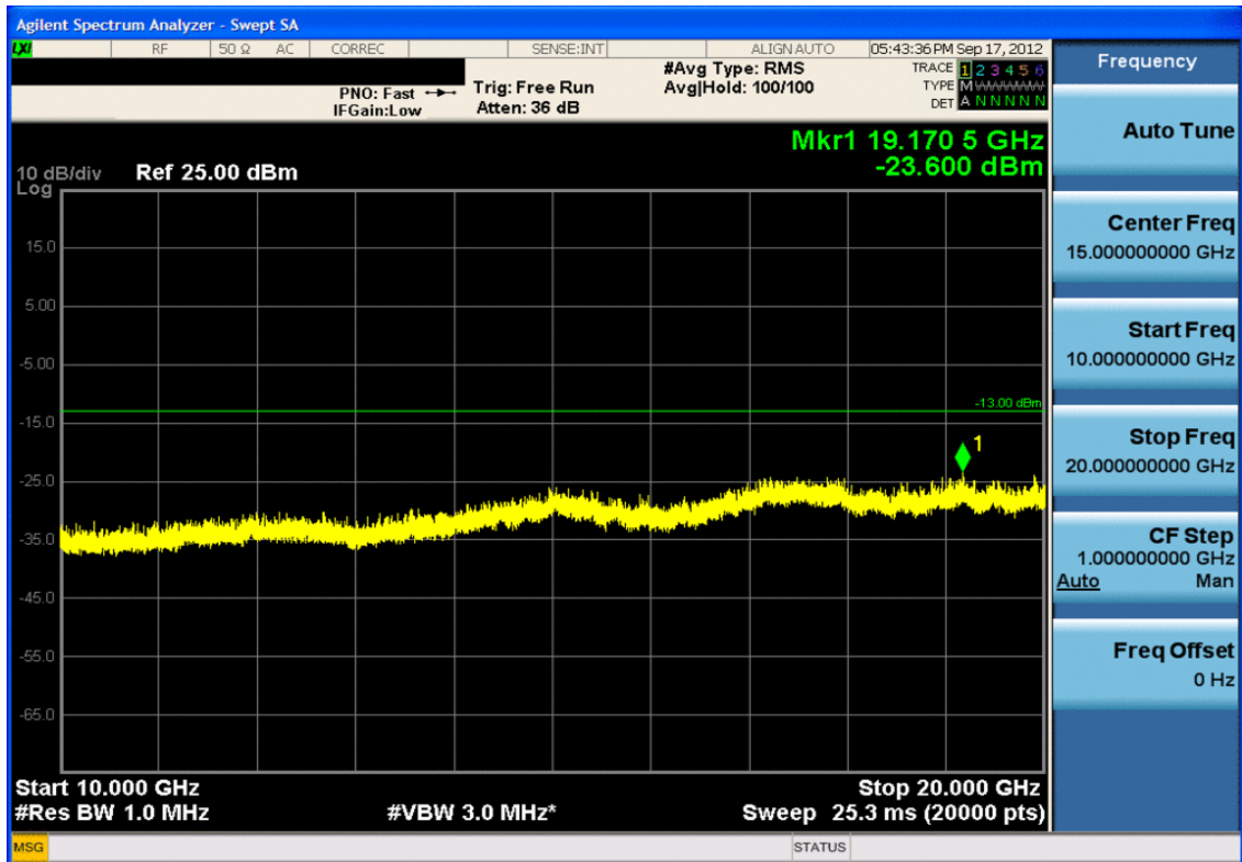
Plot 7-40. Conducted Spurious Plot (PCS WCDMA Mode – Ch. 9400)
