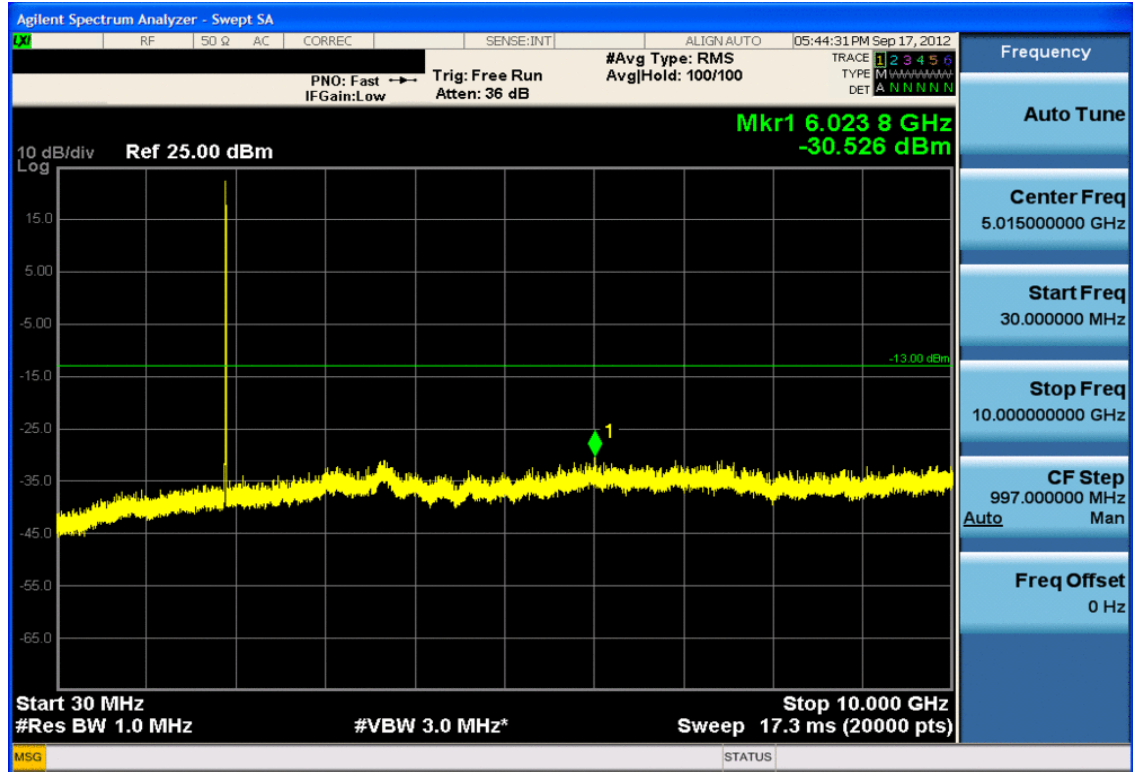
Plot 7-43. Conducted Spurious Plot (PCS WCDMA Mode – Ch. 9538)
