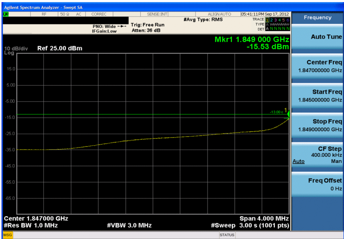
Plot 7-38. 4MHz Span Plot (PCS WCDMA Mode – Ch. 9262)
