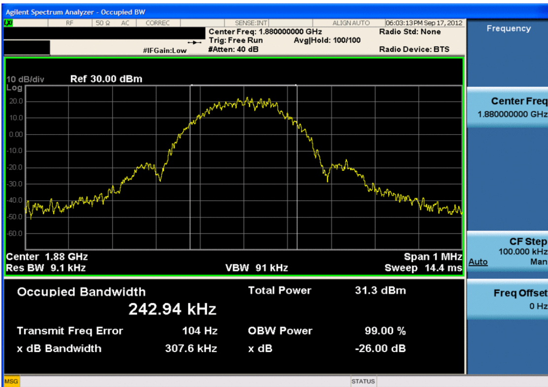
Plot 7-22. Occupied Bandwidth Plot (EDGE1900 Mode – Ch. 661)
