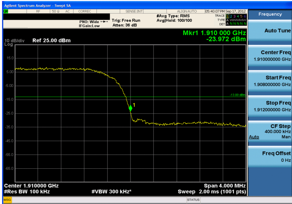
Plot 7-45. Band Edge Plot (PCS WCDMA Mode – Ch. 9538)
