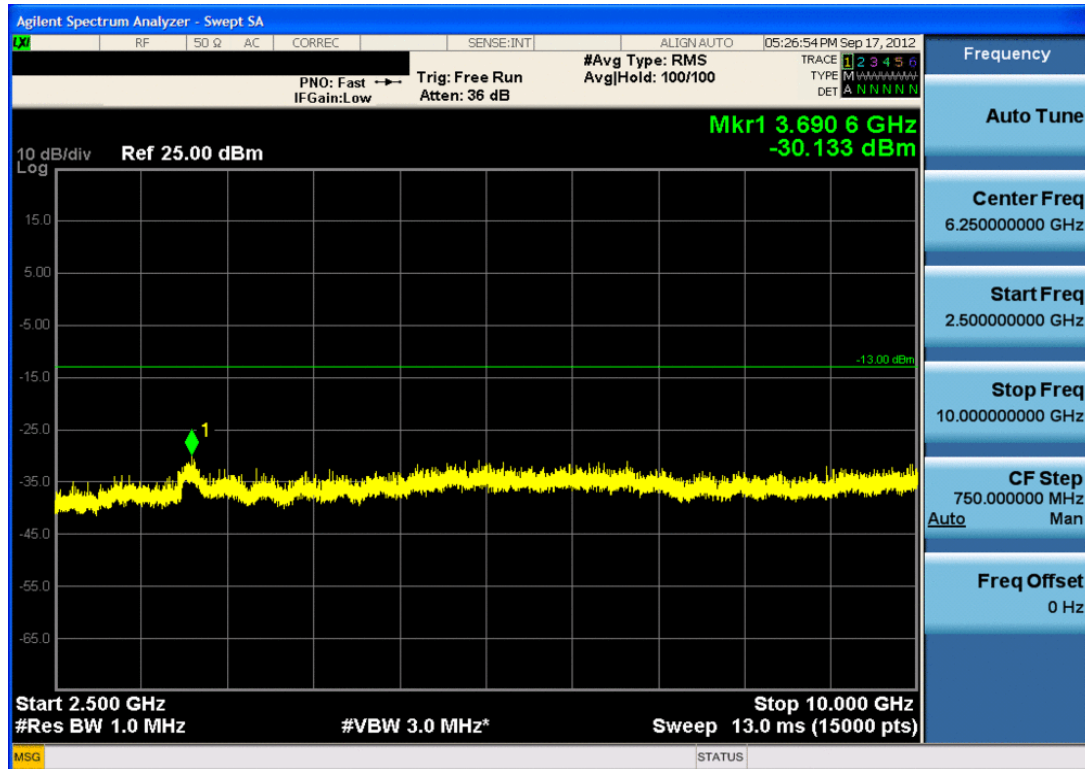
Plot 7-29. Conducted Spurious Plot (Cellular WCDMA Mode – Ch. 4183)
