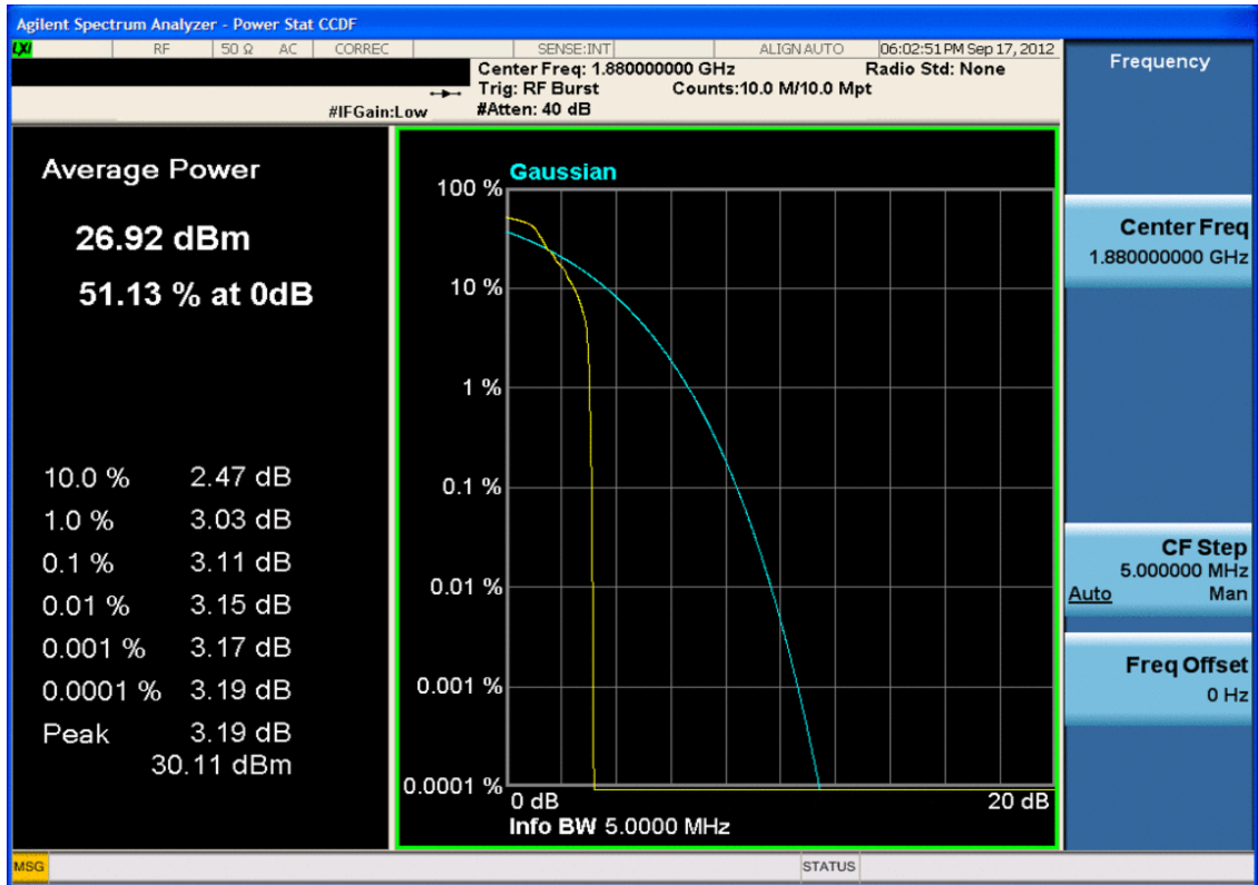
Plot 7-23. Peak-Average Ratio Plot (EDGE1900 Mode – Ch. 661)
