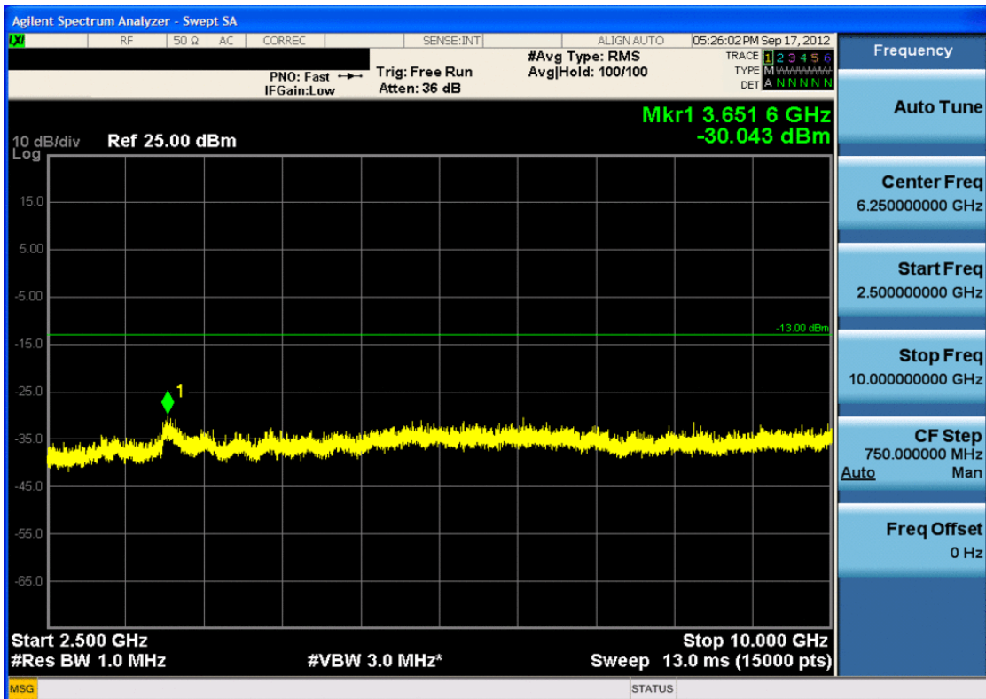
Plot 7-32. Conducted Spurious Plot (Cellular WCDMA Mode – Ch. 4233)
