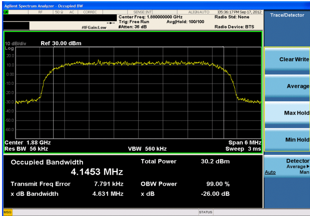
Plot 7-41. Occupied Bandwidth Plot (PCS WCDMA Mode – Ch. 9400)
