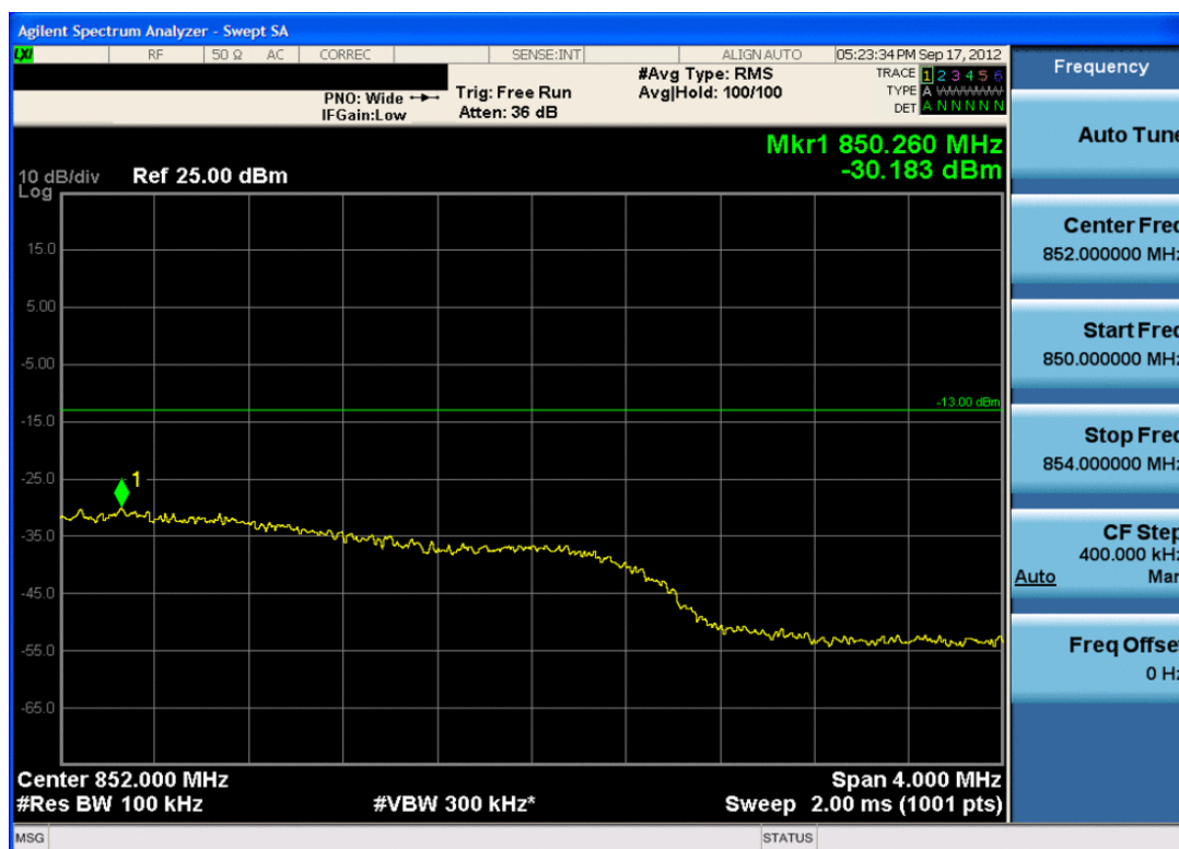
Plot 7-34. 4MHz Span Plot (Cellular WCDMA Mode – Ch. 4233)
