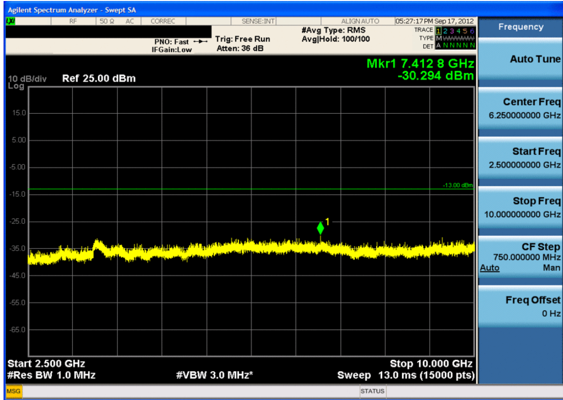
Plot 7-25. Conducted Spurious Plot (Cellular WCDMA Mode – Ch. 4132)
