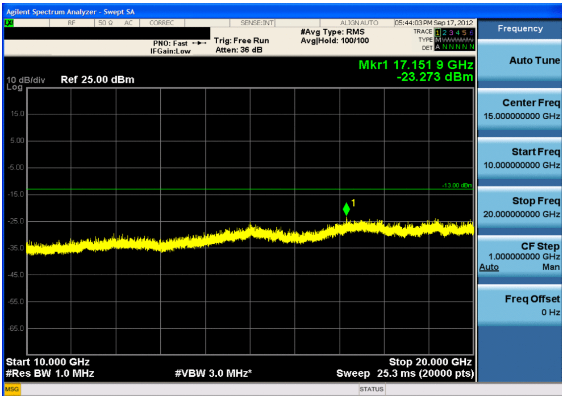
Plot 7-44. Conducted Spurious Plot (PCS WCDMA Mode – Ch. 9538)
