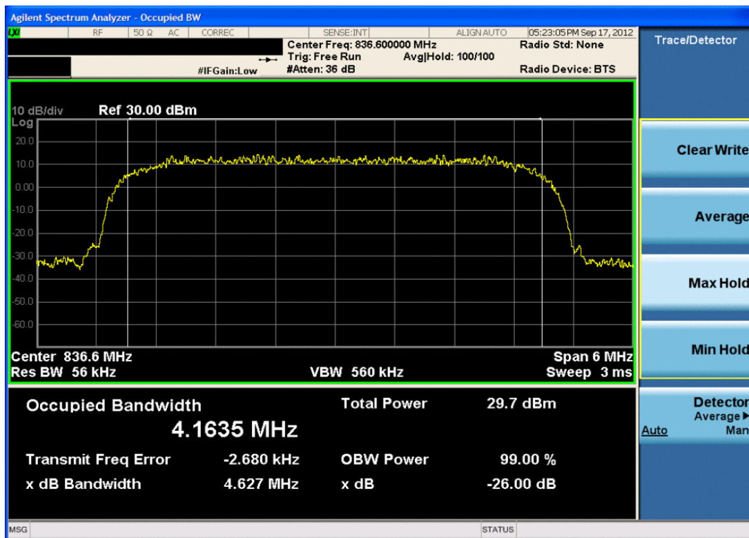
Plot 7-30. Occupied Bandwidth Plot (Cellular WCDMA Mode – Ch. 4183)
