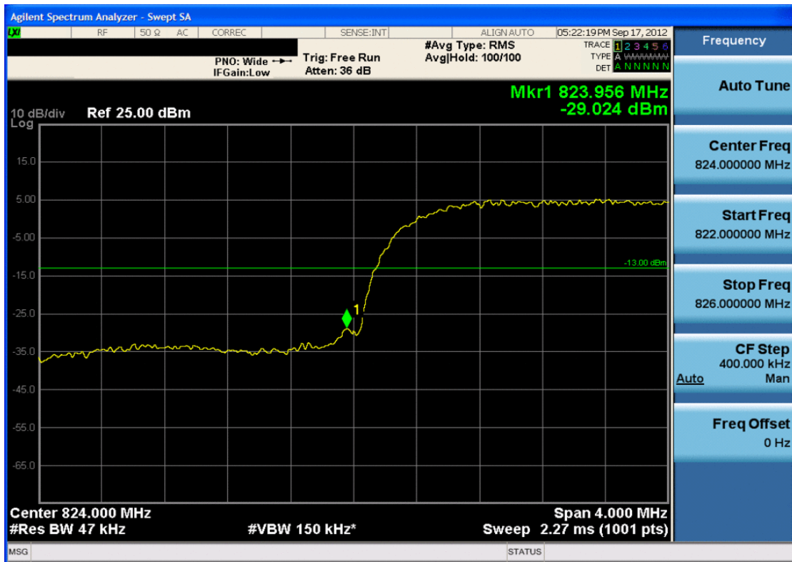
Plot 7-26. Band Edge Plot (Cellular WCDMA Mode – Ch. 4132)
