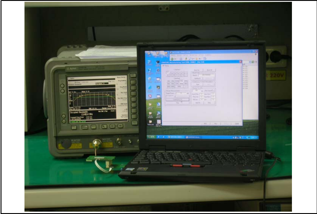
[ 6dB Bandwidth Measurement ]
