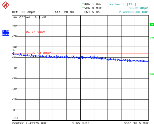
Highest Channel(2 462 MHz): Peak
