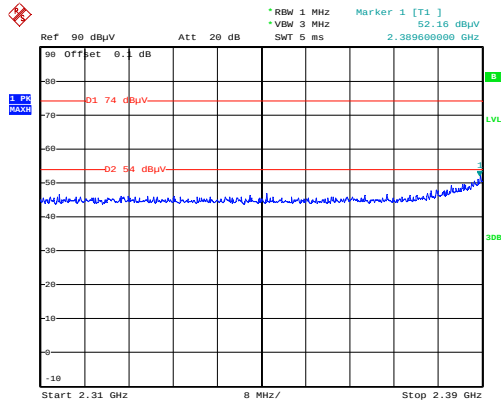
Lowest Channel(2 412 MHz): Peak
