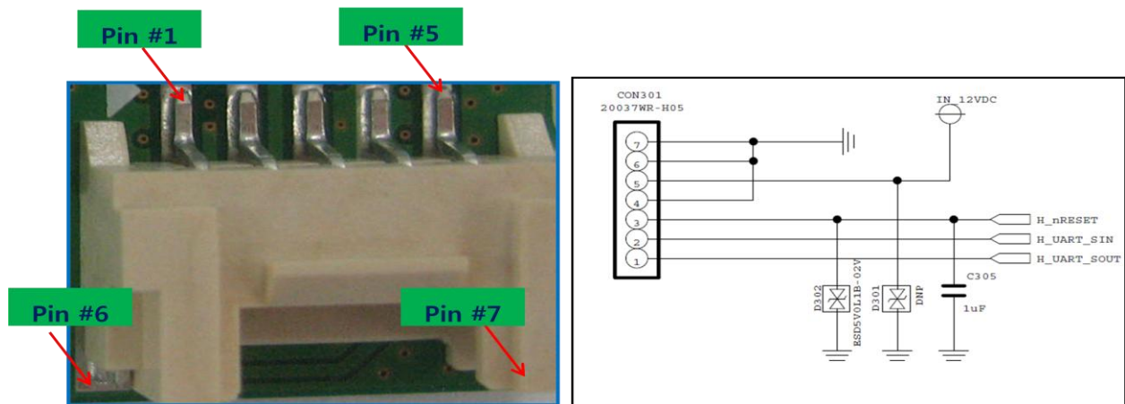
Figure 2-3 UART Pin Assignments (Top View)
