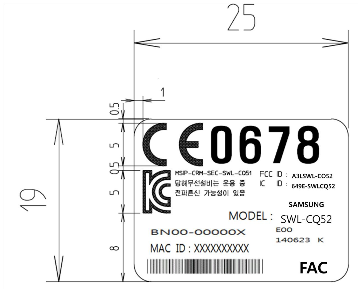
Figure 5-1. Product Label
