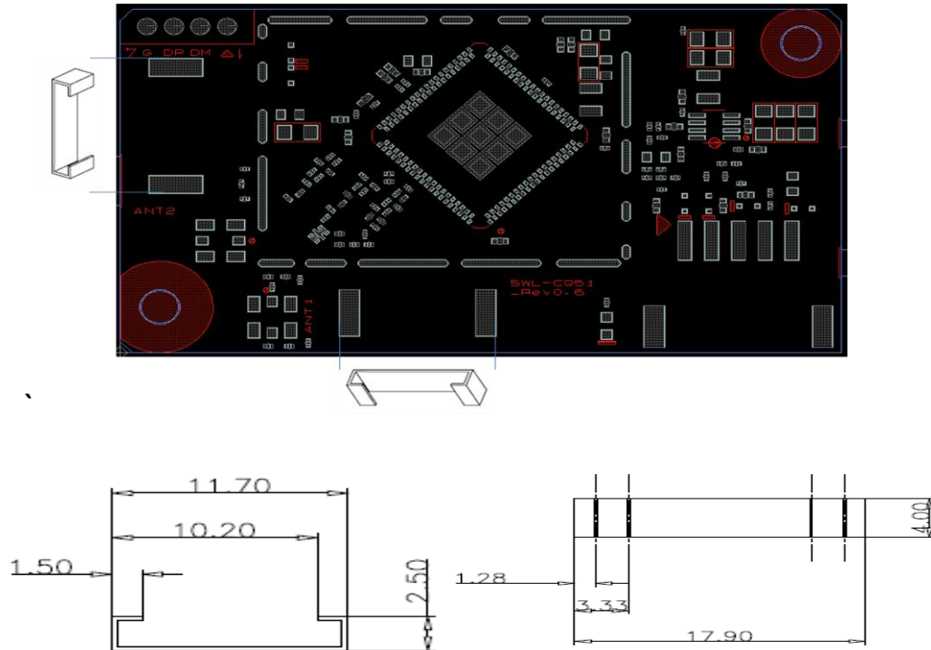
Figure 2-2 Antenna Mechanical Dimension
