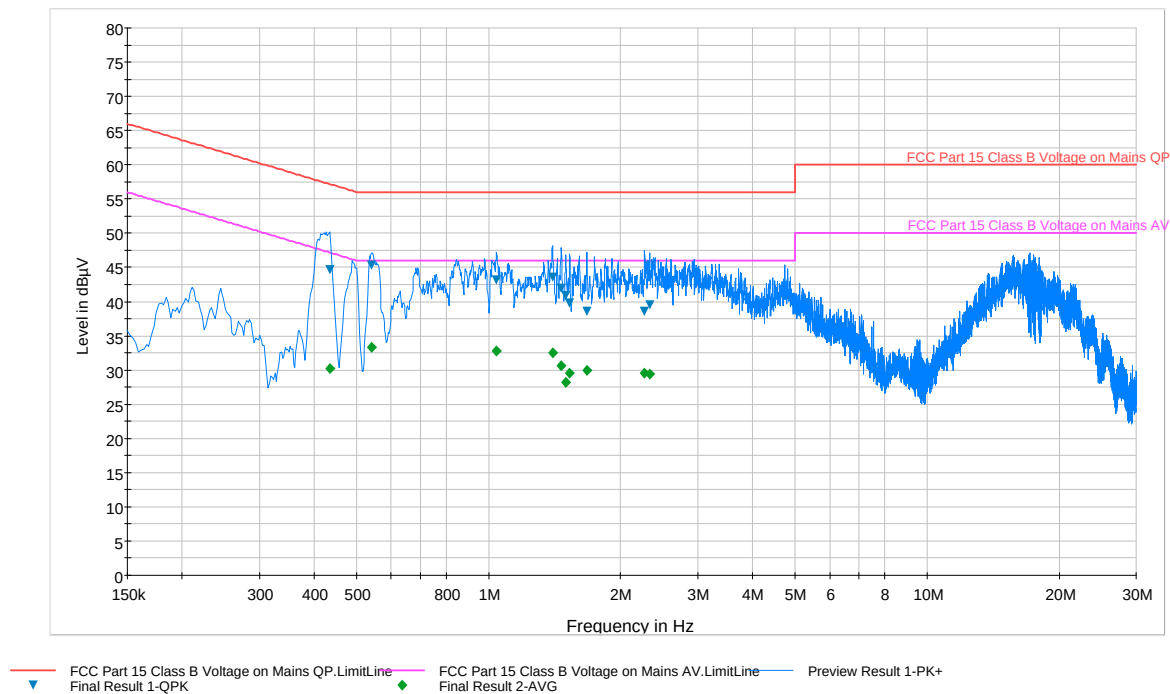
Plot 6-24. Line Conducted Plot with Bluetooth (L1)
