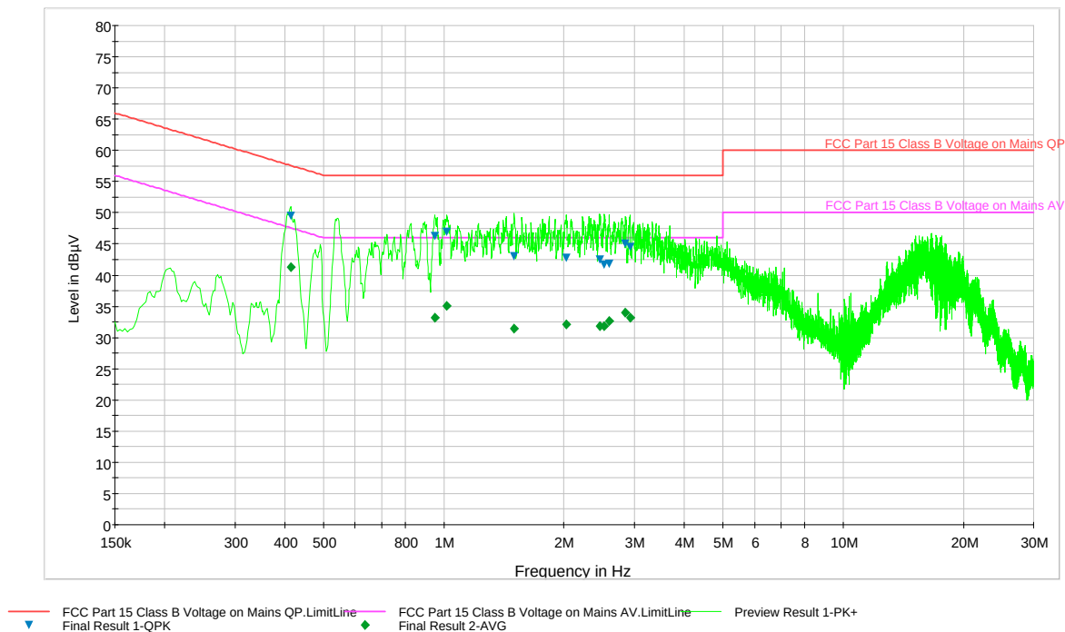
Plot 6-25. Line Conducted Plot with Bluetooth (LN)
