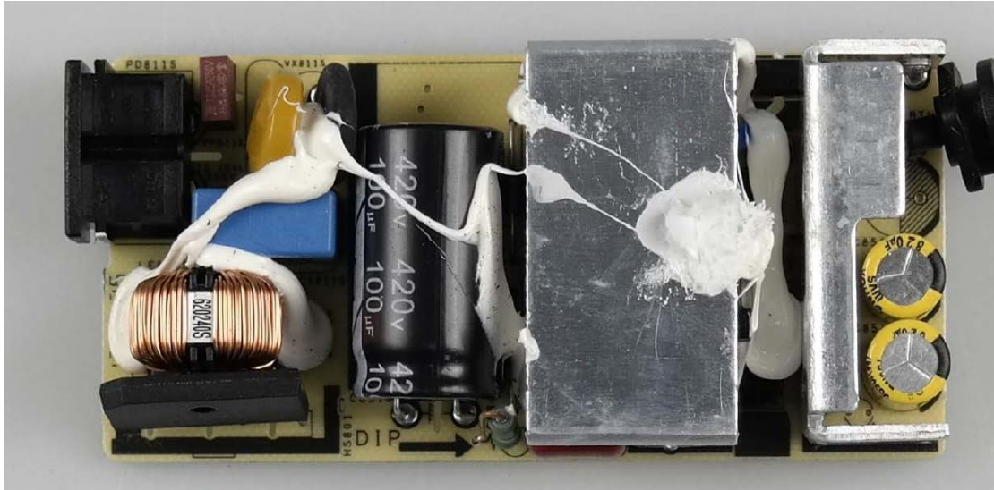
Before change A3514_ESM internal rear view
