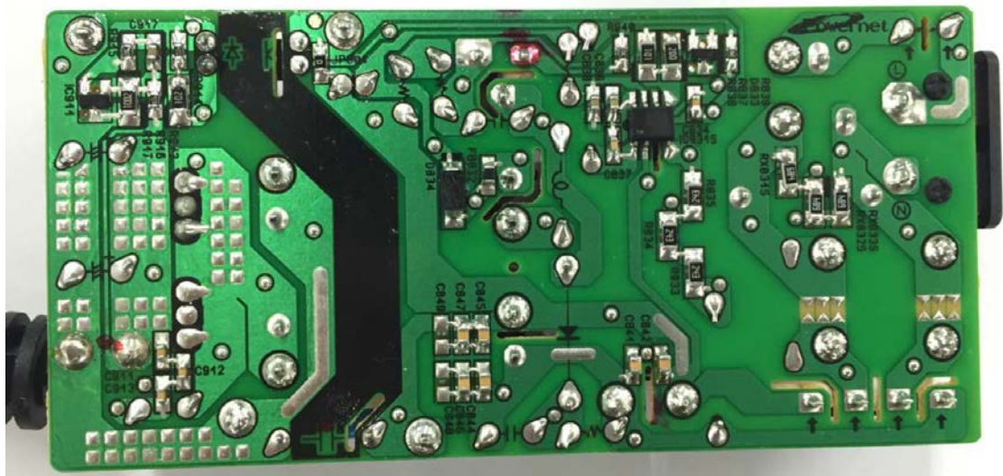
Back change A4514_FPN internal rear view
