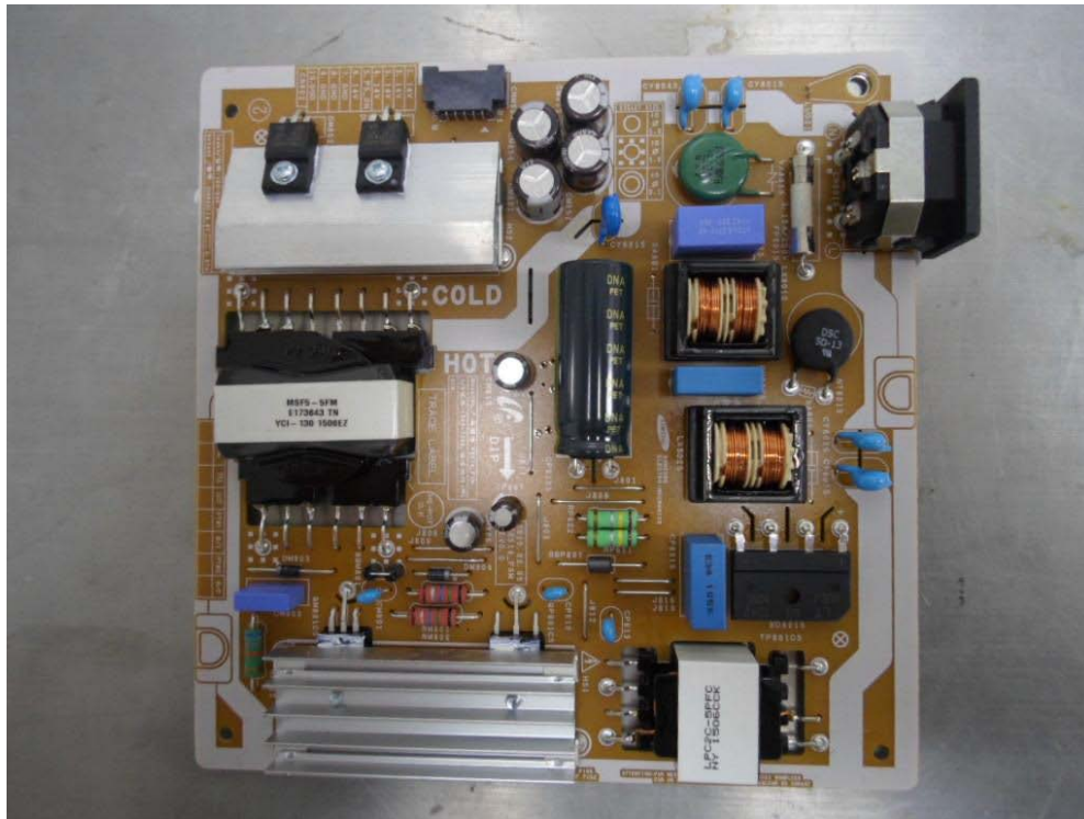
Before change P8514_FSM rear view
