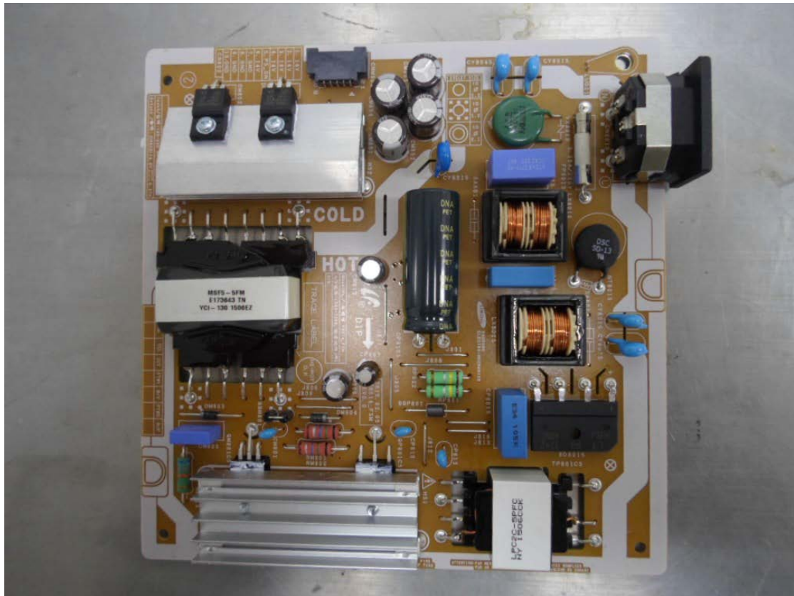
Back change L85S7N_FDY front view
