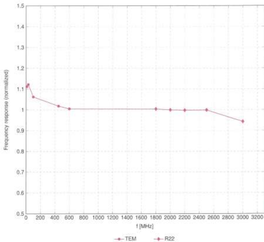
Frequency Response of E-Field (TEM-Cell:ifl110 EXX, Waveguide:R22)
