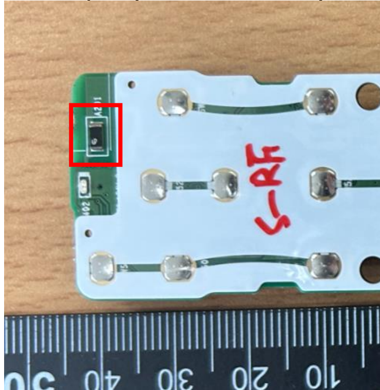
Chip ANT(ACA-3216-A1-CC-S-W1)
