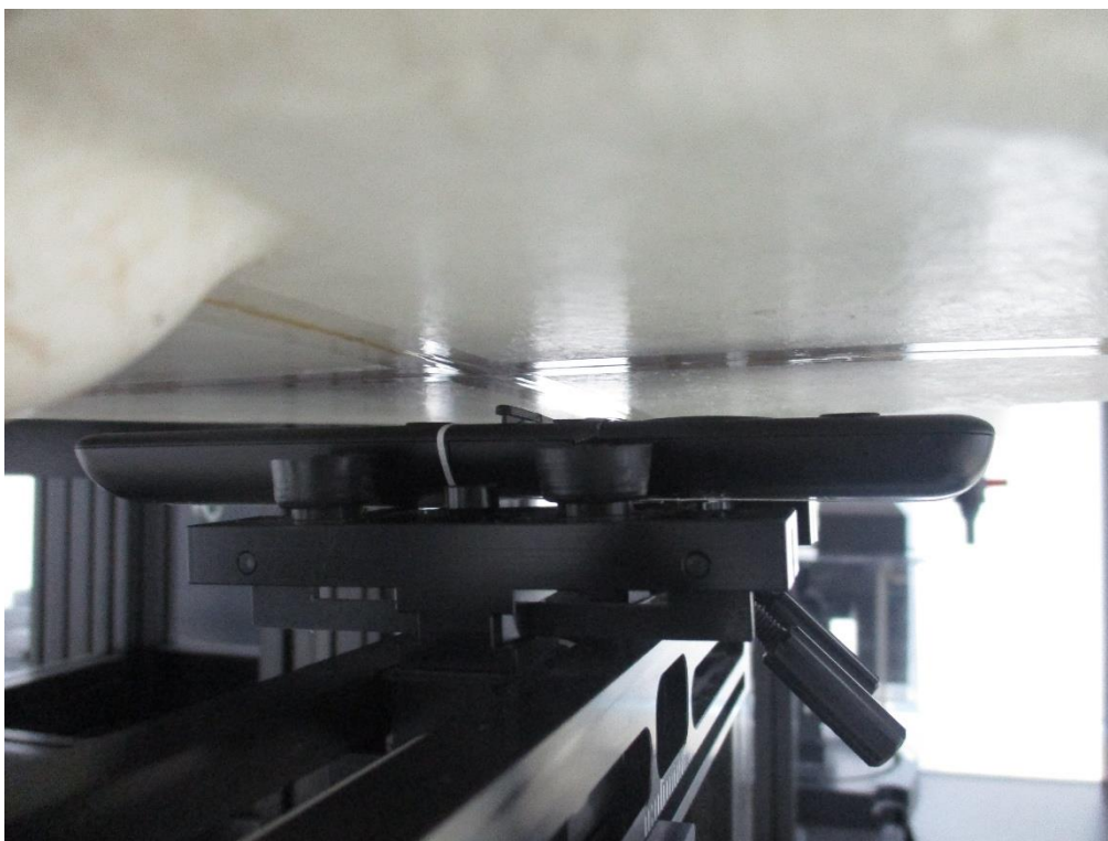
Front from Flat Phantom (Separation Distance: 1.0 cm)
