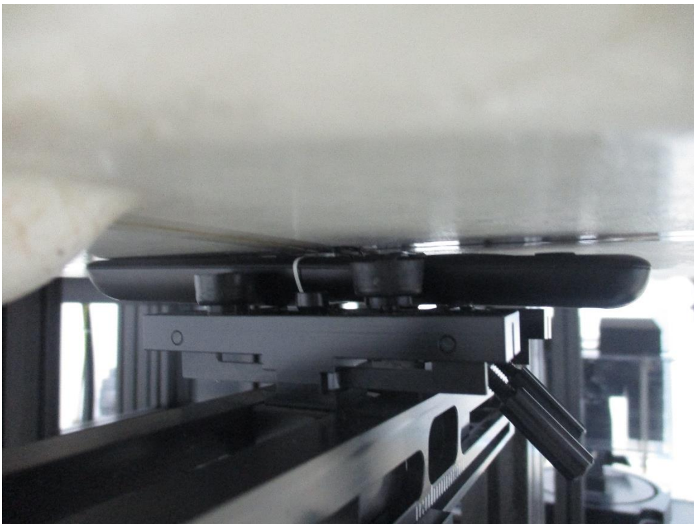
Front#2 from Flat Phantom (Separation Distance: 0 cm)
