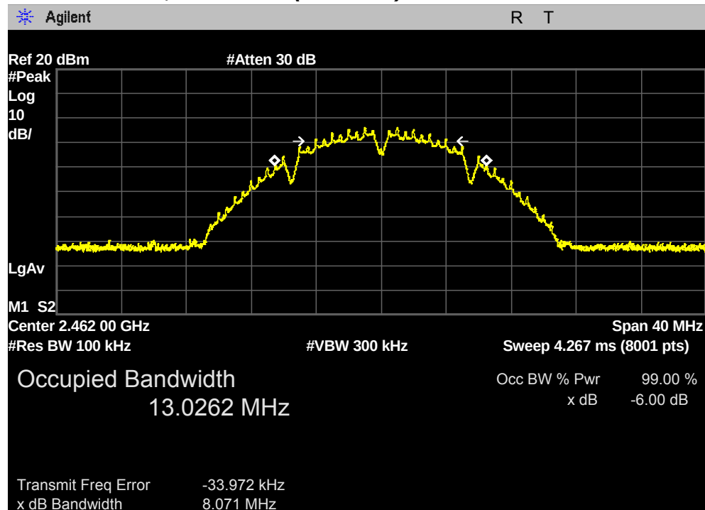
6 dB Bandwidth, 11 Channel (2462 MHz)
