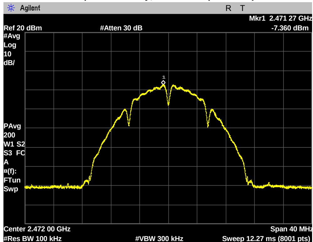
Maximum Power Spectral Density, 13 Channel (2472 MHz)
