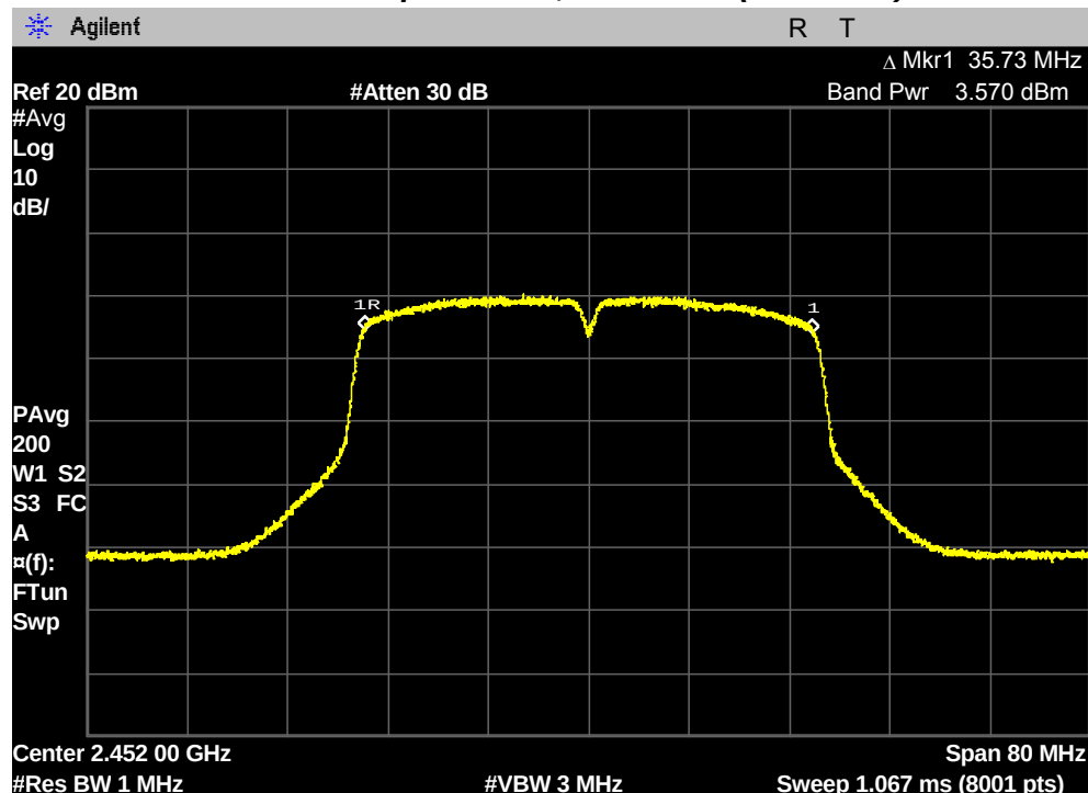
Maximum Conducted Output Power, 9 Channel (2452 MHz)
