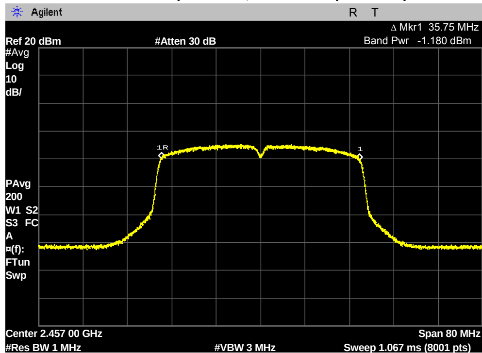
Maximum Conducted Output Power, 10 Channel (2457 MHz)
