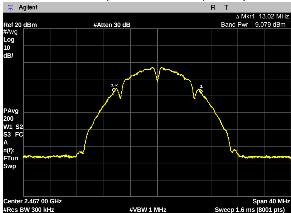
Maximum Conducted Output Power, 12 Channel (2467 MHz)
