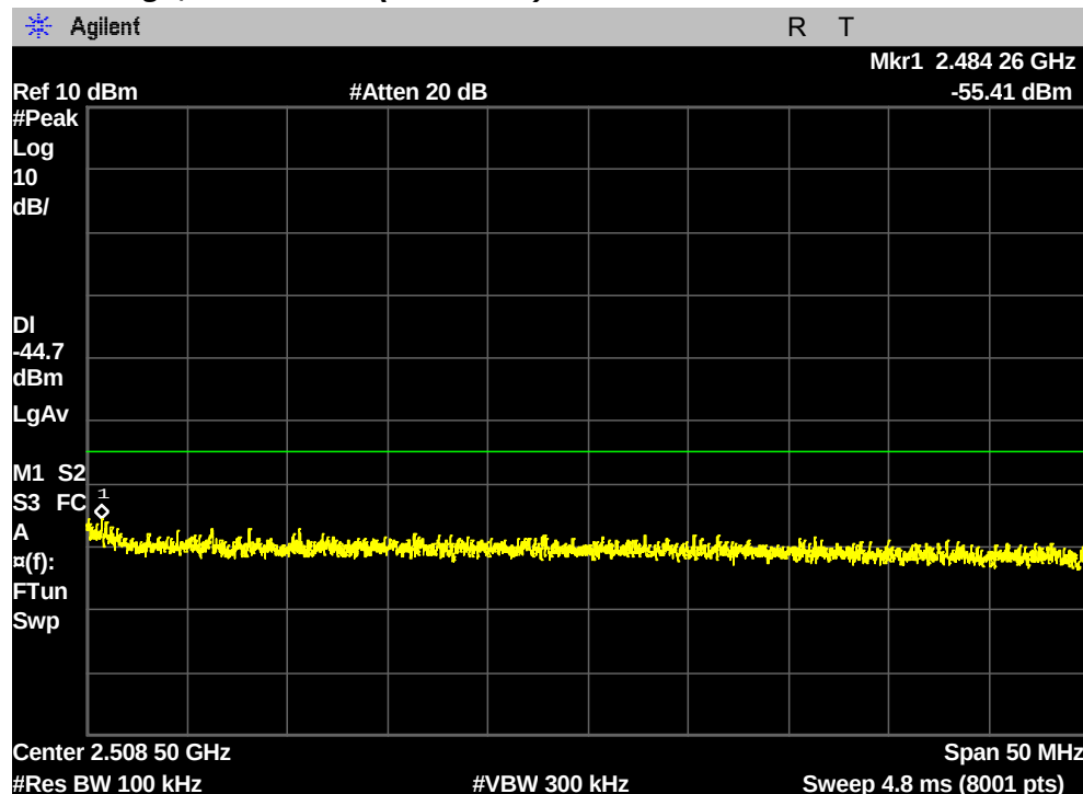
Band Edge, 10 Channel (2457 MHz)
