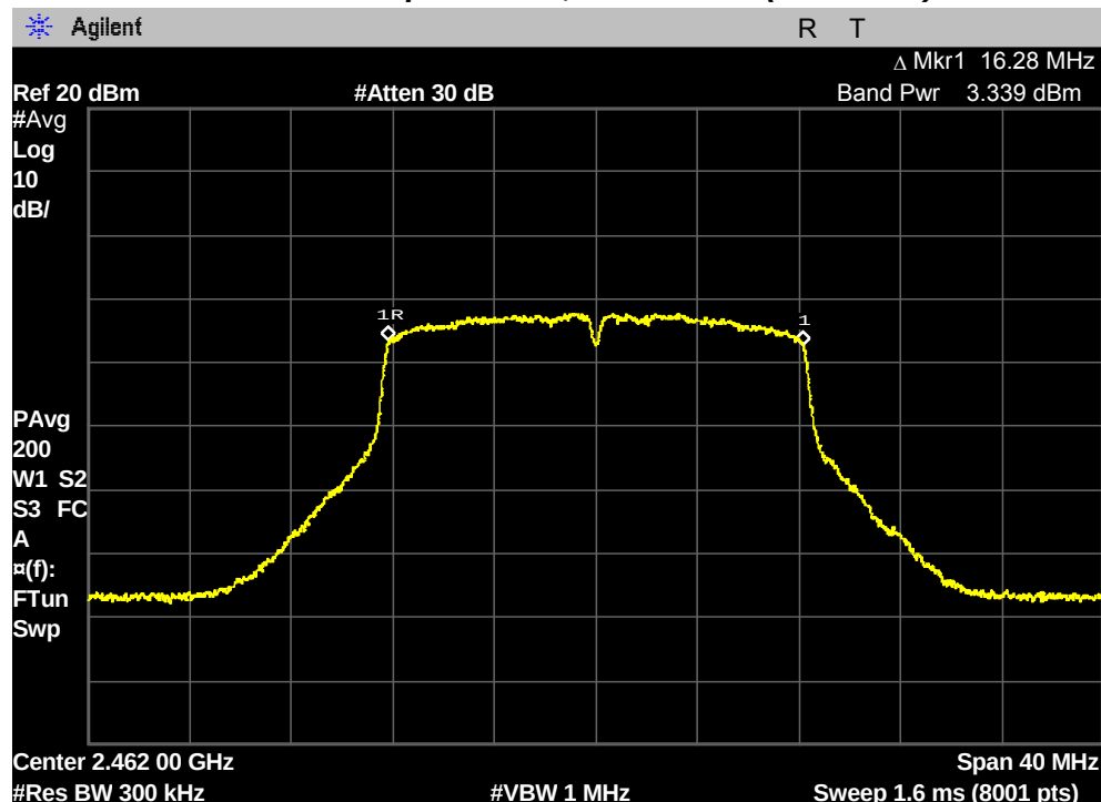
Maximum Conducted Output Power, 11 Channel (2462 MHz)
