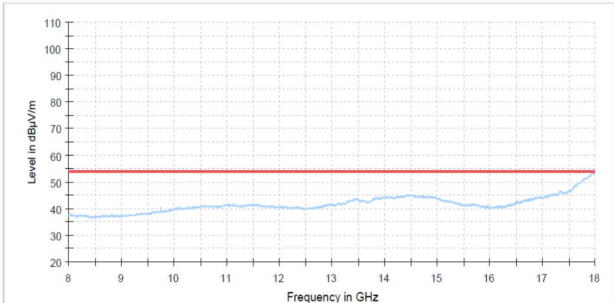
6 channel : 8 GHz to 18 GHz_Average
