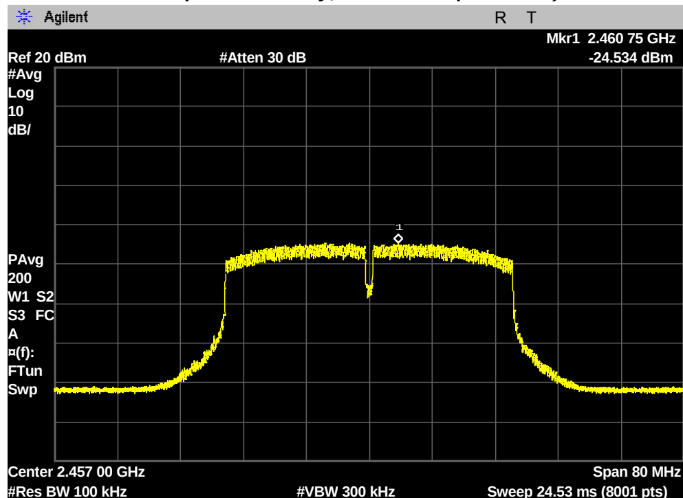
Maximum Power Spectral Density, 10 Channel (2457 MHz)
