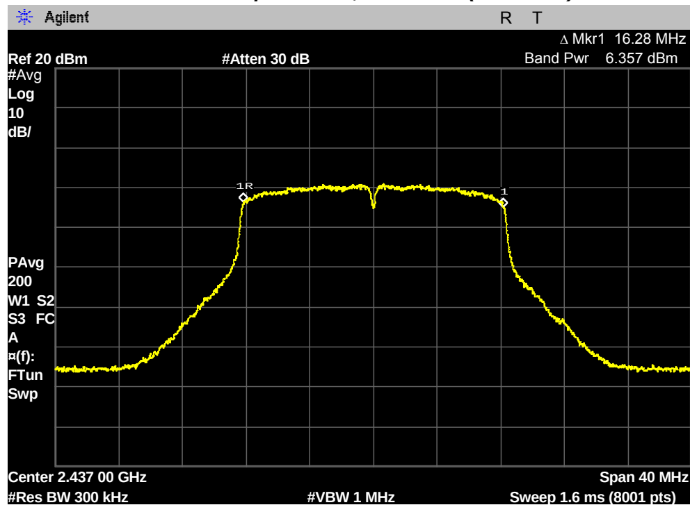
Maximum Conducted Output Power, 6 Channel (2437 MHz)
