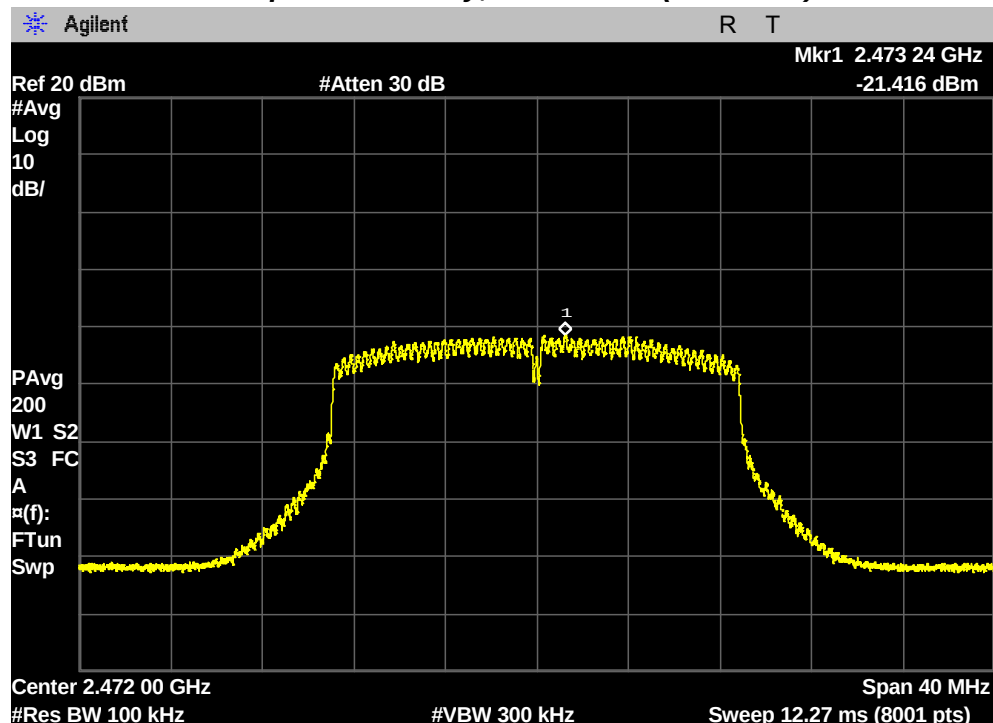
Maximum Power Spectral Density, 13 Channel (2472 MHz)
