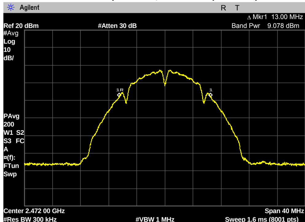
Maximum Conducted Output Power, 13 Channel (2472 MHz)
