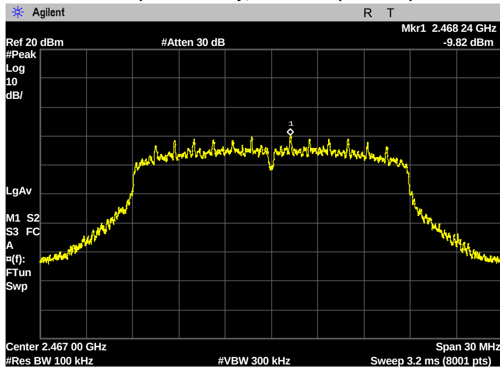
Reference Power Spectral Density, 12 Channel (2467 MHz)
