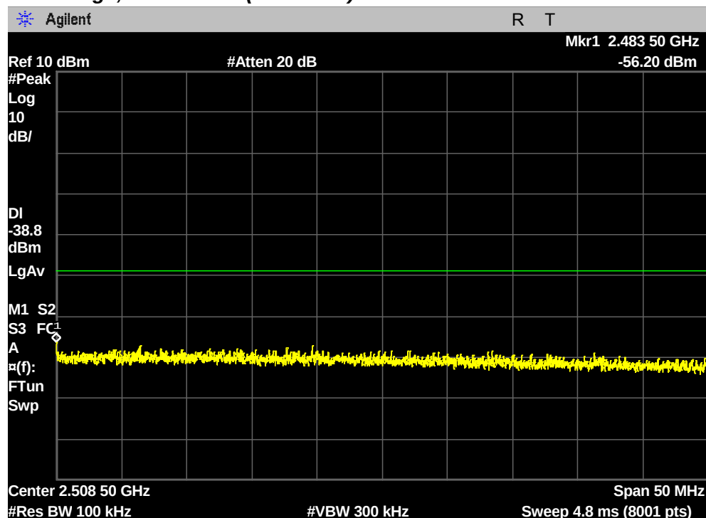
Band Edge, 12 Channel (2467 MHz)
