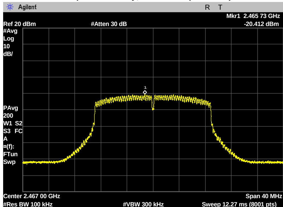
Maximum Power Spectral Density, 12 Channel (2467 MHz)
