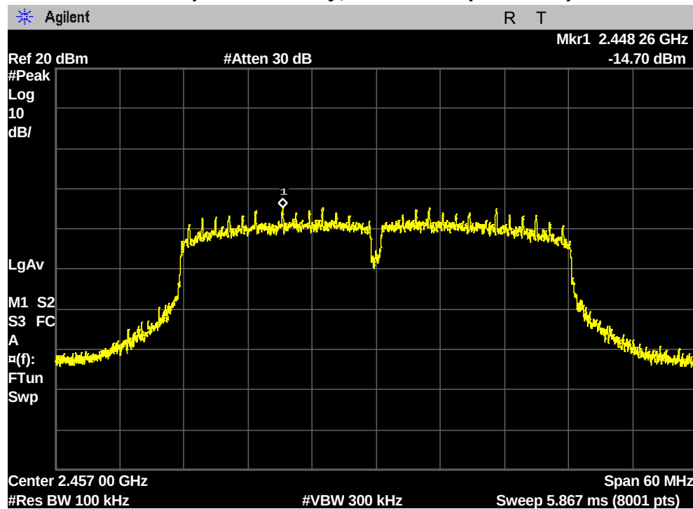
Reference Power Spectral Density, 10 Channel (2457 MHz)
