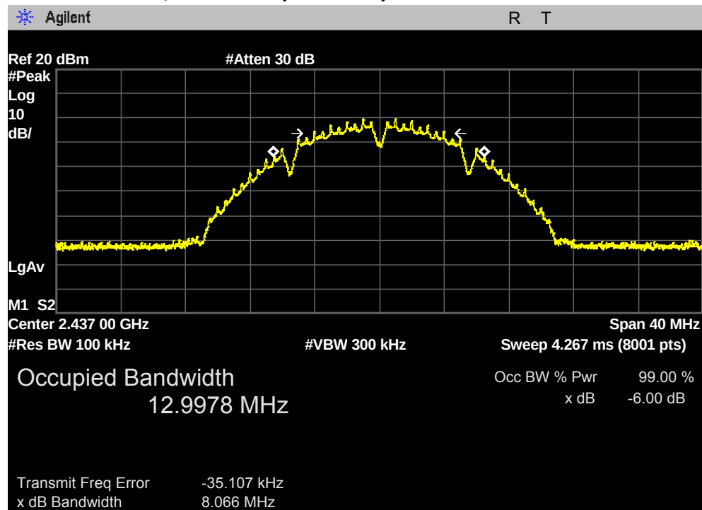
6 dB Bandwidth, 6 Channel (2437 MHz)
