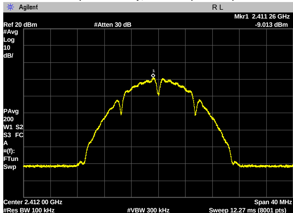
Maximum Power Spectral Density, 1 Channel (2412 MHz)
