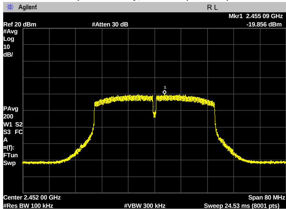
Maximum Power Spectral Density, 9 Channel (2452 MHz)
