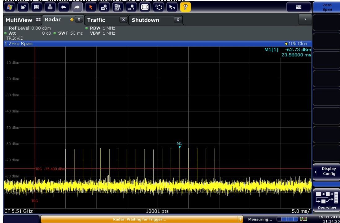
Radar test signal 0 threshold level at 5510 MHz
