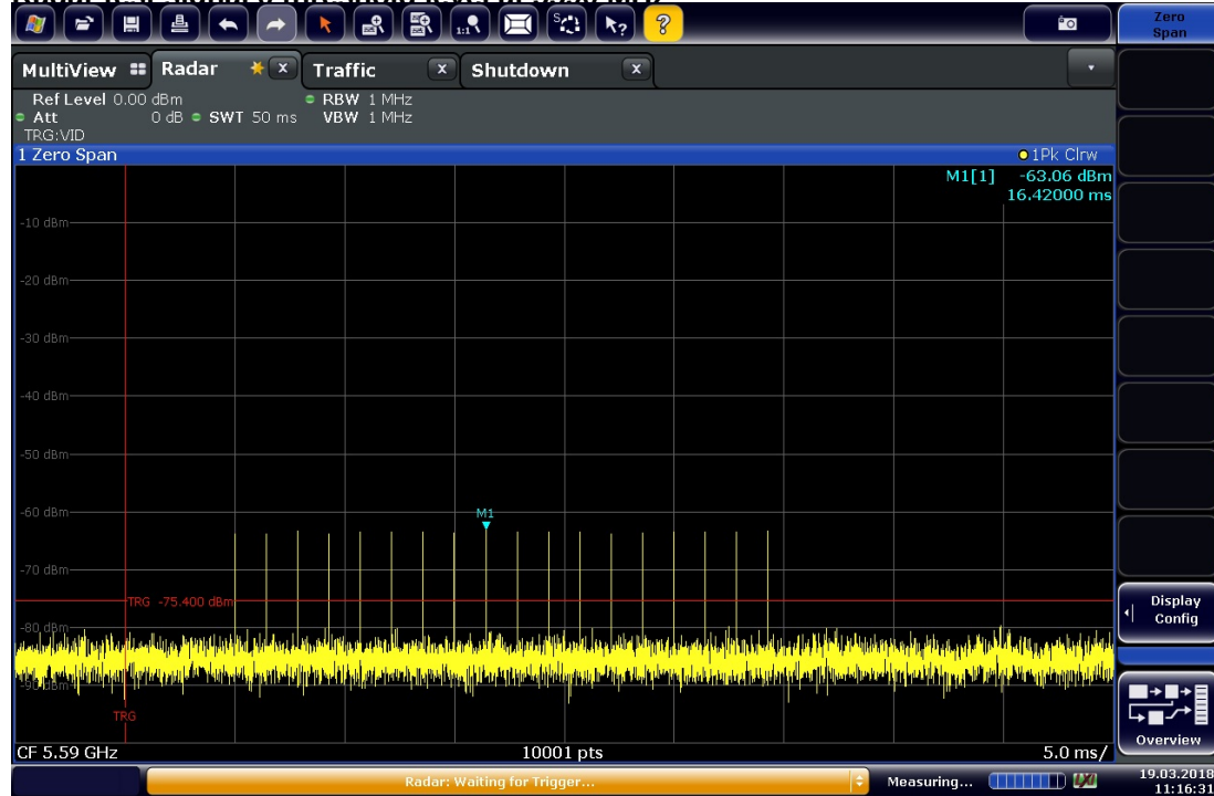
Radar test signal 0 threshold level at 5590 MHz
