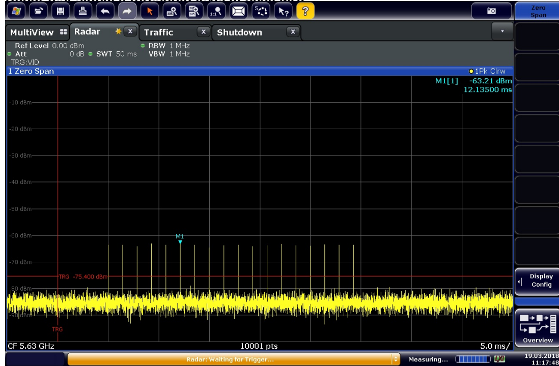
Radar test signal 0 threshold level at 5630 MHz
