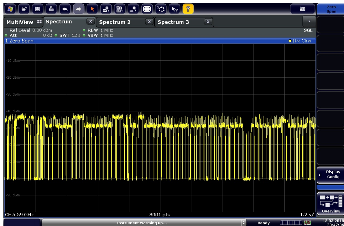
Data Traffic Plot at 5590 MHz
