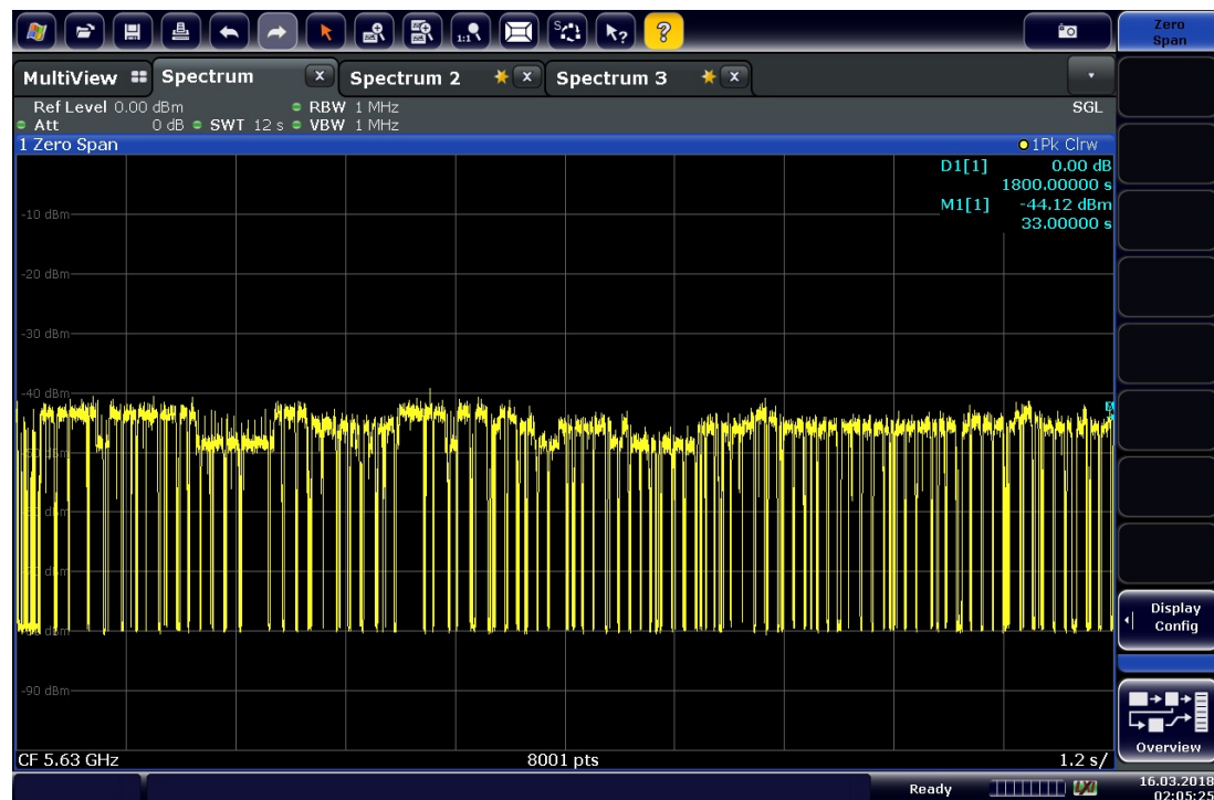
Data Traffic Plot at 5630 MHz
