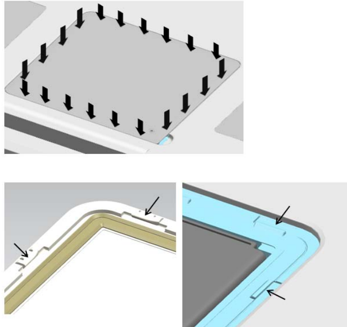
FIGURE 16 BATTERY COVER INSTALLATION
