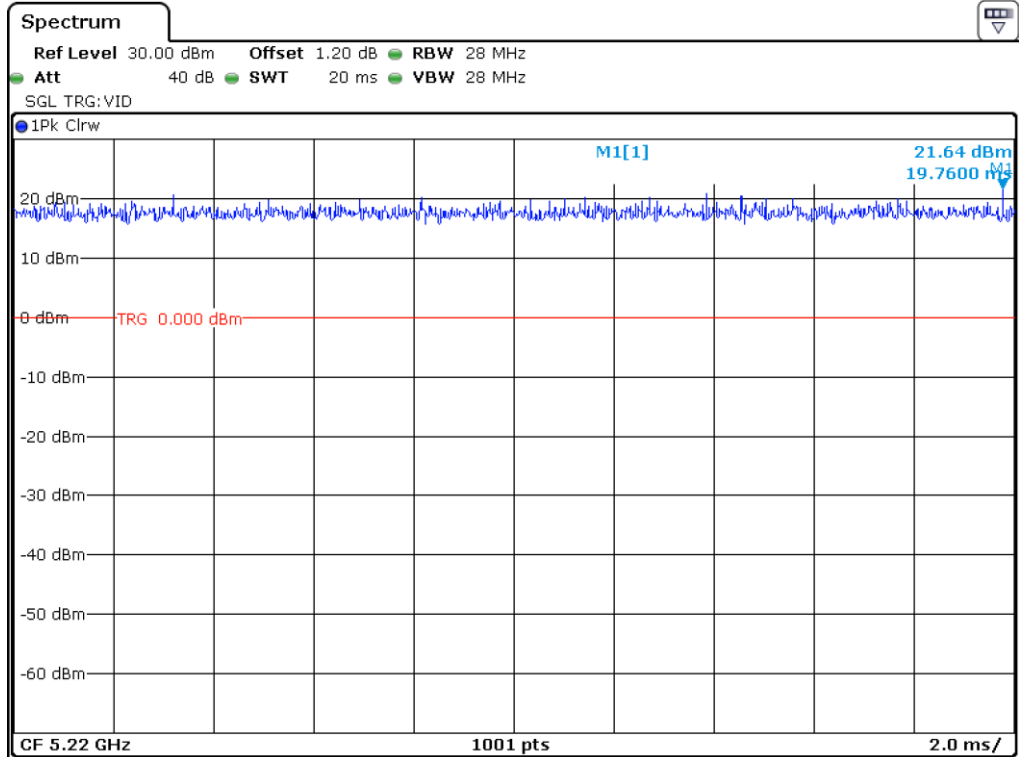
UNII 1_802.11 a_Antenna 1
