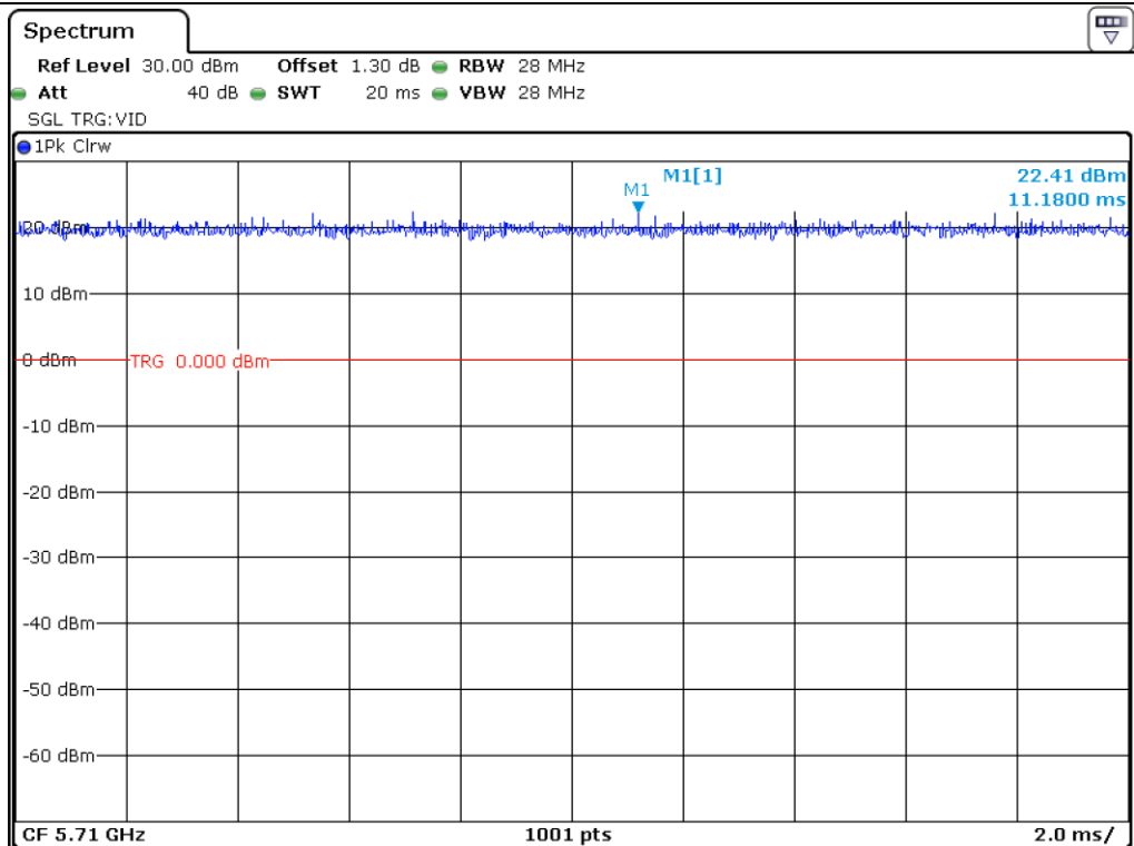
Staddle_802.11 HT40_Antenna 1
