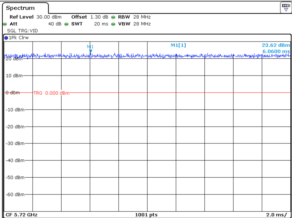
Staddle_802.11 a_Antenna 1
