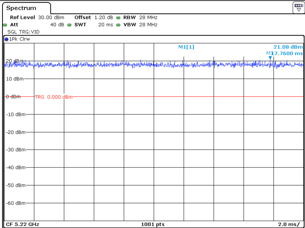
UNII 1_802.11 a_Antenna 1
