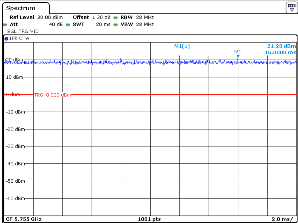
UNII 3_802.11 HT40_Antenna 0
