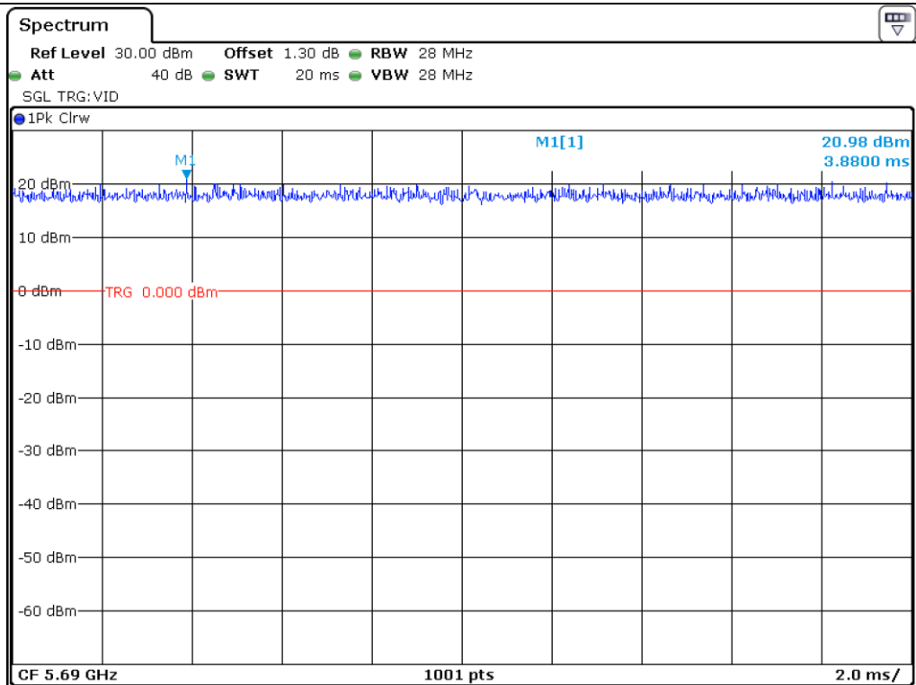
Staddle_802.11 HT40_Antenna 1
