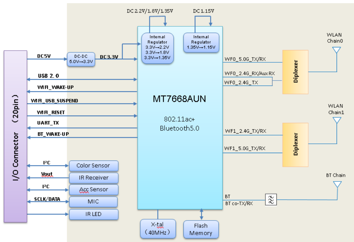
Figure 1-1 WCA732M block diagram and System Interface
