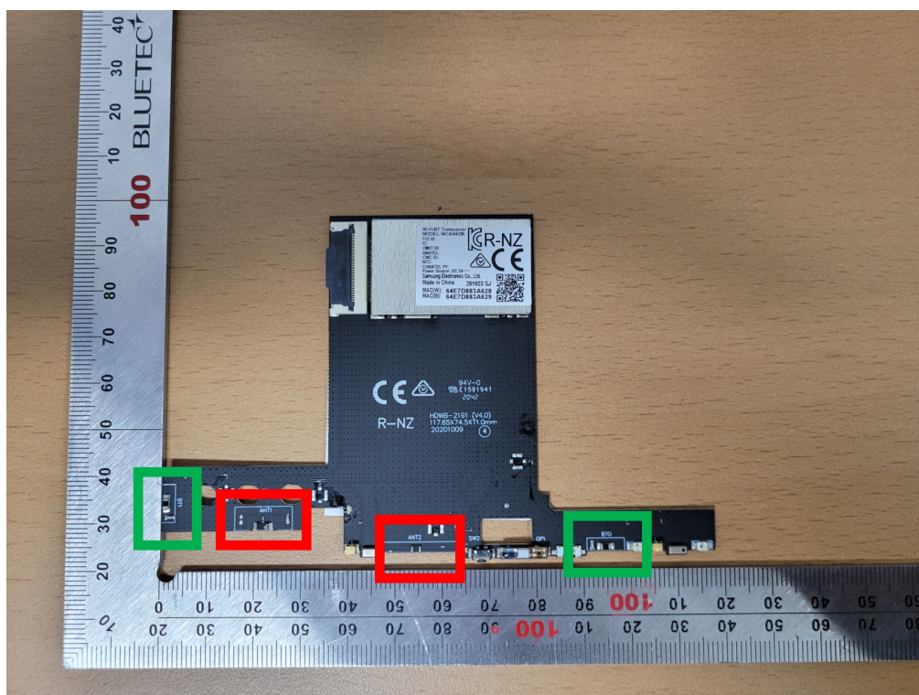
WLAN, BT Antenna
