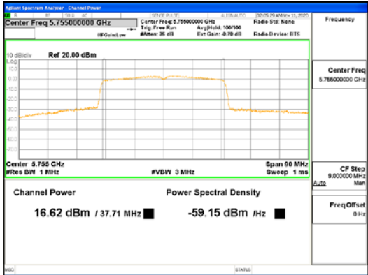
ANT1_802.11ax_HE40_UNI 3
