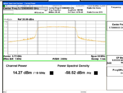
ANT1_802.11ax_HE20_UNII 2C
