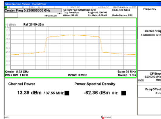
ANT2_802.11ax_HE40_UNII 1
