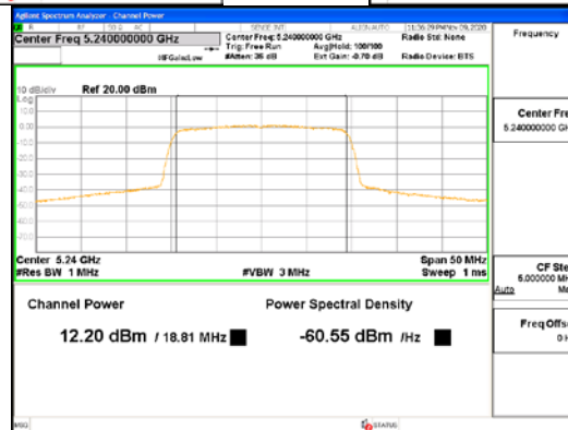
ANT2_802.11ax_HE20_UNII 1
