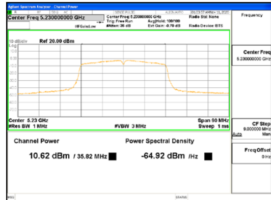
ANT1_802.11ac_VHT40_UNI1 1
