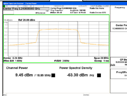
ANT1_802.11ax_HE20_UNII 1
