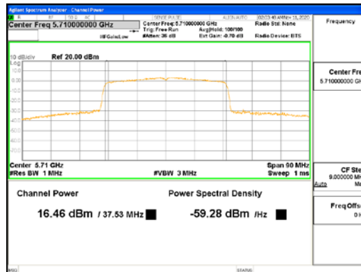
ANT1_802.11ax_HE40_UNII 2C
