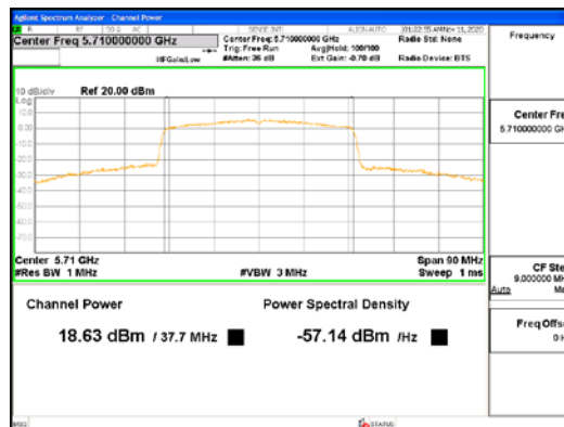
ANT2_802.11ax_HE40_UNII 2C
