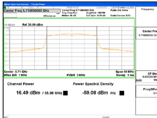
ANT1_802.11n_HT40_UNII 2C
