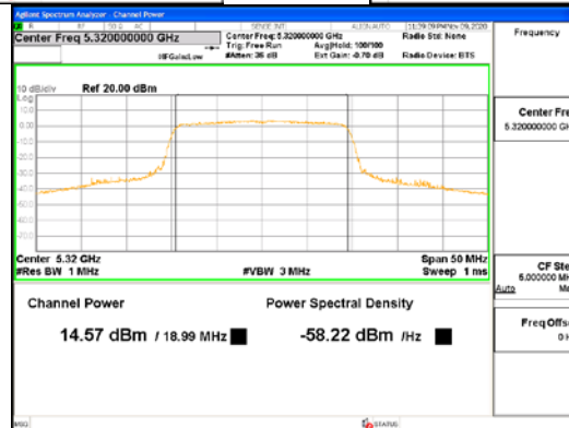
ANT2_802.11ax_HE20_UNII 2A
