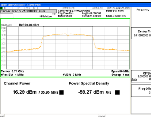
ANT1_802.11ac_VHT40_UNI1 2C
