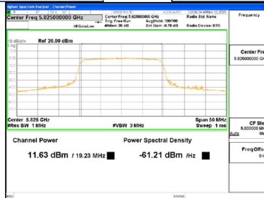
ANT1_802.11ax_HE20_UNII 3
