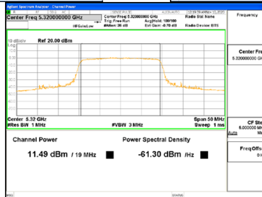
ANT1_802.11ax_HE20_UNII 2A
