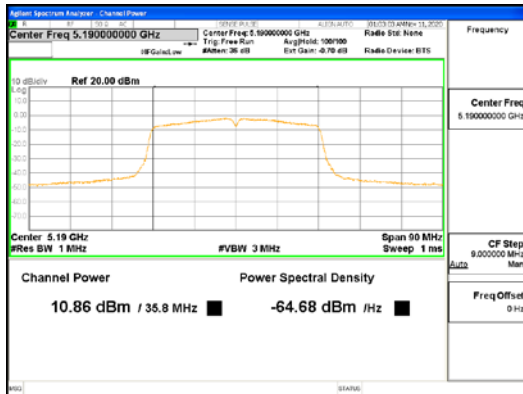
ANT1_802.11ac_VHT40_UNI1 1
