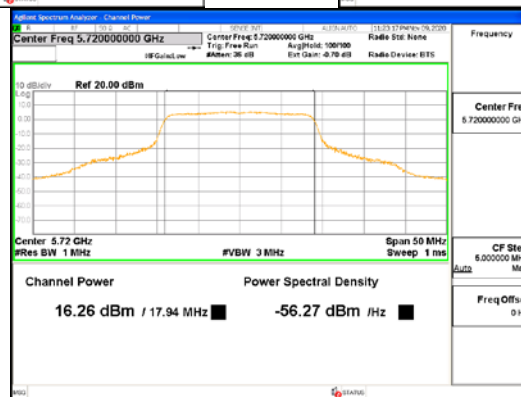
ANT2_802.11ac_VHT20_UNII 2C
