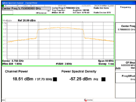
ANT2_802.11ax_HE40_UNI 3
