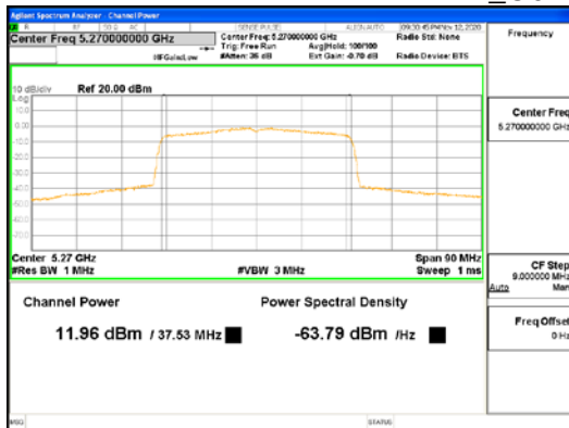
ANT1_802.11ax_HE40_UNII 2A
