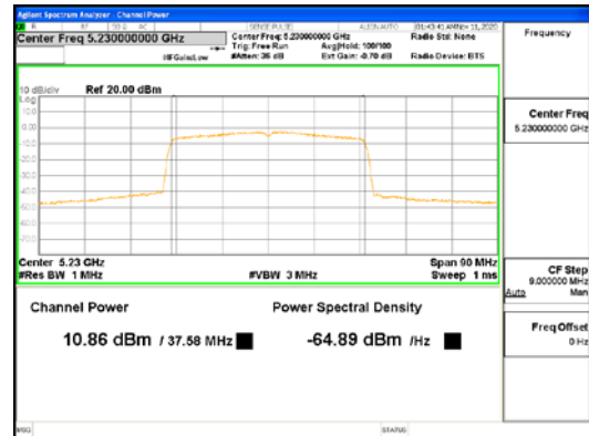
ANT1_802.11ax_HE40_UNII 1
