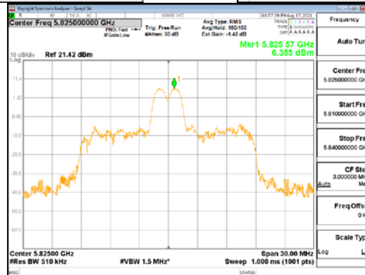
ANT2_802.11ax_HE20_26T_Mid_UNII 3
