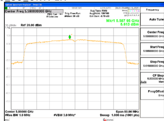
ANT2_802.11ax_HE40_SU_UNII 2C
