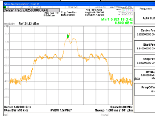
ANT1_802.11ax_HE20_26T_Mid_UNI1 3
