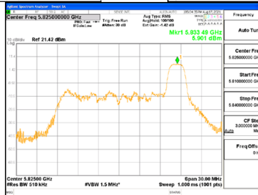
ANT1_802.11ax_HE20_26T_High_UNII 3
