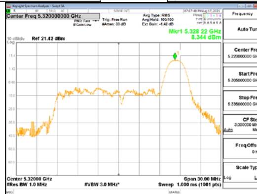
ANT2_802.11ax_HE20_26T_High_UNI1 2A
