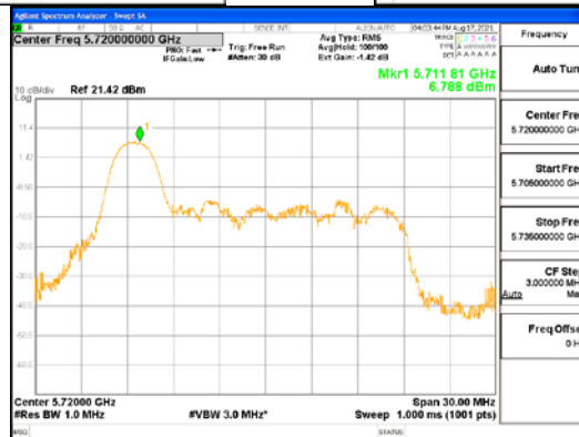
ANT1_802.11ax_HE20_26T_Low_UNII 2C
