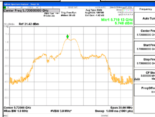
ANT1_802.11ax_HE20_26T_Mid_UNI1 2C
