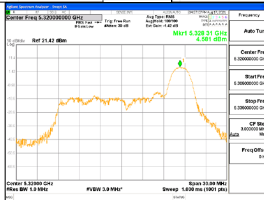
ANT1_802.11ax_HE20_26T_High_UNII 2A
