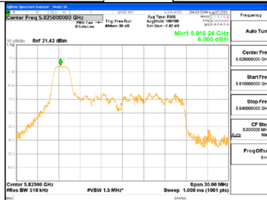
ANT1_802.11ax_HE20_26T_Low_UNII 3
