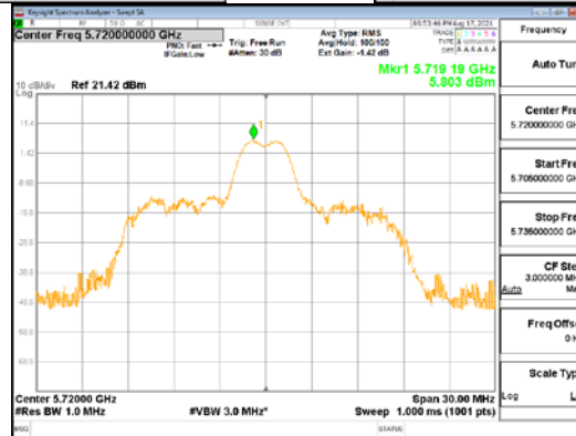
ANT2_802.11ax_HE20_26T_Mid_UNII 2C
