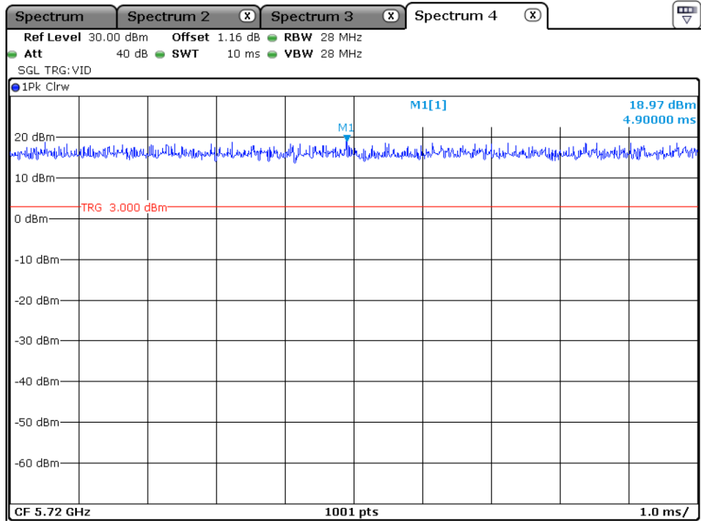
Staddle_802.11 a_Antenna 1
