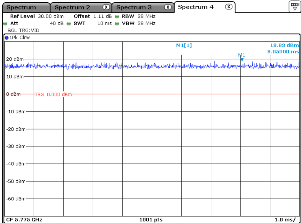
UNII 3_802.11 HT40_Antenna 1
