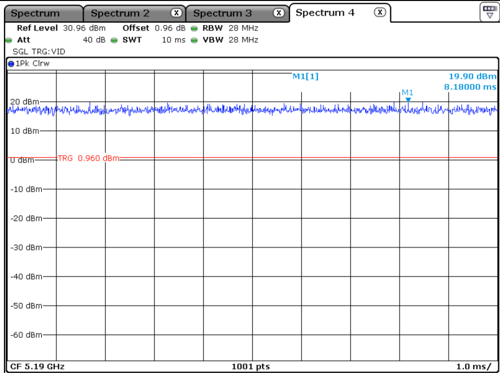
UNII 1_802.11 HT40_Antenna 0
