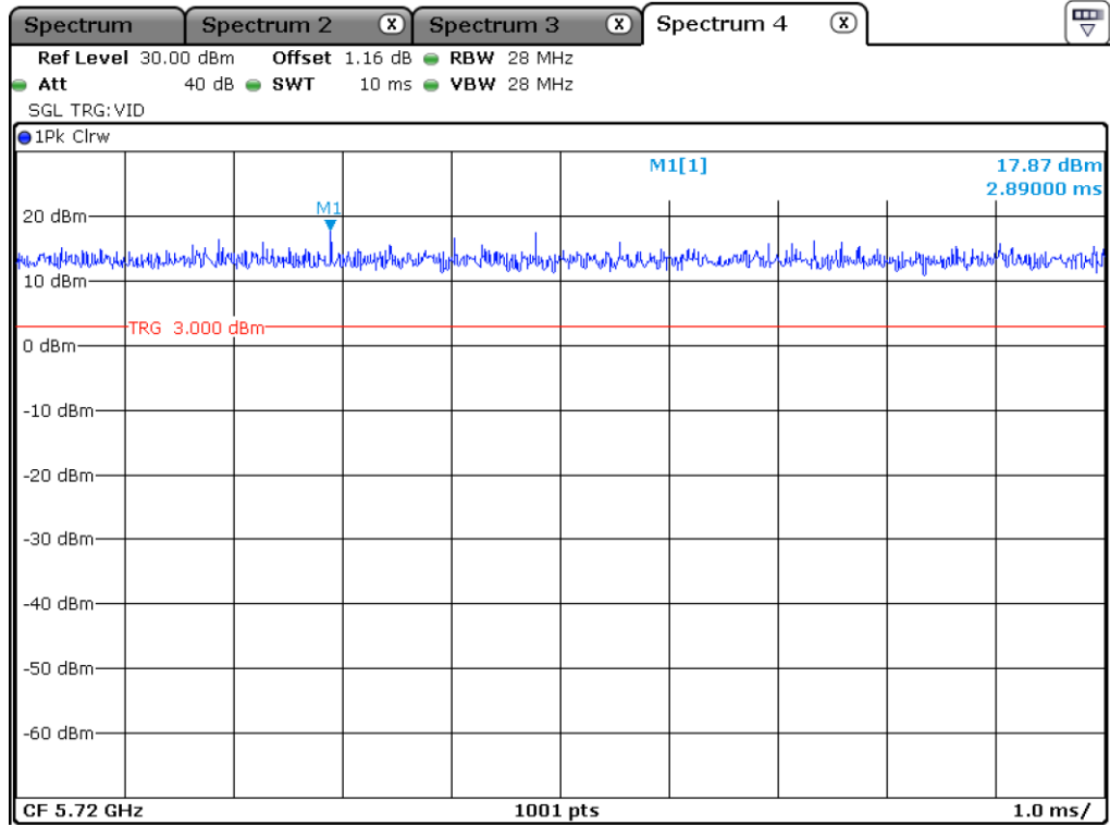
Staddle_802.11 a_Antenna 0
