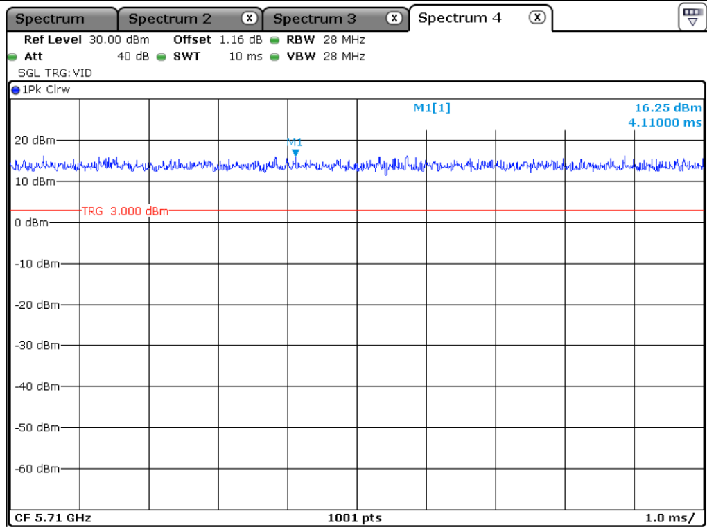
Staddle_802.11 HT40_Antenna 0
