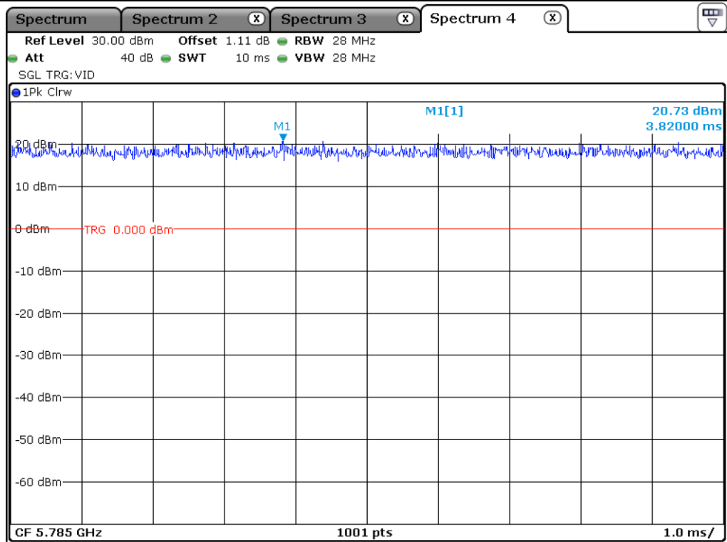
UNII 3_802.11 a_Antenna 1
