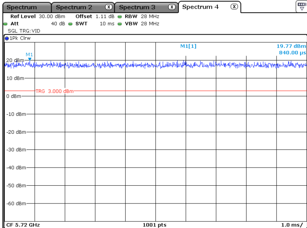
Staddle_802.11 a_Antenna 1
