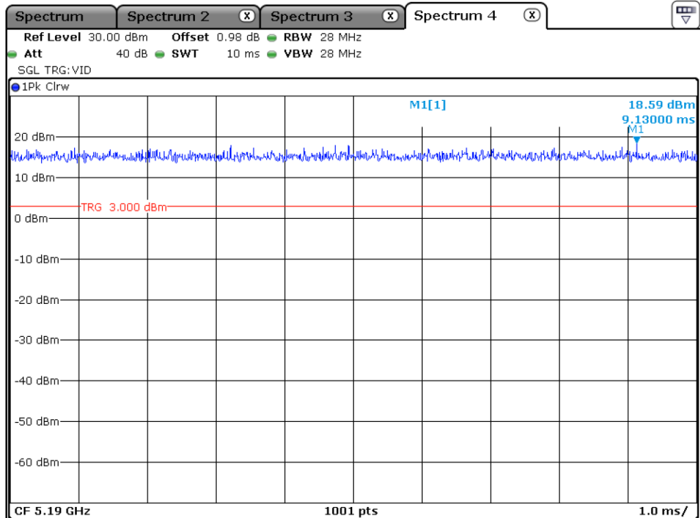
UNII 1_802.11 HT40_Antenna 1
