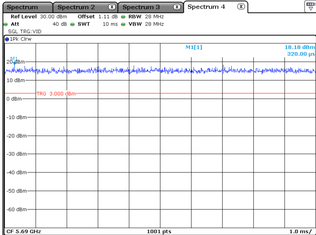
Staddle_802.11 HT40_Antenna 1
