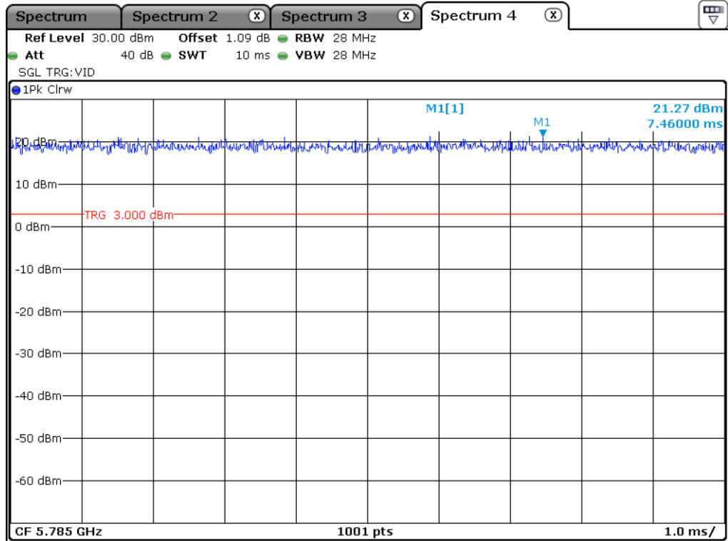
UNII 3_802.11 a_Antenna 0
