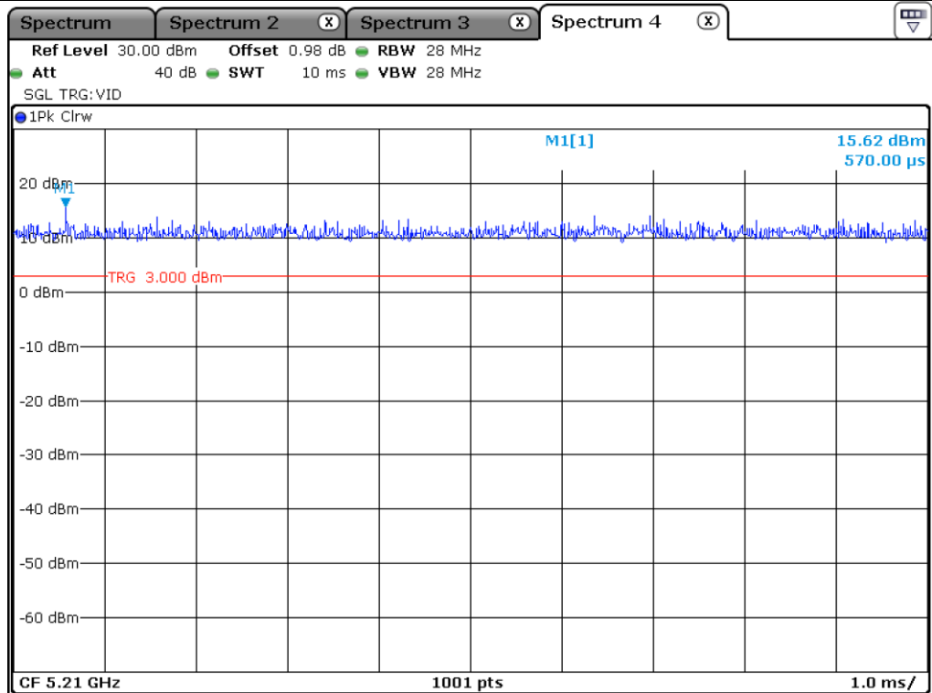
UNII 1_802.11 HT40_Antenna 1
